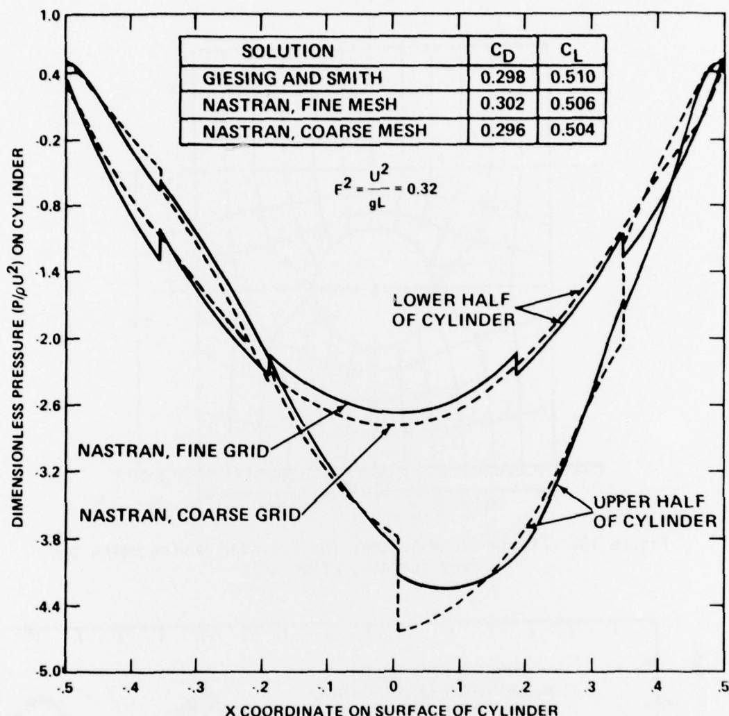
Figure 17. Pressure Distribution on the Cylinder
