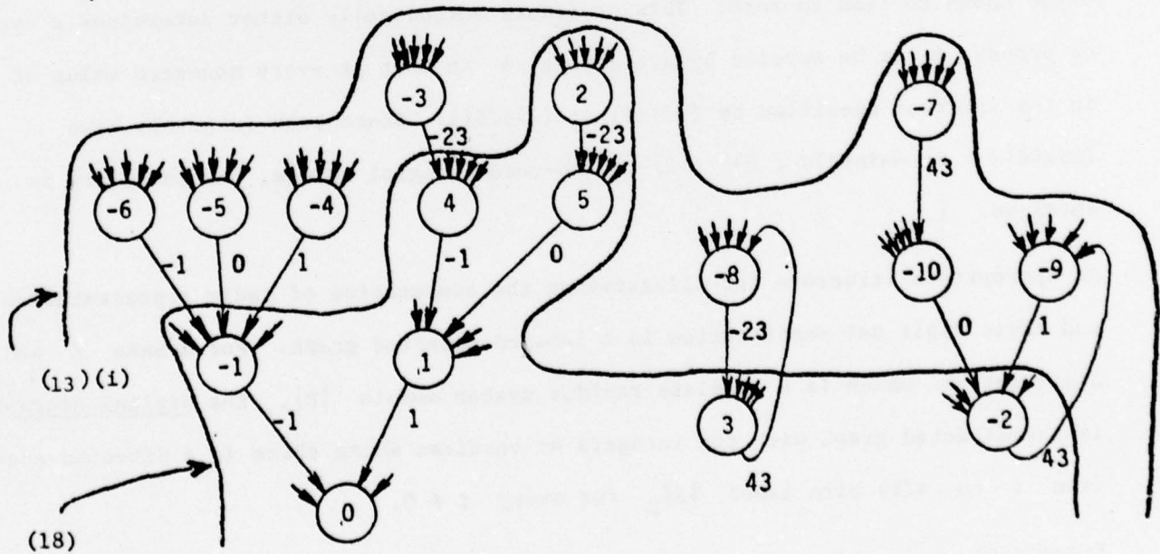
b) \beta = 5, D = \{0, 1, -23, 43, -1\}
