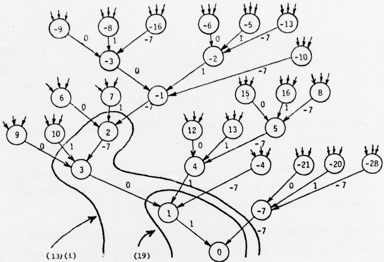
a) \beta = 3, D = \{0, 1, -7\}
