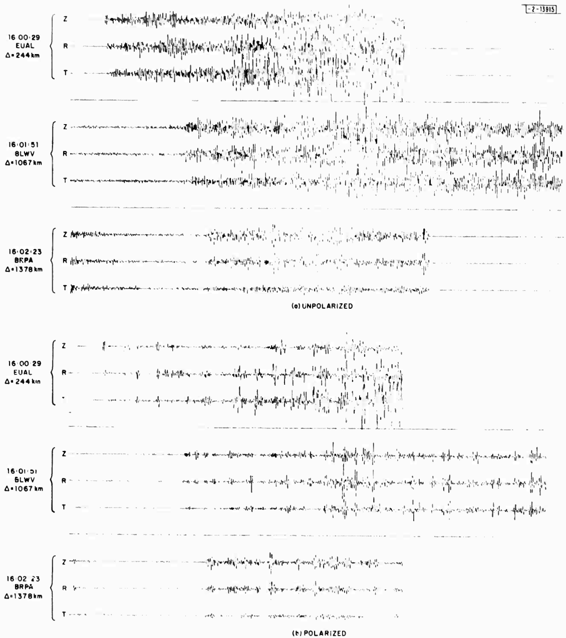
Fig. I-23. (a) Rotated 3-component data from SALMON recorded at LRSM stations EU-AL, BL-WV, and BR-PA. (b) Polarized data as described in text with cutoff ellipticity \epsilon_0 = 0.25 and filter order n = 3 .
