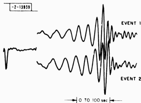
Fig. II-10. Rayleigh waves (Z component) at MAIO for Events 1 and 2 in Table II-3. Least-squares filter to shape Event 1 to 2 is to left.
