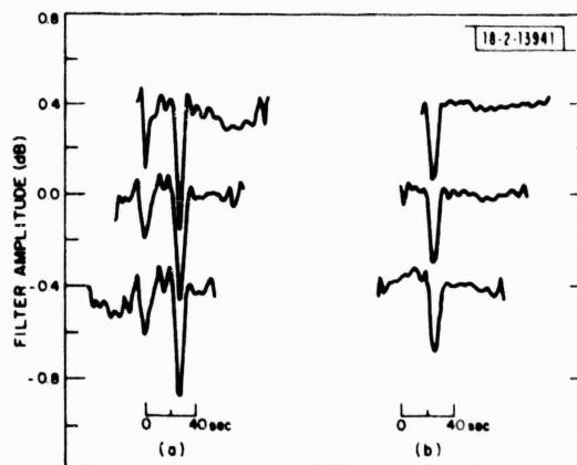
Fig. II-12. Filters at different lags: (a) to shape Event 1 to sum of Events 3 and 4, and (b) to shape Event 1 to 2.
