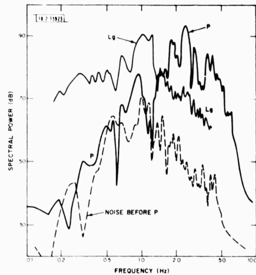
Fig. 1-31. Spectra of 20-sec windows of P, Lg, and noise before P of event 5 - PNE of 9 July 1972. Note higher frequency character of P wave and lower level of Lg spectrum compared with Fig. 1-30. m_b = 4.8 , \Delta = 17.7^\circ .
