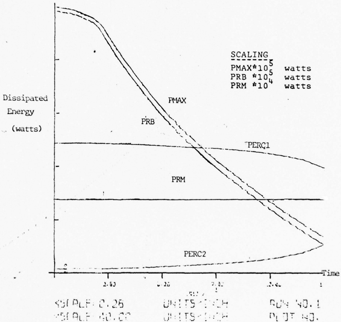
Fig.15-Power dissipation diagram-Theoretical resistor
