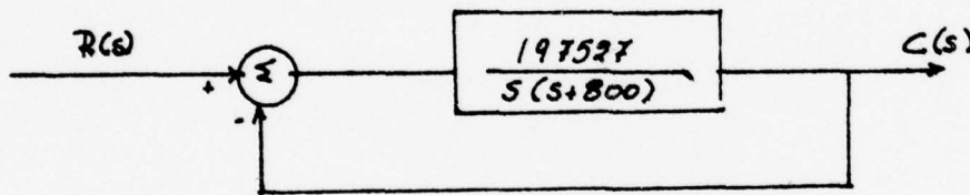
Figure 8. Closed loop positioning servo
