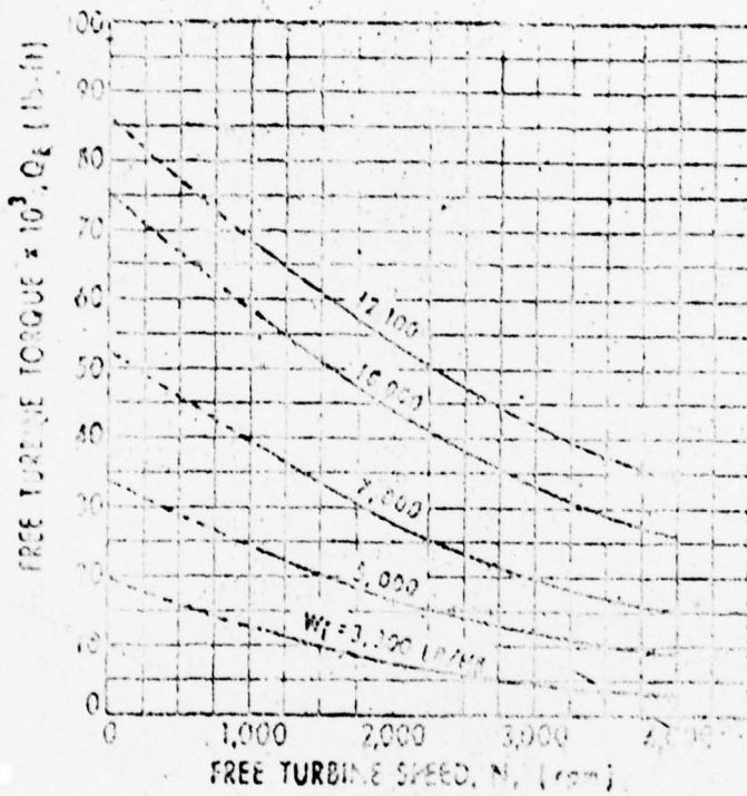
Fig. 38-Engine torque versus engine speed and fuel flow rate.
