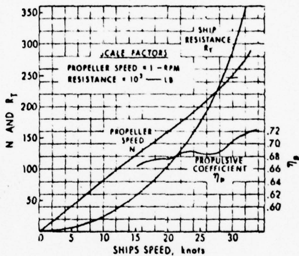
Fig 41-Plot of ship's resistance (R), propeller speed (N p ) and propulsive coefficient (η p ) versus ship's speed (V).
