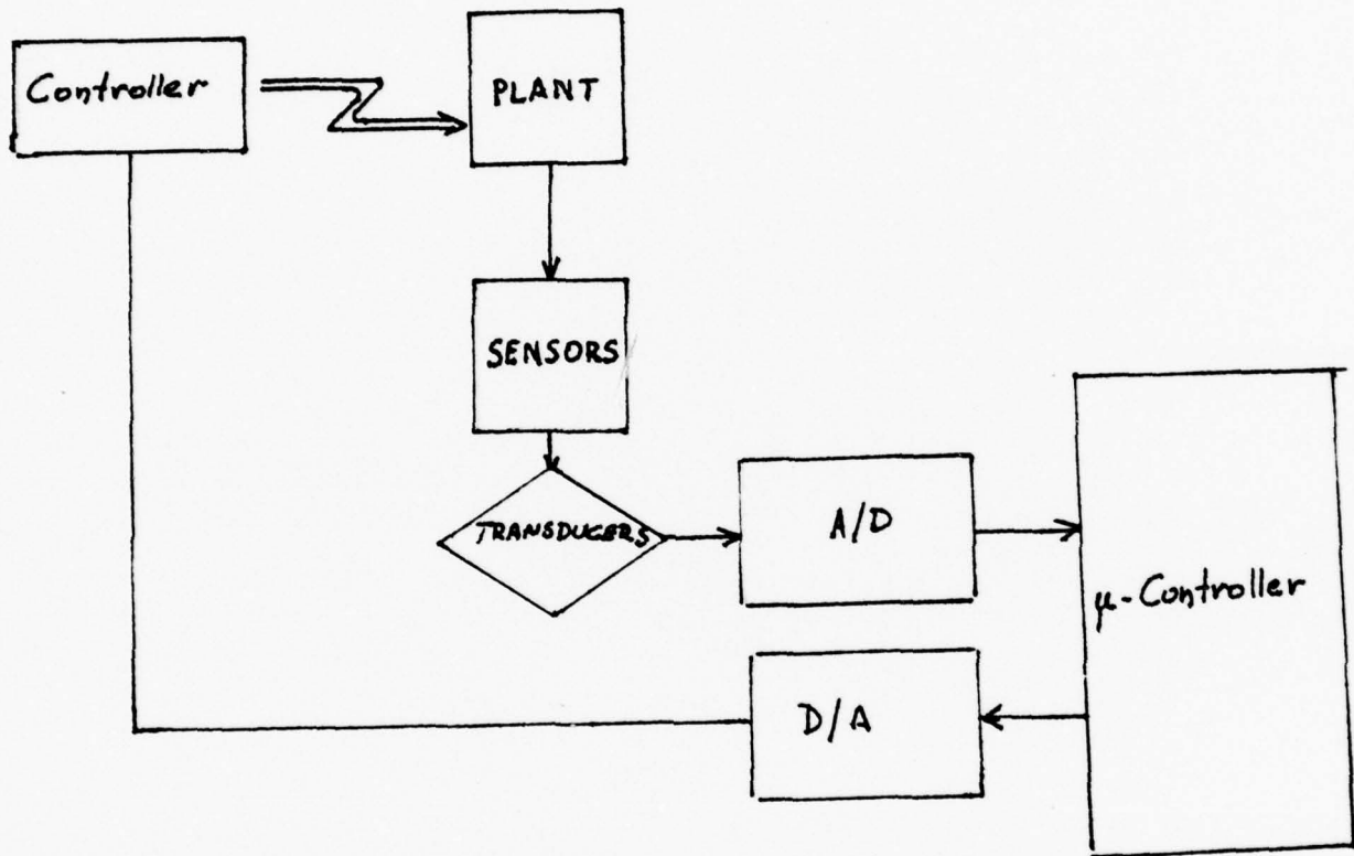
Figure 6. A real time \mu -controller system
