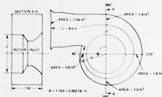
Fig. 6 - SES-100B Scale Model Fan Geometry
