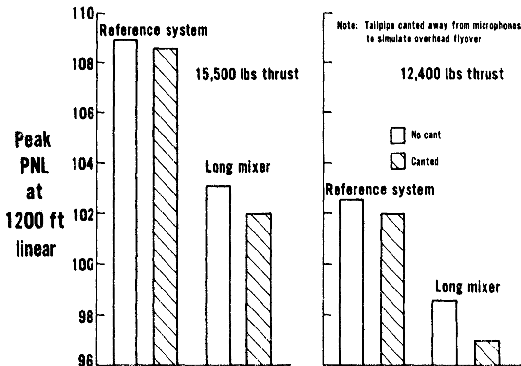
Figure 10 Effect of 5 Degree Tailpipe on Peak Perceived Noise Levels of Reference Exhaust System and the Canback Scaloped Long Flowpath Mixer (without Engine Secondary Flow Simulation)
