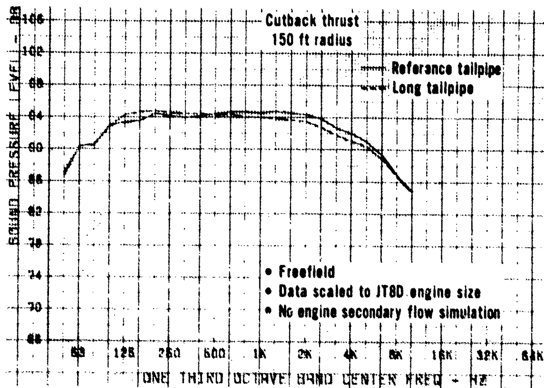
Figure 8.82.a Effect of Long Tailpipe on SPL Spectra at 90 Degrees of Cutback Scalloped Long Aliver
