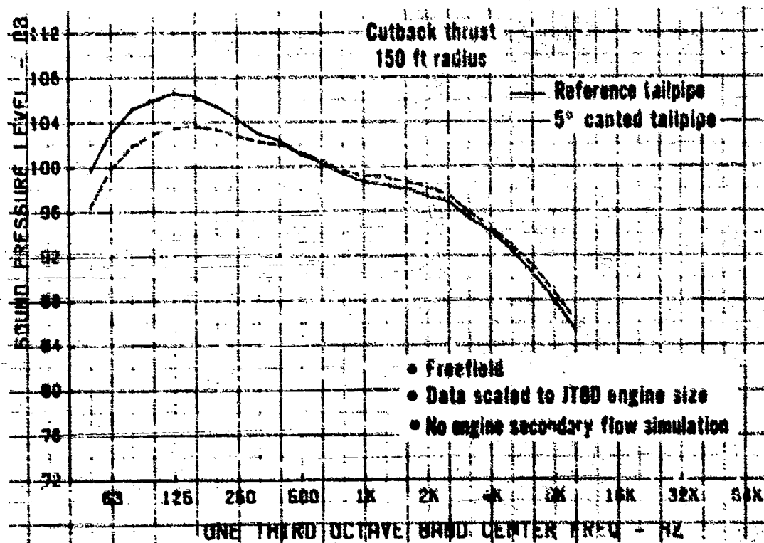
Figure 5-75(b) SPL Spectra at 140 Degrees
