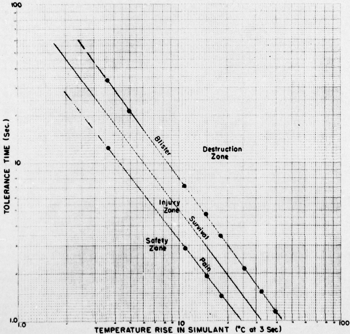
Fig. 2. Human skin tolerance time indicated by the temperature rise measured in a skin simulant at 3 seconds' exposure to a rectangular heat pulse.
