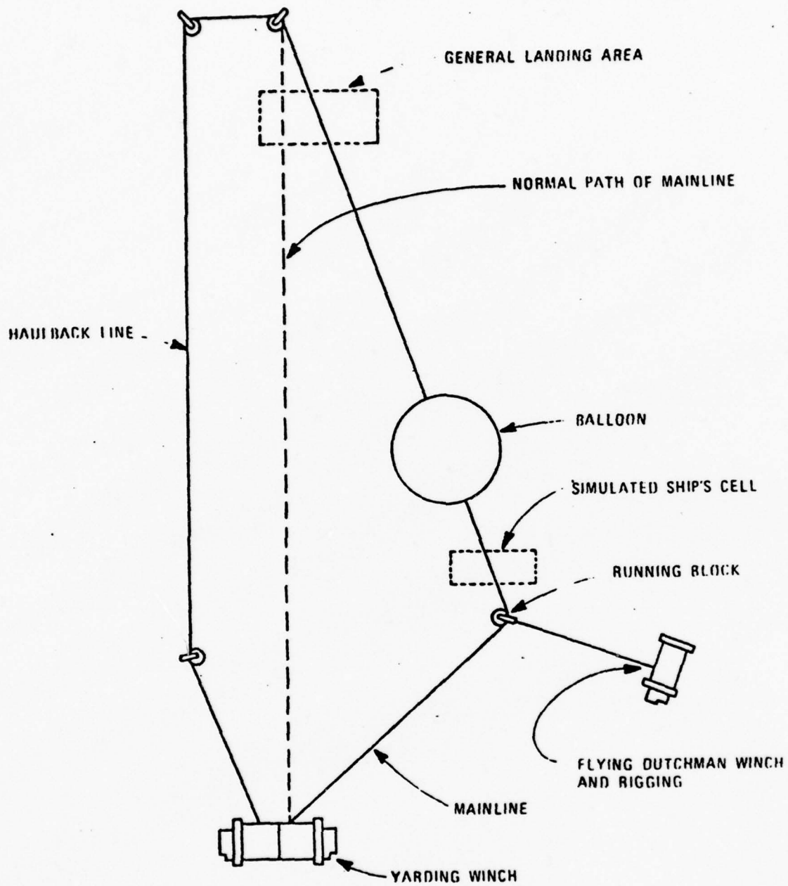
Figure 28. Test Series II (Plan View). Source: Air Force Range Measurements Laboratory, Balloon Feasibility Study .
