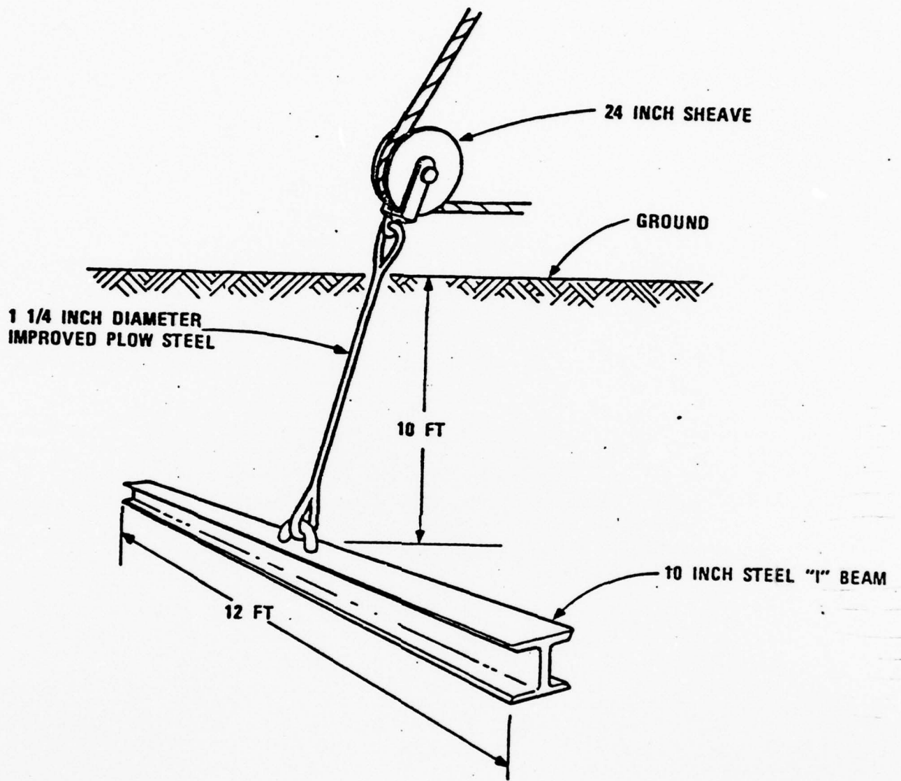
Figure 22. Anchor System.
