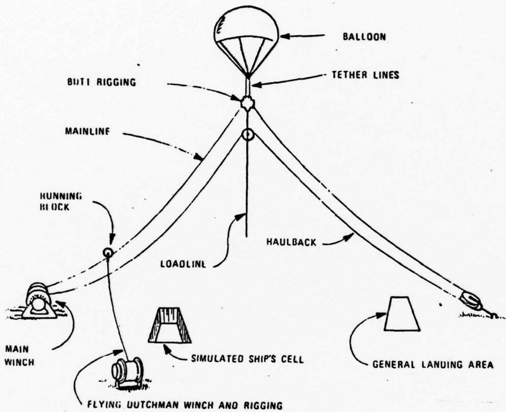
Figure 30. Inverted Skyline. Source: Air Force Range Measurements Laboratory, Balloon Feasibility Study.
