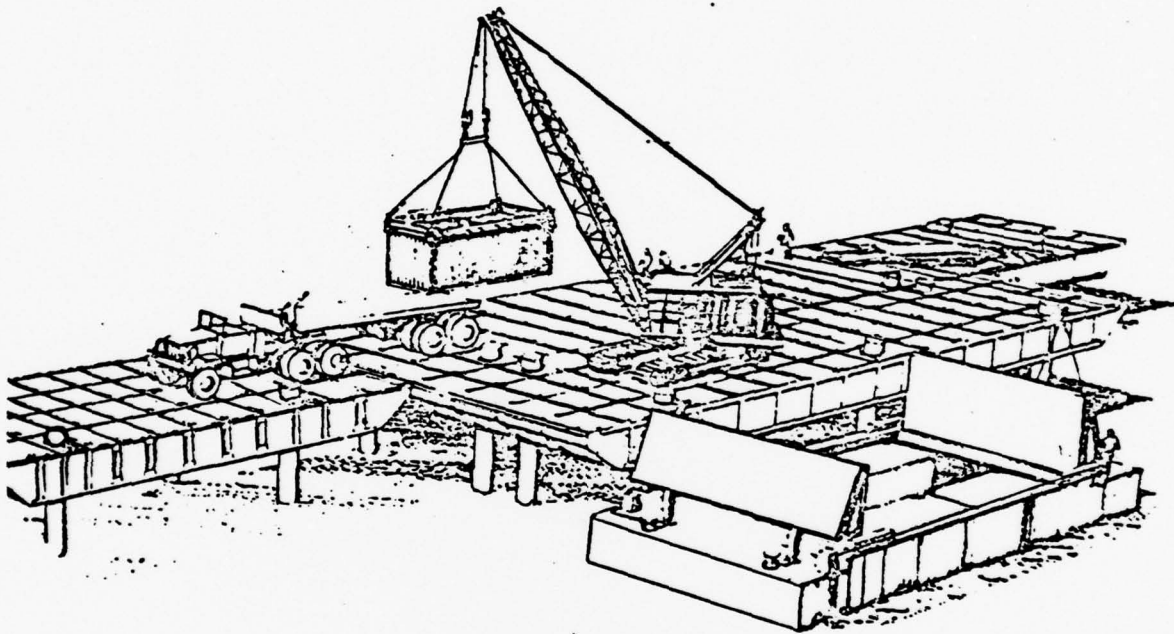
Figure 3. The Elevated Causeway. Source: Naval Facilities Engineering Command, Naval Beach Group Capabilities in Support of SMLS or Barge/Container Missions.
