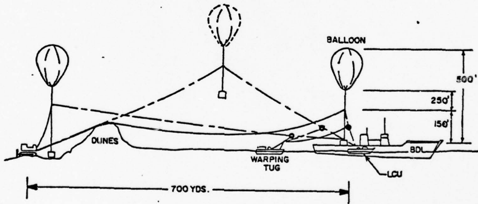
ELEVATION VIEW
