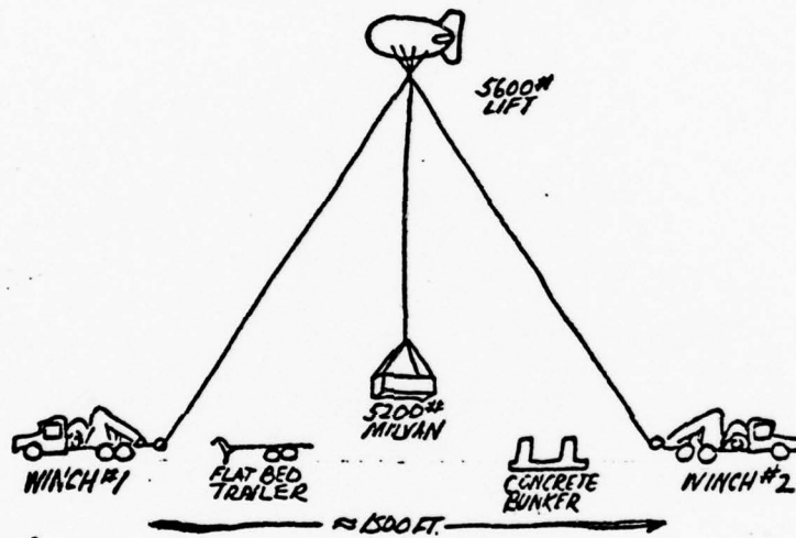
Figure 32. Stapleton Logistics Experiment Test Configuration. Source: Air Force Range Measurements Laboratory, Stapleton Logistics Experiment.
