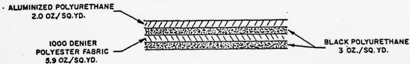
Figure 24. Material Construction Schematic.
