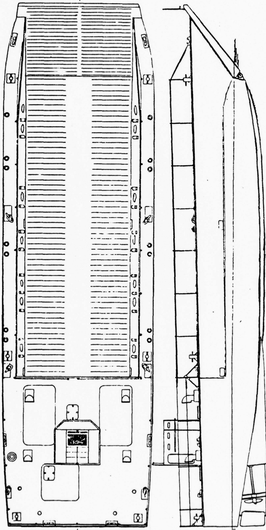
Figure 5. The LCM-8. Source: David W. Taylor Naval Research and Development Center, Follow-On and Resupply Shipping Assets for a Representative Marine Corps Situation.
