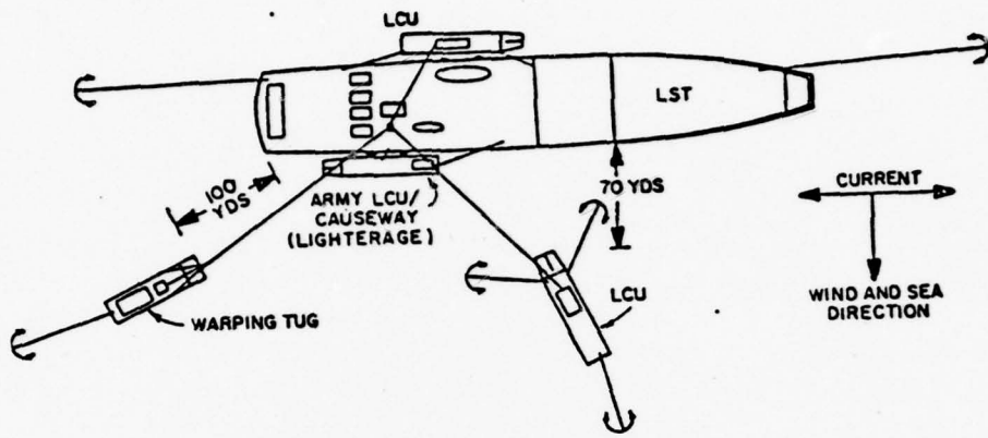
PLAN VIEW (Showing Anchoring Arrangement)
