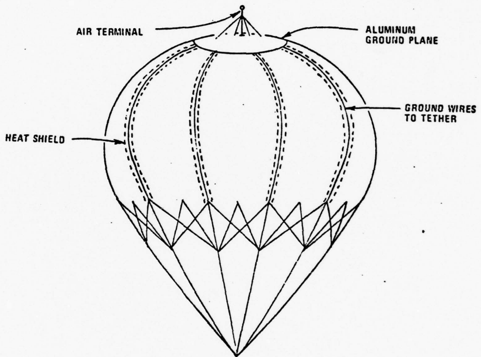
Figure 37. Balloon Lightning Protection System. Source: Air Force Range Measurements Laboratory, Balloon Feasibility Study .
