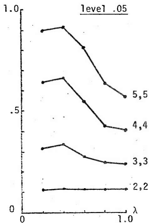
Figure 5.2. Estimated power of T_\lambda as a function of \lambda under compound periodicity at two frequencies with equal amplitudes R_1 and R_2 , indicated next to curve.
