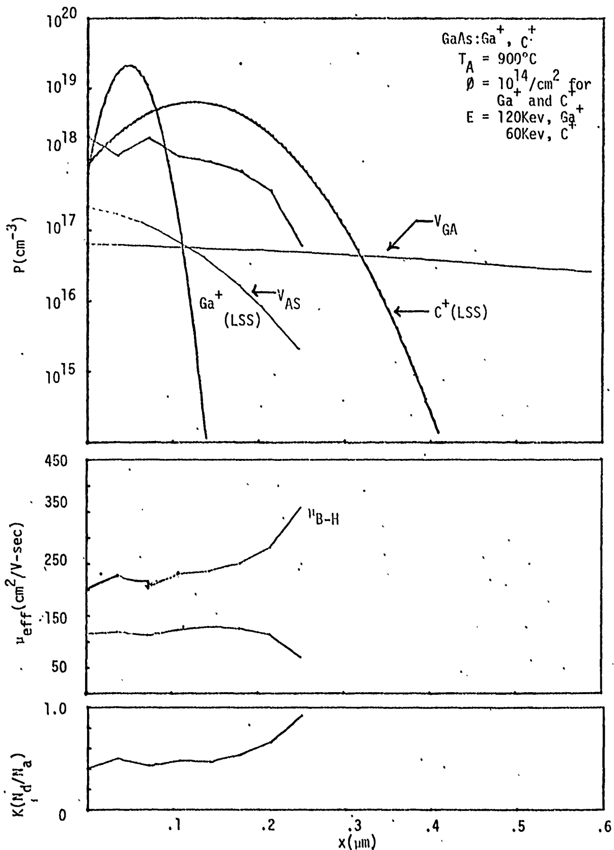
Fig. 15. Electrical profiles of carrier concentration ( P ), mobility ( \mu_{\text{eff}} ) and electrical compensation factor ( K ) with depth ( x )
