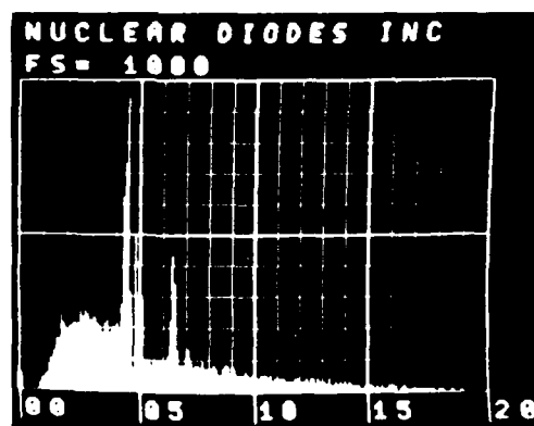
(b) FROM THE GRAIN BOUNDARY PHASE SHOWN IN FIGURE 6.
