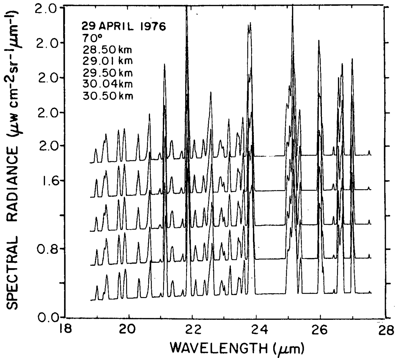
Figure 57. Linear spectral radiance in the 18.8-27 \mu\text{m} region at 28.50, 29.01, 29.50, 30.04 and 30.50 km and a zenith angle of 70°. Spectra are offset for clarity.
