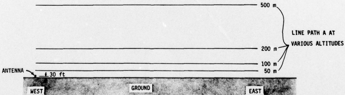
Figure 5 ELECTRIC FIELD ALONG LINE A DUE TO THE N-S WTF ANTENNA
