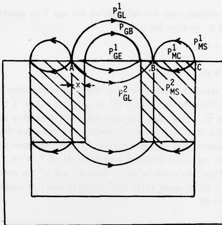
Fig. 3. Configuration C. This arrangement differs from configuration A chiefly in its shorter gap which gives rise to the additional permeance paths P^1_{GL} , P^2_{GL} , P_{GB} . The location of points A and B and length x are derived in the text.
