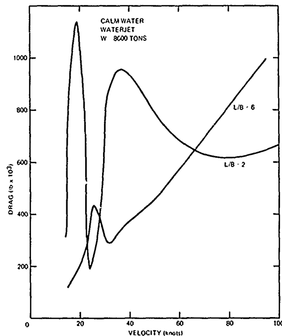
Fig. 26 - Total Drag versus Velocity Comparison for L/B 2.0 and 6.0
