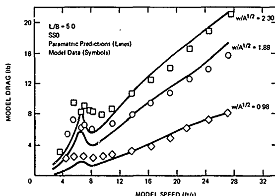
Fig. 15 - Weight Variation Predictions -- Parametrics versus Model Data
