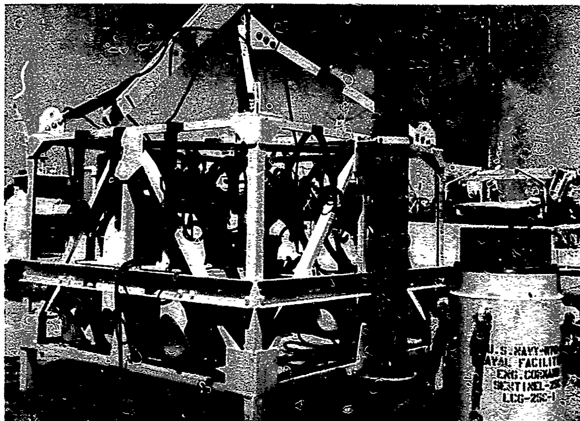
Figure 2-17. Sentinel-25C1 RTG Standing Beside Platform on Which it was Mounted for Mission.
