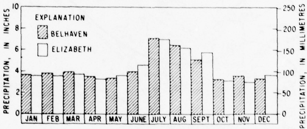
Figure 5.--Average monthly precipitation at Elizabeth City, N.C., and Belhaven, N.C., 1910-60.
