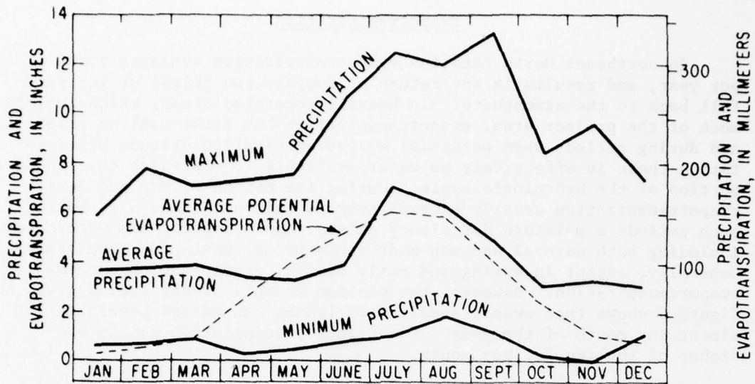
Figure 6.--Maximum, average, and minimum monthly precipitation and calculated average evapotranspiration at Elizabeth City, N.C., 1931-60.
