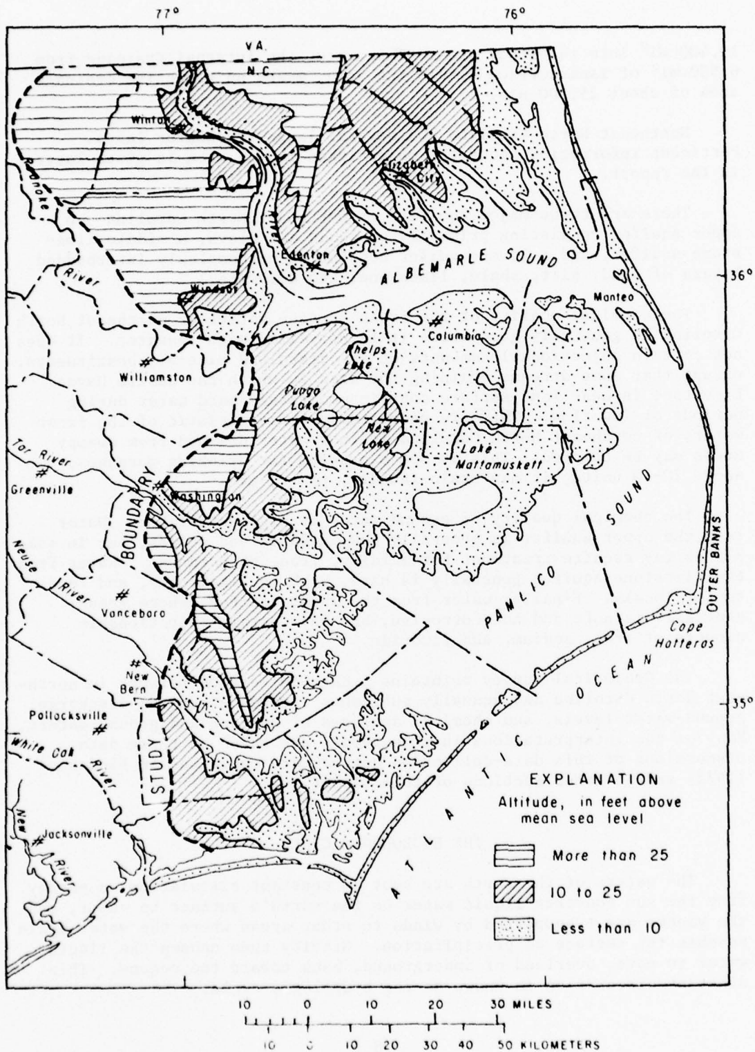
Figure 2.--Generalized land-surface altitude.
