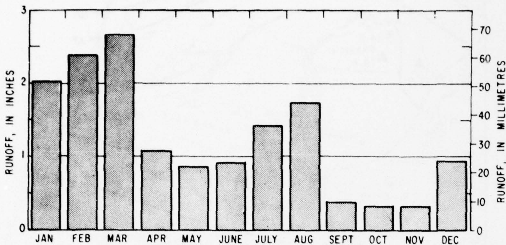
Figure 19.--Average monthly runoff for streams draining the study area.
