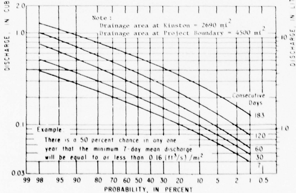
Figure 23.--Low-flow frequency curves of annual lowest mean discharge for indicated number of consecutive days, for Neuse River near Kinston, N. C.
