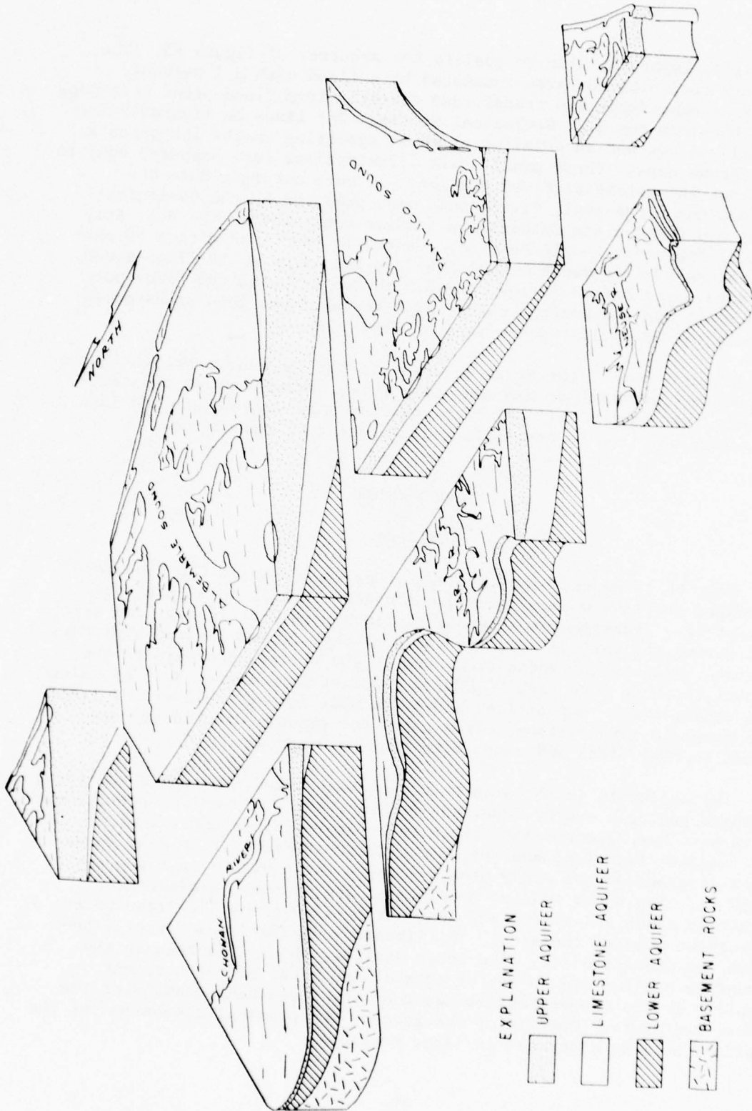
Figure 46.--Generalized block diagrams of northeast North Carolina showing the upper 1,000 feet of the underlying aquifers.
