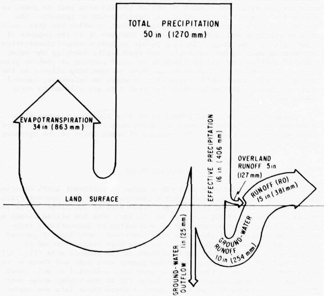
Figure 11.--The components of the hydrologic cycle in northeast North Carolina.
