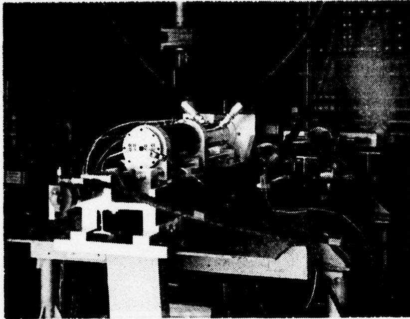
Figure 4. Photograph of Apparatus on Thrust Stand.
