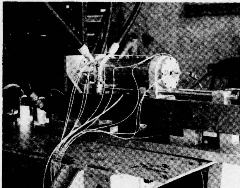
Figure 6. Photograph of Full Forward Position with Instrumentation.
