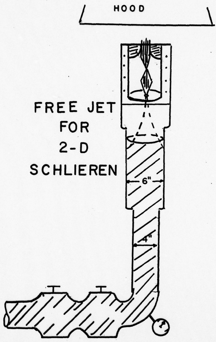
Figure 13. Schematic of Free Jet Equipment.
