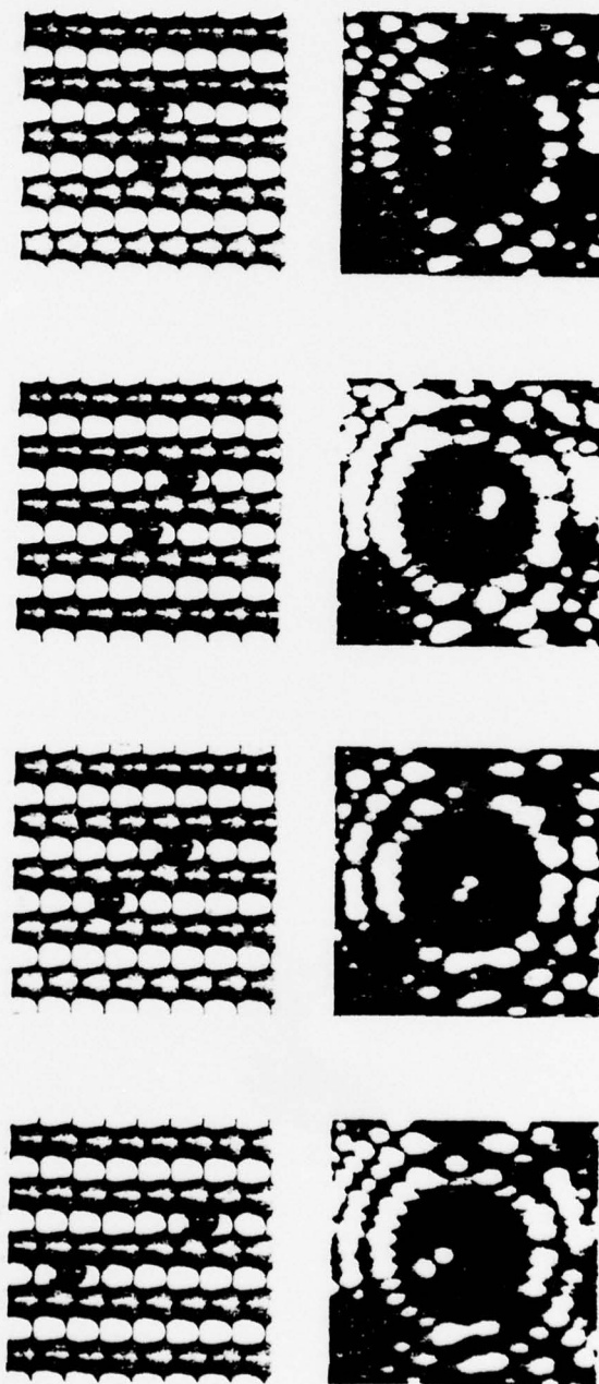
Fig. 2. Configurations of bound and dissociated rhenium dimers on W(211). Hard-sphere model on left, field ion image on right. Dimer configurations, from top to bottom: 0, 1, 2, and 4: the top two are bound, the bottom two free. Interatomic separation of atoms in dimer established by techniques in reference 4.
