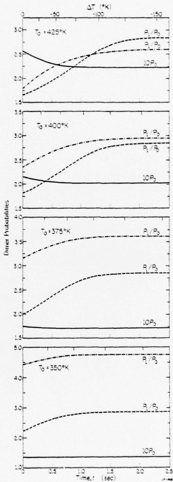
Fig. 8. Change in probabilities P_1/P_0 , P_1/P_D , and P_D during quench of model dimers equilibrated at T_0 . Temperature decay parameter \underline{b} = 5.75 \times 10^{-4} \text{ (deg sec)}^{-1} .
