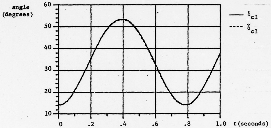
Figure 5.3 Plots of \delta_{c1} and \tilde{\delta}_{c1} .
