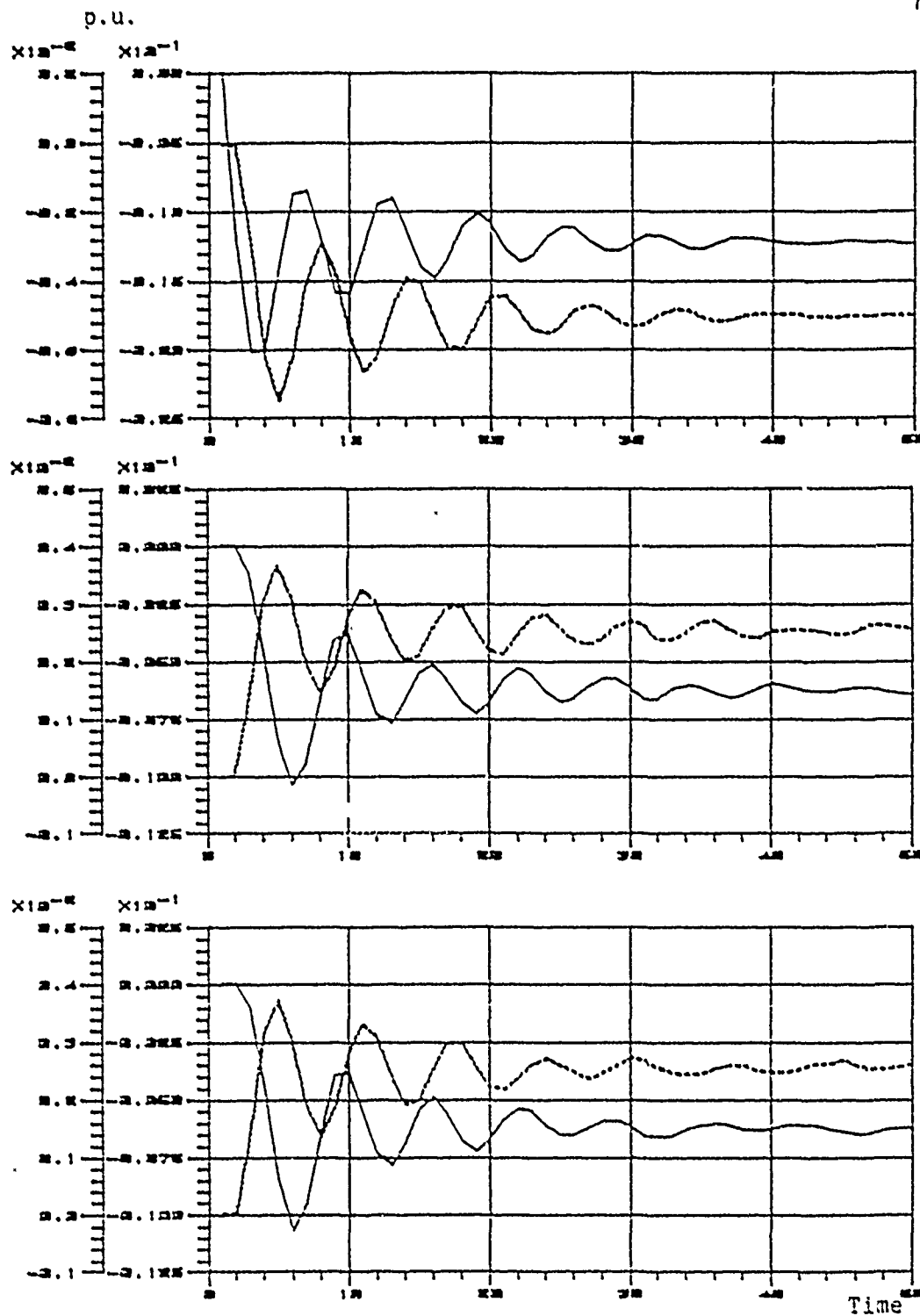
Fig. 5.1 Free system response of area 0,1,2
