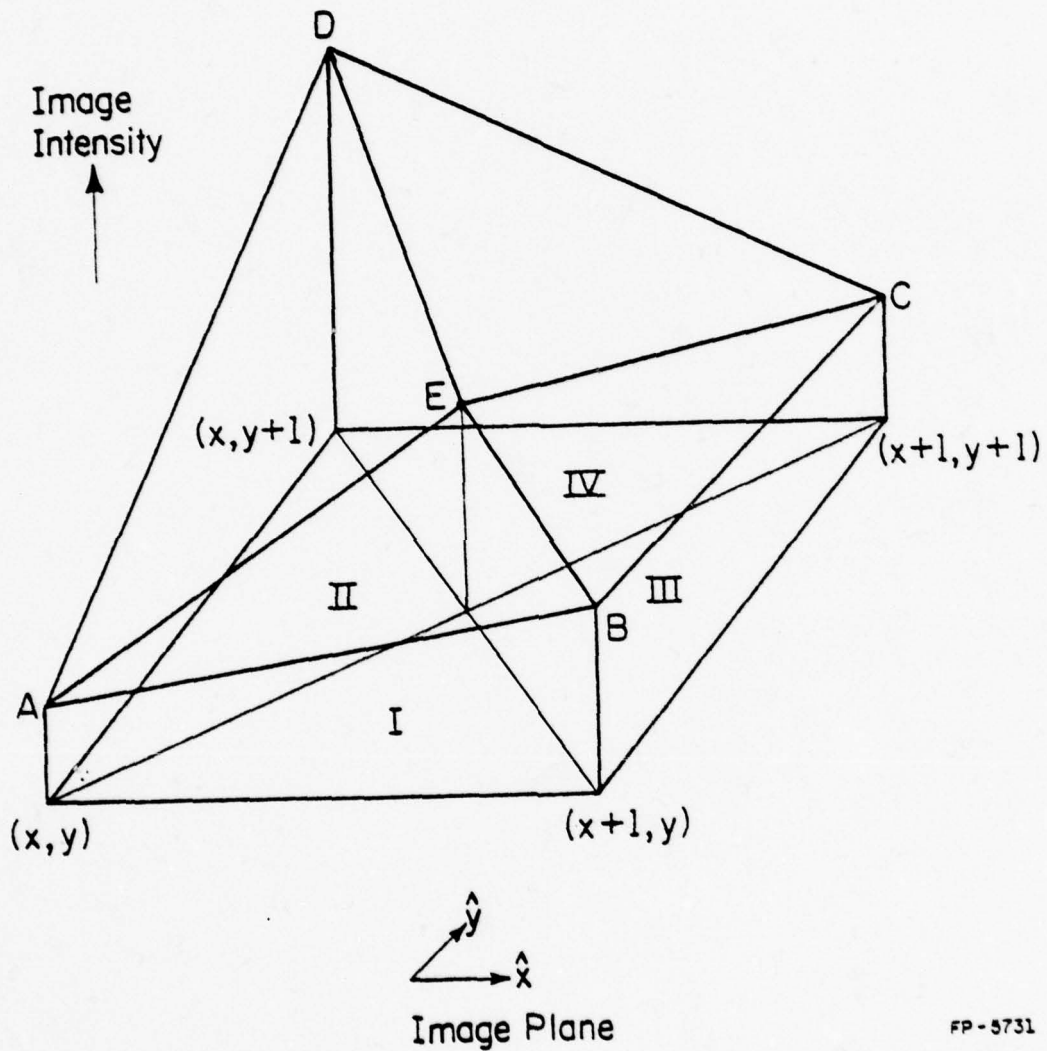
Figure 5.3-1 Illustration of planar interpolation of intensities between discrete pixel locations. If E is defined as the average of the intensities A, B, C, and D, then four planes are specified, ABE, BCE, CDE, and DAE. The interpolated intensity value for an arbitrary location within the square region becomes the value indicated by the planar segment directly above it. This results in a continuous intensity surface with piecewise constant gradients.
