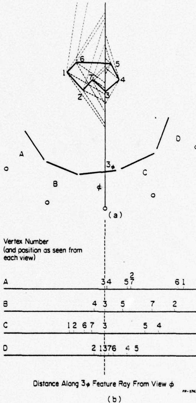
Figure 5.1-1 (a) Illustration of multiple view redundancy in two dimensions. A feature from vertex 3 in the object appears at location 3\phi in view \phi . Additional views A, B, C, and D are shown, and corresponding features of the object are projected from these projection centers onto the ray 3-3\phi . (b) The locations of projected features along line 3-3\phi of 'a' are shown. Notice that the projections of the true feature (number 3) all occur at the same ray coordinate, and others are misaligned.
