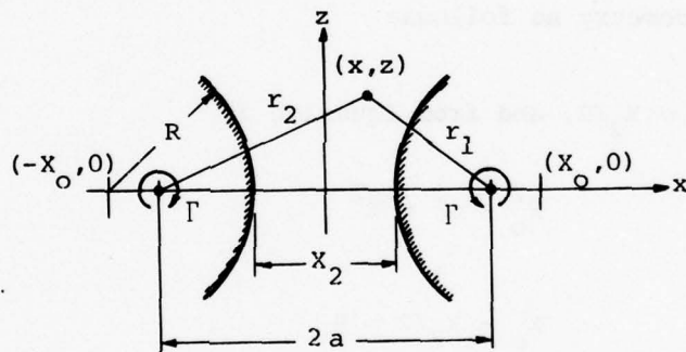
Figure 5. MID-SECTION OF AN AJDE
