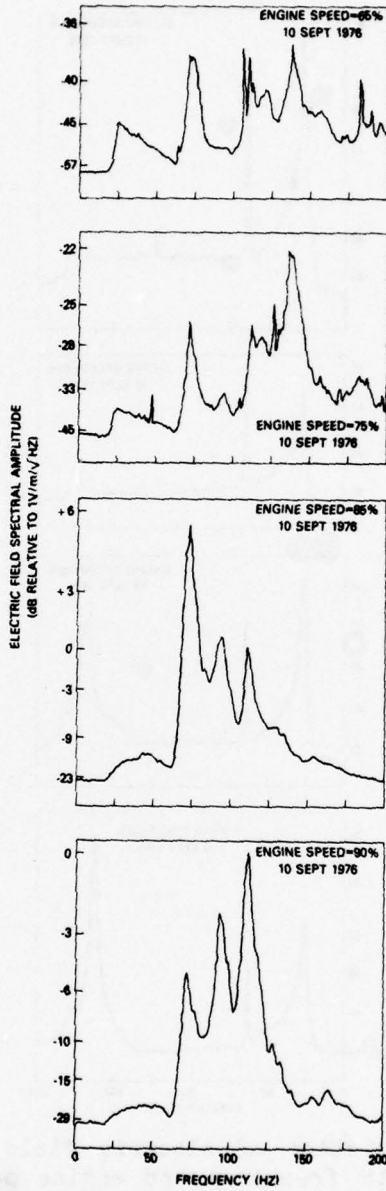
Fig. 4 - Variation of electric field spectral amplitude with frequency and engine power setting. 10 September 1976. Aft antenna.
