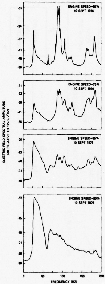
Fig. 3 - Variation of electric field spectral amplitude with frequency and engine power setting. 10 September 1976. Forward antenna.
