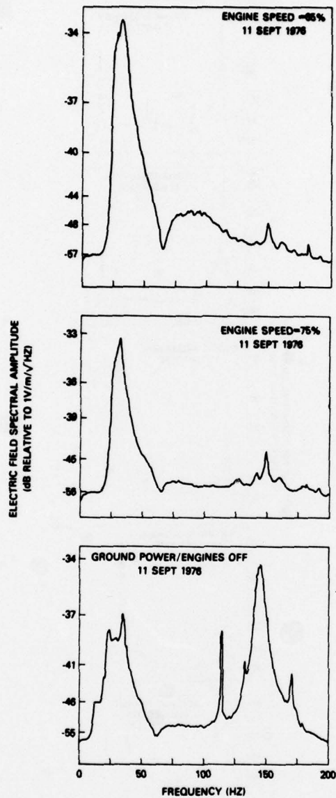
Fig. 11- Variation of electric field spectral amplitude with frequency and engine power setting. 11 September 1976. Center antenna.
