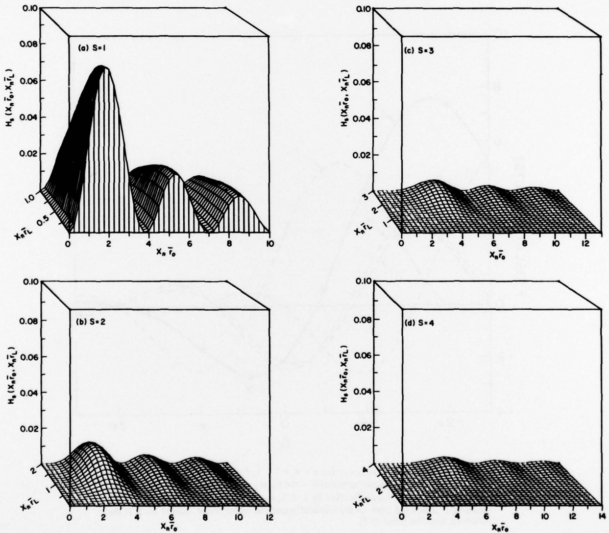
Fig. 5 - Plots of the beam-wave coupling coefficient H_s(x_n \bar{r}_0, x_n \bar{L}) as a function of its arguments for the first four cyclotron harmonics.
