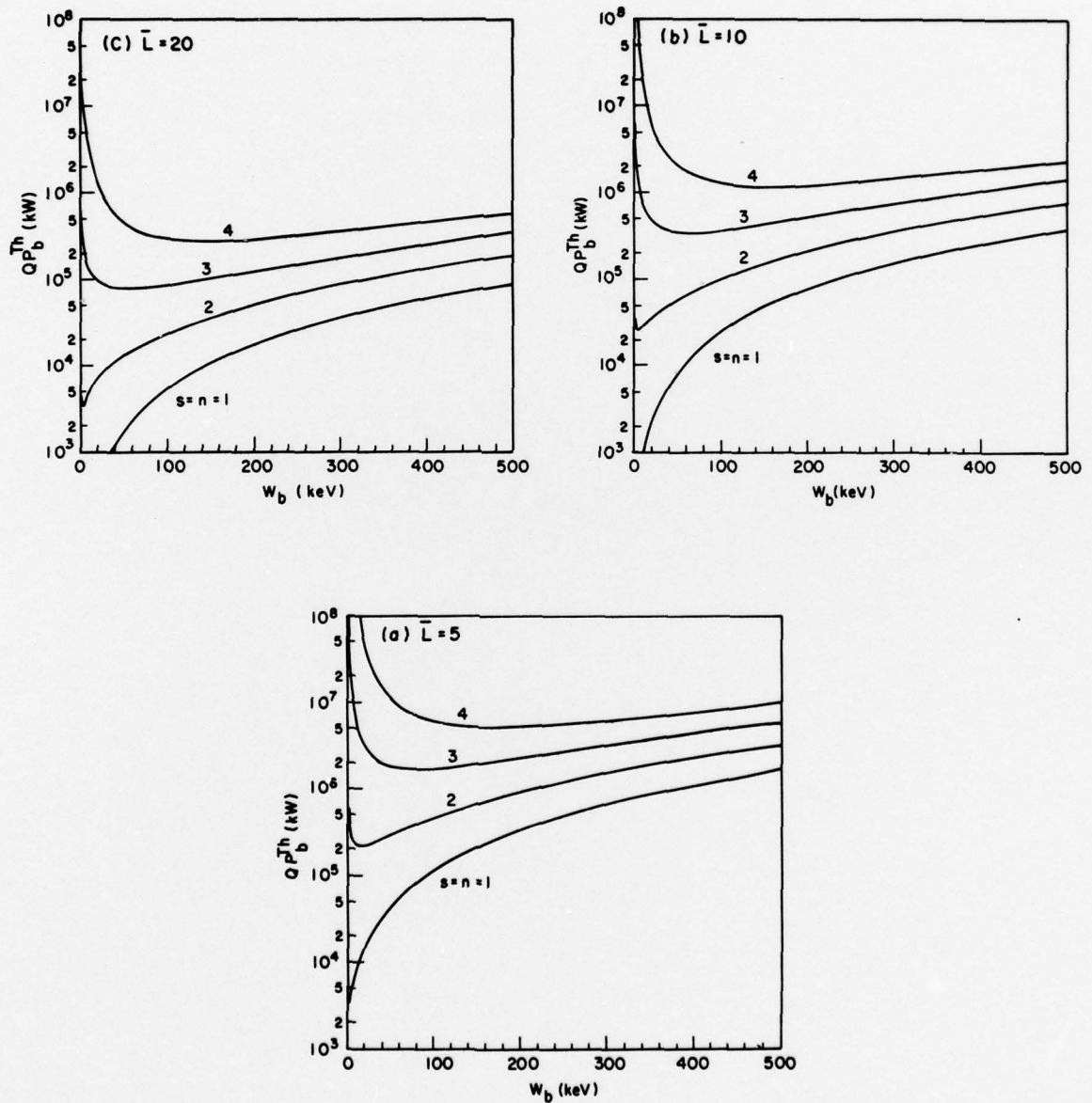
Fig. 7 - Threshold beam power ( P_b^{Th} ) times Q versus beam kinetic energy ( W_b ) for l=1 , n=s , v_{10}/v_{z0} = 1.5 , and (a) \bar{L} = 5 , (b) \bar{L} = 10 , (c) \bar{L} = 20 . The beam guiding center position \bar{r}_0 is so chosen that H_s(x_n \bar{r}_0, x_n \bar{r}_L) falls on its first peak with respect to x_n \bar{r}_0 (see Fig. 5). The magnetic field B_0 has been specified to maximize the beam energy low (see point X on Fig. 6).
