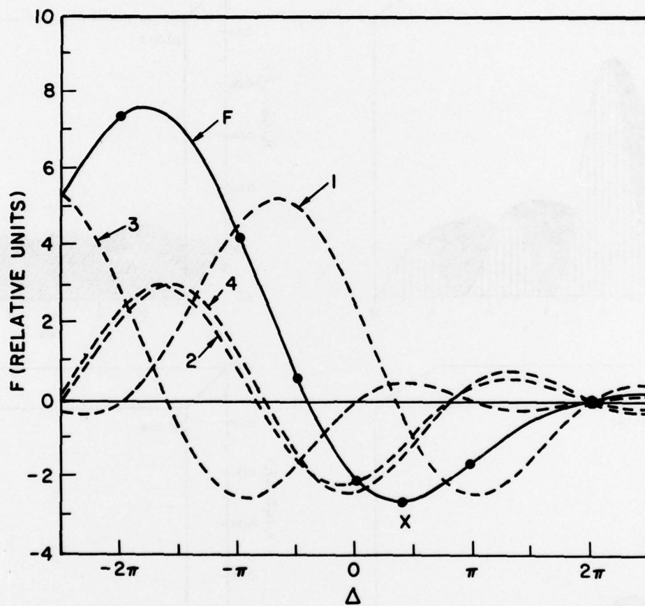
Fig. 6 - F (solid wave) versus \Delta for s = n = l = 1 , V_0 = 0.48 , L = 5 , \gamma_0 = 1.1 , and v_{10}/v_{20} = 1.5 . The four components of F - the \alpha_1, \alpha_2, \alpha_3, and \alpha_4 terms in Eq. (35) are also plotted in dashed curves (marked by 1, 2, 3, and 4, respectively). Solid dots are the values of F calculated from an independent numerical code. Point marked by X is the maximum negative value of F .
