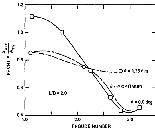
Fig. 14 - Percent Wetted Area for Low L/B SES
