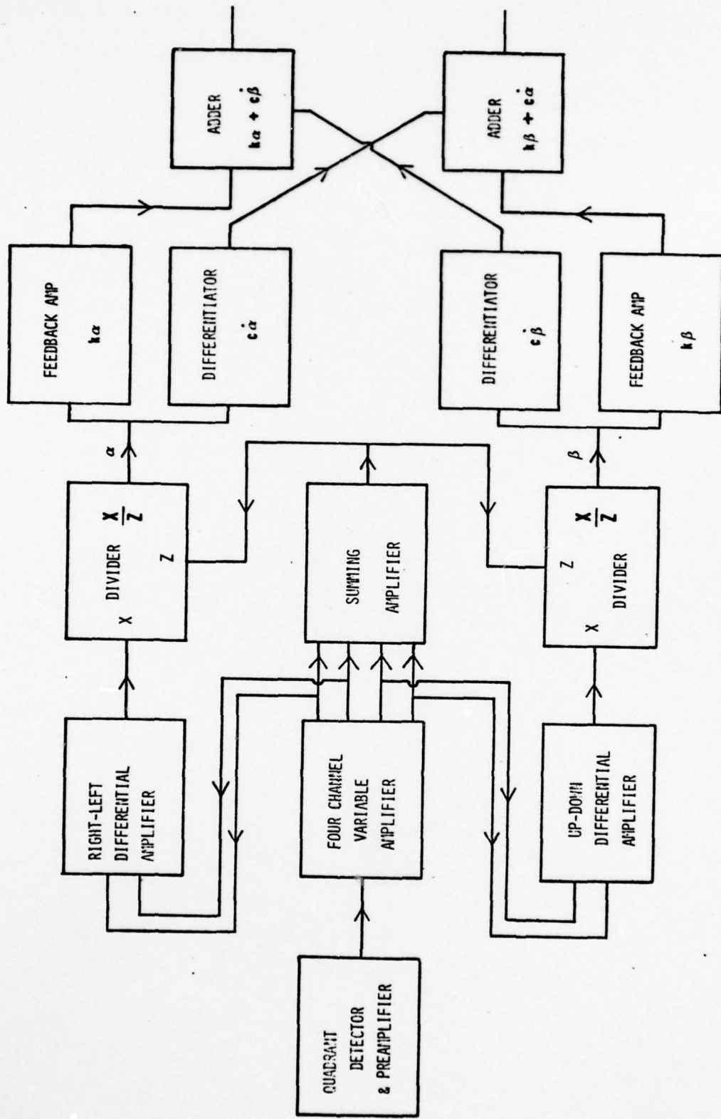
Figure 2 Control System Block Diagram
