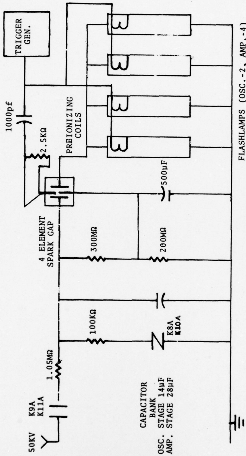
Figure 12 - CAPACITOR CHARGE AND DISCHARGE SYSTEM
