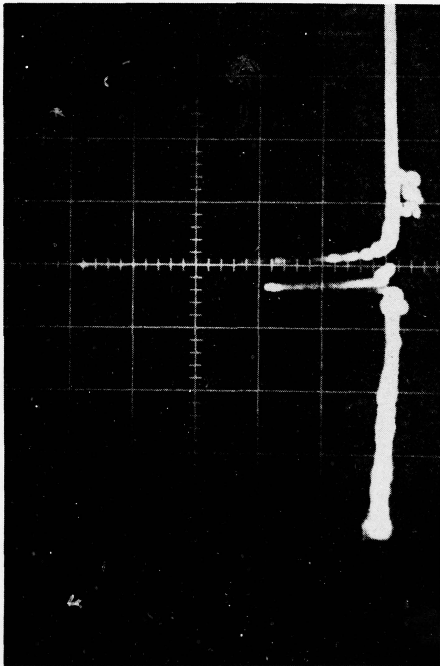
Figure 29 - Q-SWITCHED TOTAL SYSTEM OUTPUT (total amplifier cell pressure = 460 torr, argon with 60 torr C F I, sweep 5 \mu s/div.)
