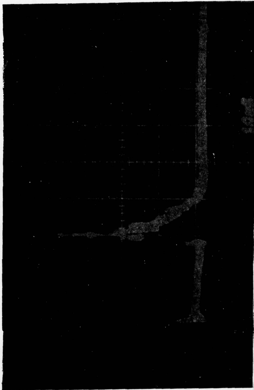
Figure 26 - Q-SWITCHED TOTAL SYSTEM OUTPUT (total amplifier cell pressure = 160 torr, argon with 60 torr C 3 F 7 I, sweep 10 \mu s/div.)
