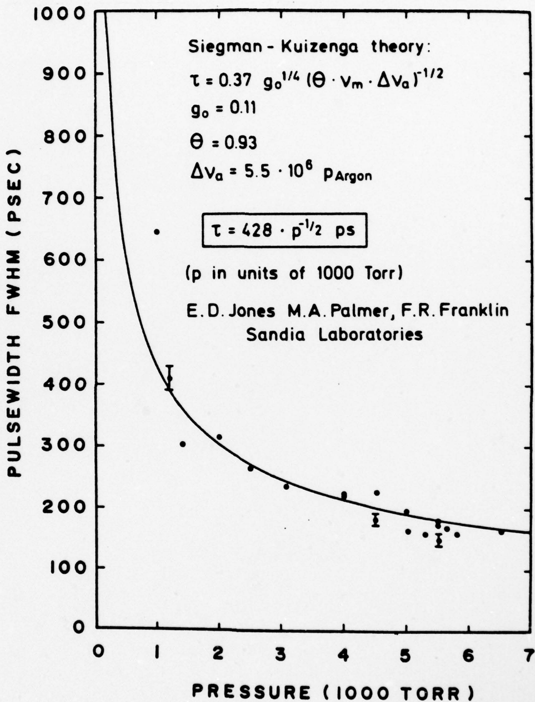
Figure 21 - PULSE WIDTH DEPENDENCE ON TOTAL CELL PRESSURE
