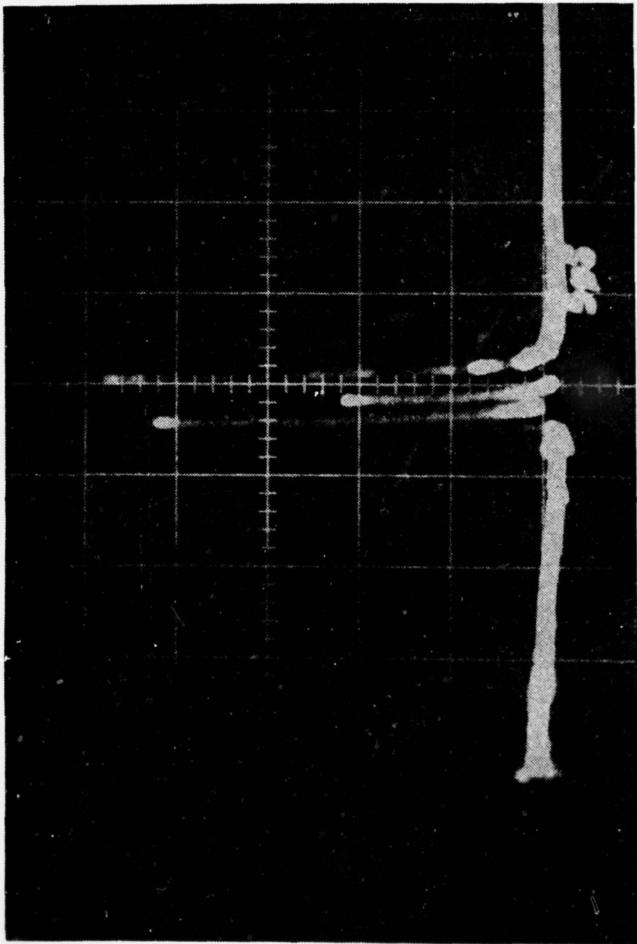
Figure 28 - Q-SWITCHED TOTAL SYSTEM OUTPUT (total amplifier cell pressure = 360 torr, argon with 60 torr C F I, sweep 5 \mu s/div.)
