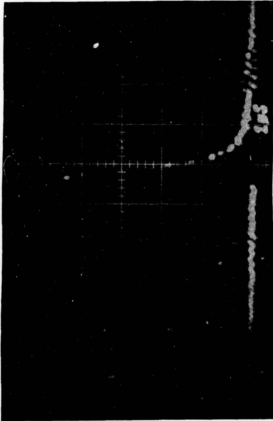
Figure 32 - GIANT PULSE AT CALCULATED BEST TIME (total amplifier cell pressure = 660 torr, argon with 60 torr C 3 F 7 I, sweep 1 \mu s/div.)
