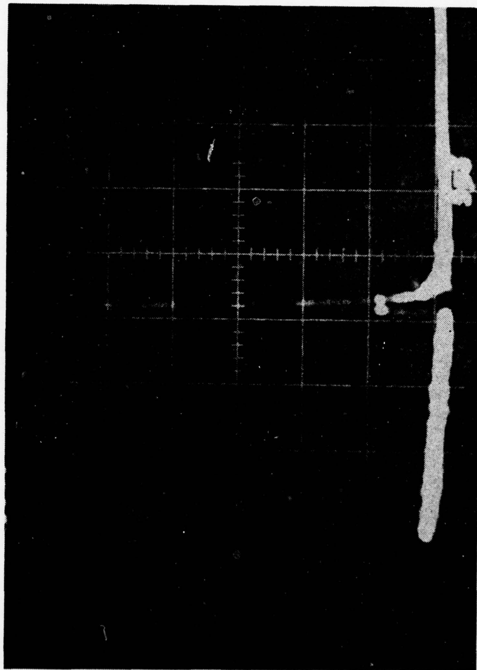
Figure 30 - Q-SWITCHED TOTAL SYSTEM OUTPUT (total amplifier cell pressure = 560 torr, argon with 60 torr C 3 F 4 I, sweep 5 \mu s/div.)
