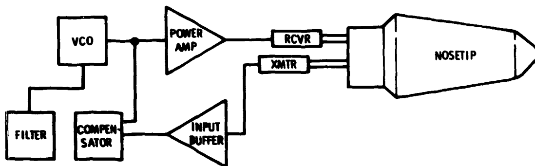
Figure 2-25. Noretip Acoustic Instrumentation
