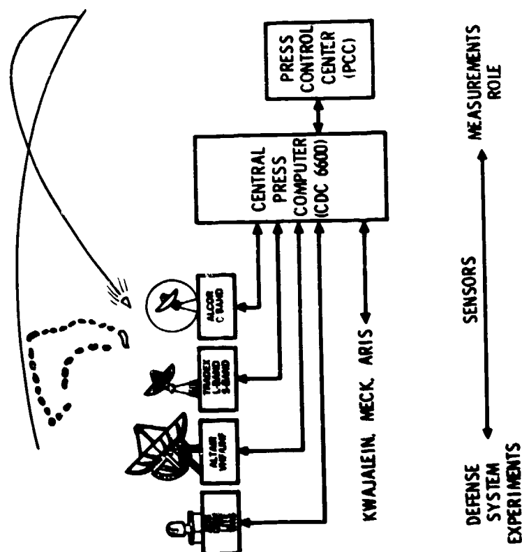
Figure 6-1. KREMS Instrumentation
