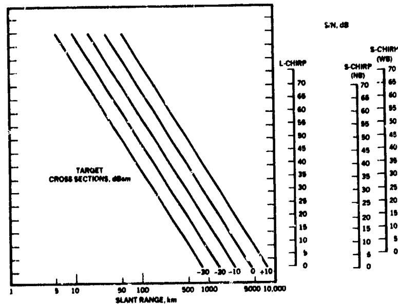
Figure 6-5. TRADEX Sensitivity
