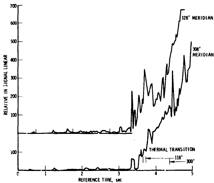
Figure 5-27. Kaman Detector
