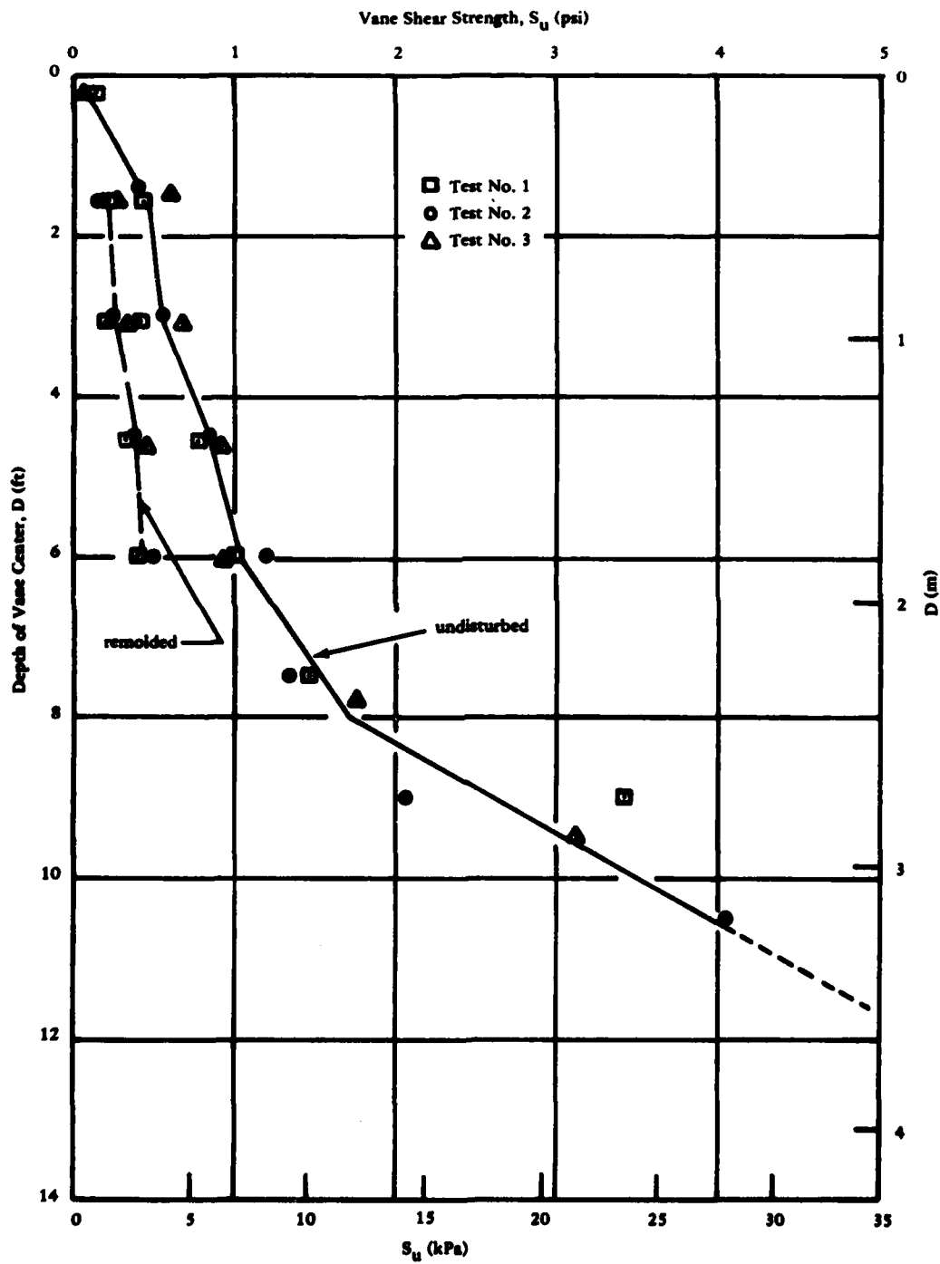
Figure 10. In-situ vane shear strength versus depth for CEL 29-m site in Santa Barbara Channel.
