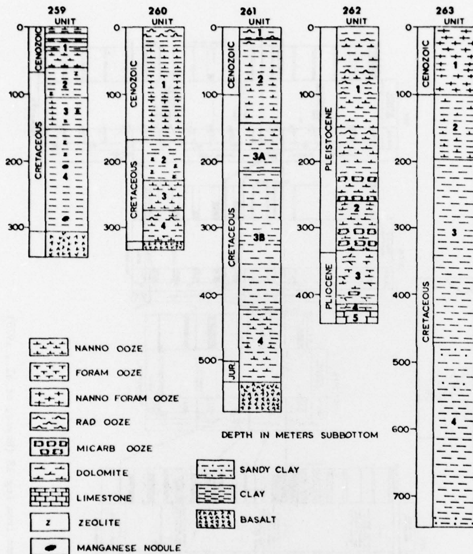
Fig. 11. Lithofacies sections from Leg 27 (Veevers, et al., 1975).
