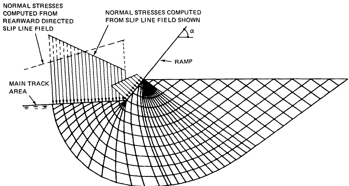
Fig. 7 Front Slip Line Field modified to Include Part of the Main Track Area
