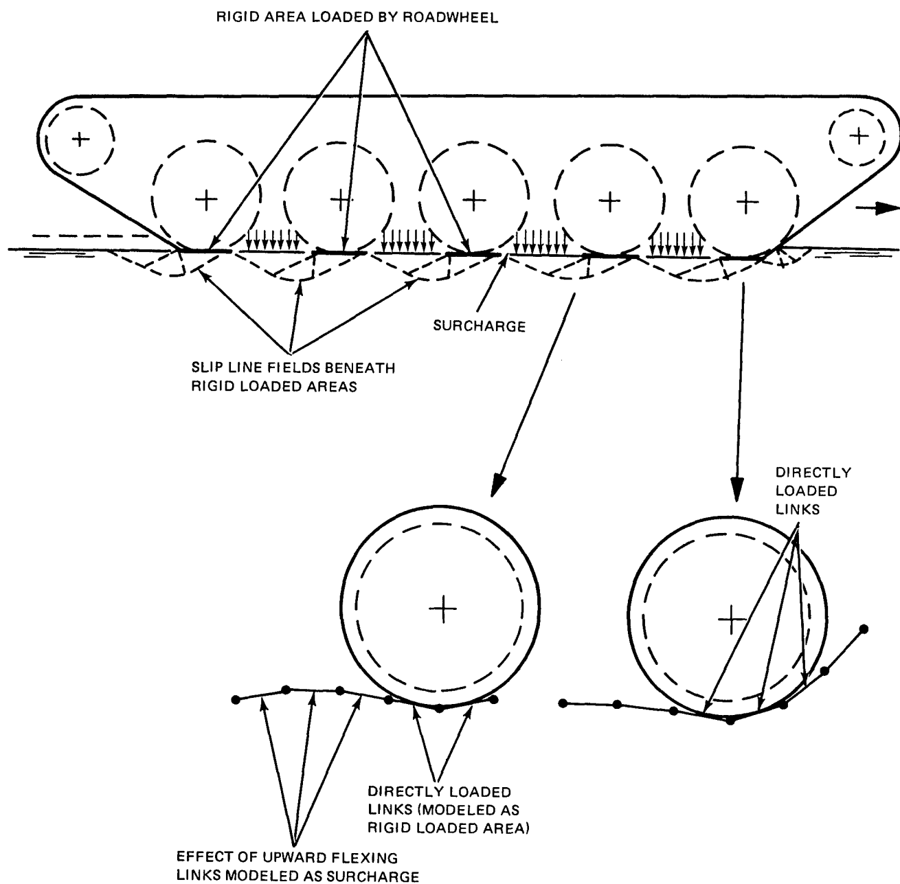
Fig. 11 Concept of Semirigid Track-Soil Interaction Model
