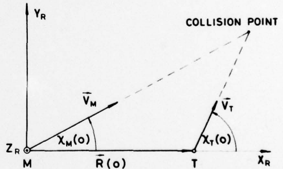
Fig. 1. Initial collision geometry
