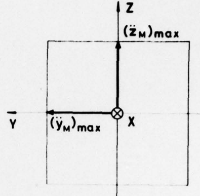
Fig. 5. Vectogram of cruciform missile.
