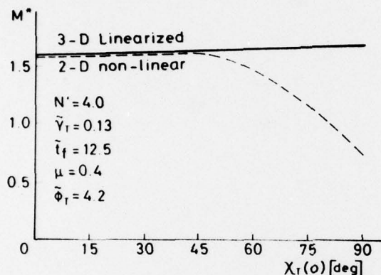
Fig. 8. Comparison of 3-D and 2-D tactics.
