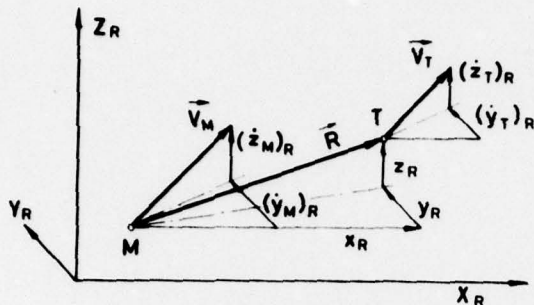
Fig. 2. 3-D pursuit-evasion geometry
