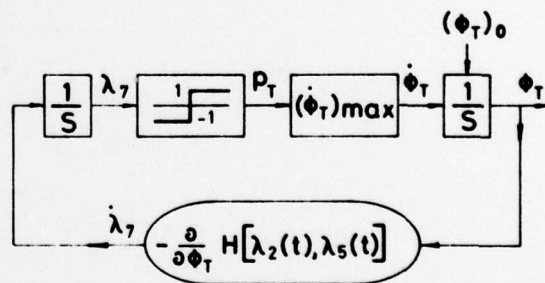
Fig. 7. Roll rate as control variable.
