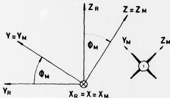
Fig. 3. Roll orientation of missile maneuver planes.
