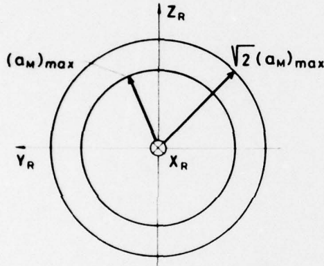
Fig. 4. Circular vectogram of missile acceleration.
