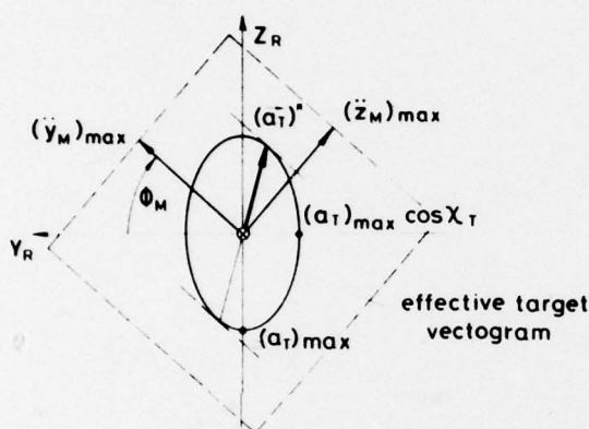
Fig. 6. Minimization of the effective missile-target maneuver ratio.
