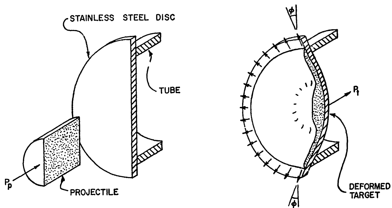
Figure 14. Impact onto disk mounted normal to trajectory.
