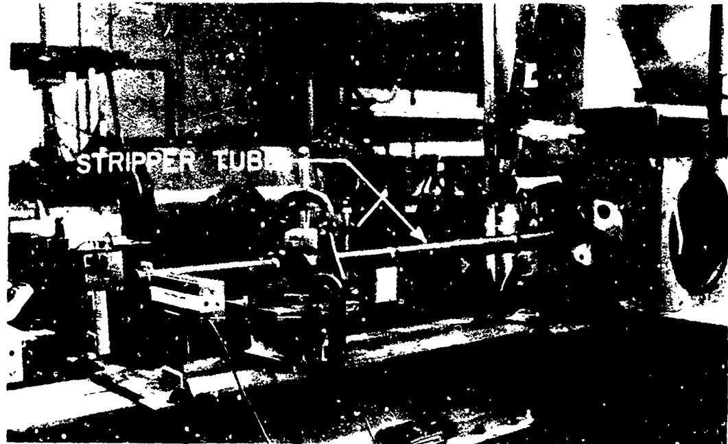
Figure 7. Sabot stripper.
