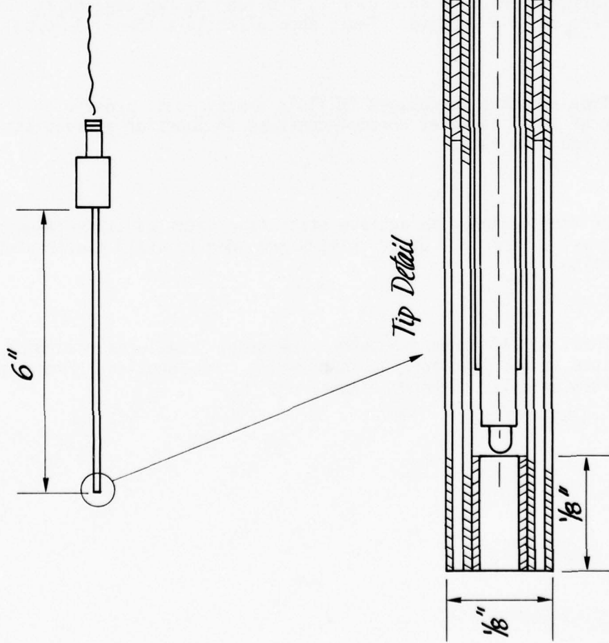
Figure 33. Aspirated Thermocouple Probe
