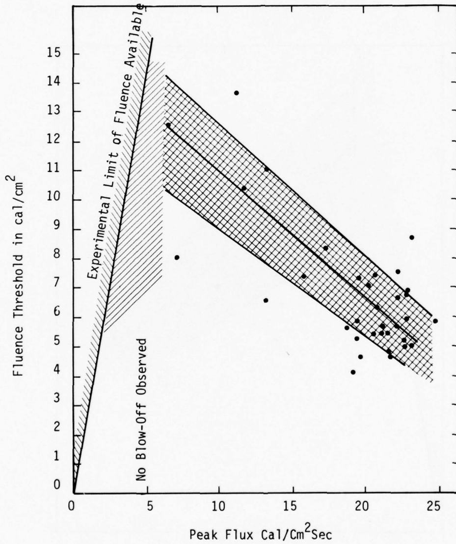
Figure 11. Fluence Threshold for Particle Ejection vs. Peak Flux (Sample 14)
