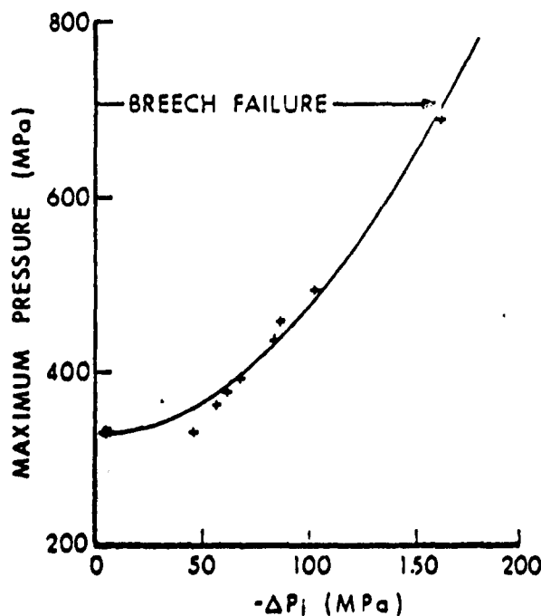
Figure 5. Pressure Wave Sensitivity for the 175-mm M107 Gun (M86A2 (Zone 3) Propelling Charge)
