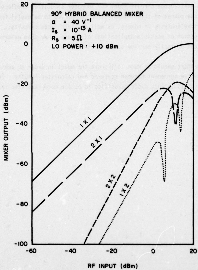
Figure 12. Calculated Single-Tone IMD Response for a 90° Hybrid Balanced Mixer
