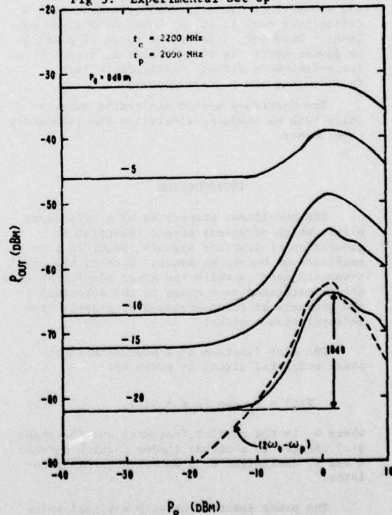
Fig 4: Measured power output at 2\omega_c - \omega_p as a function of the pump power P_p , with the carrier power P_c as a parameter.
