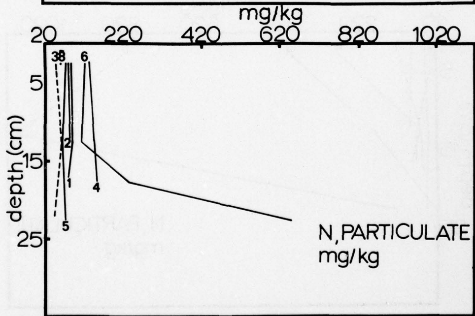
Figure B93. Distribution of particulate carbon and nitrogen in sediment cores taken from stations sampled on cruise Y7501 B
