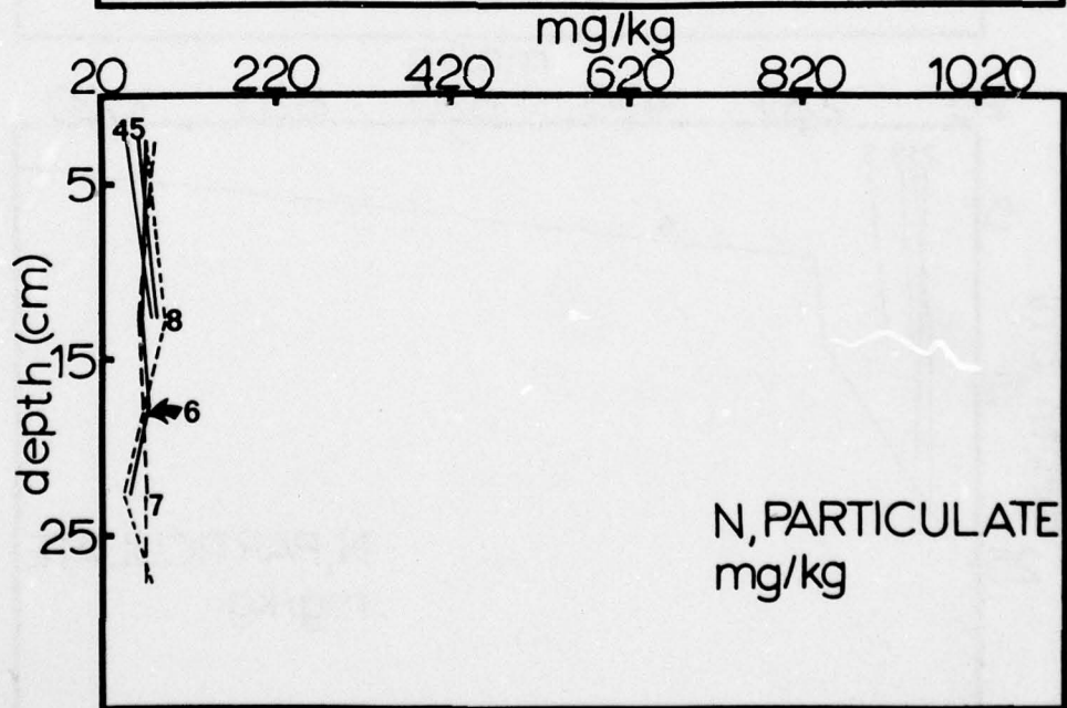
Figure B94. Distribution of particulate carbon and nitrogen in sediment cores taken from stations sampled on cruise Y7506 B-2
