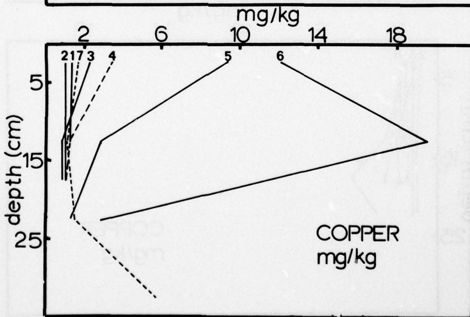
Figure B112. Distribution of manganese and copper in sediment cores taken from stations sampled on cruise Y7409 F
