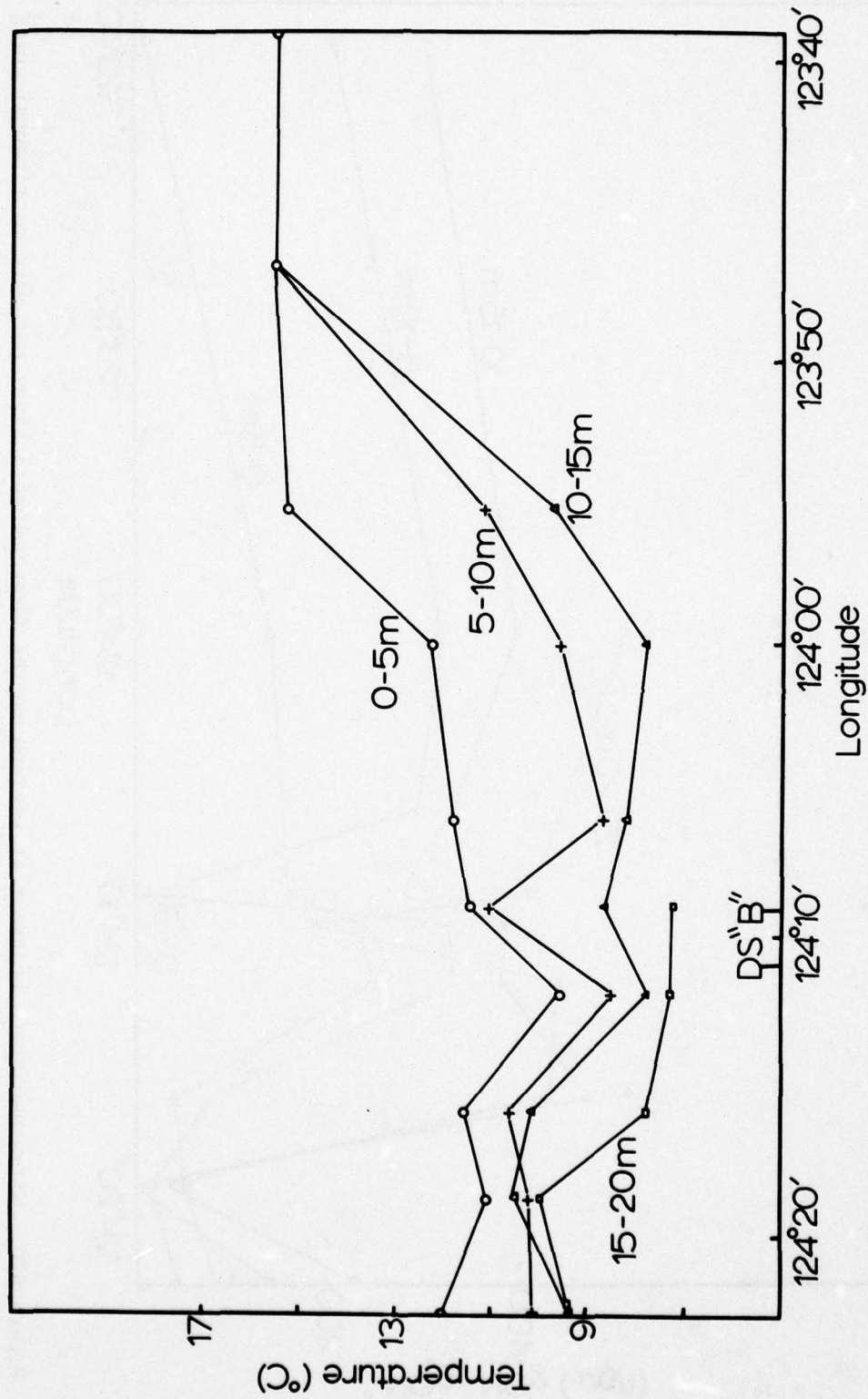
Figure B69. Temperature transect at various depths from Columbia River out onto continental shelf
