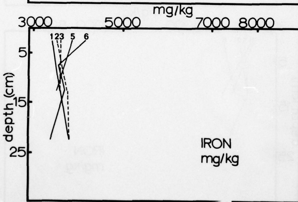
Figure B110. Distribution of nickel and iron in sediment cores taken from stations sampled on cruise Y7508 D-2
