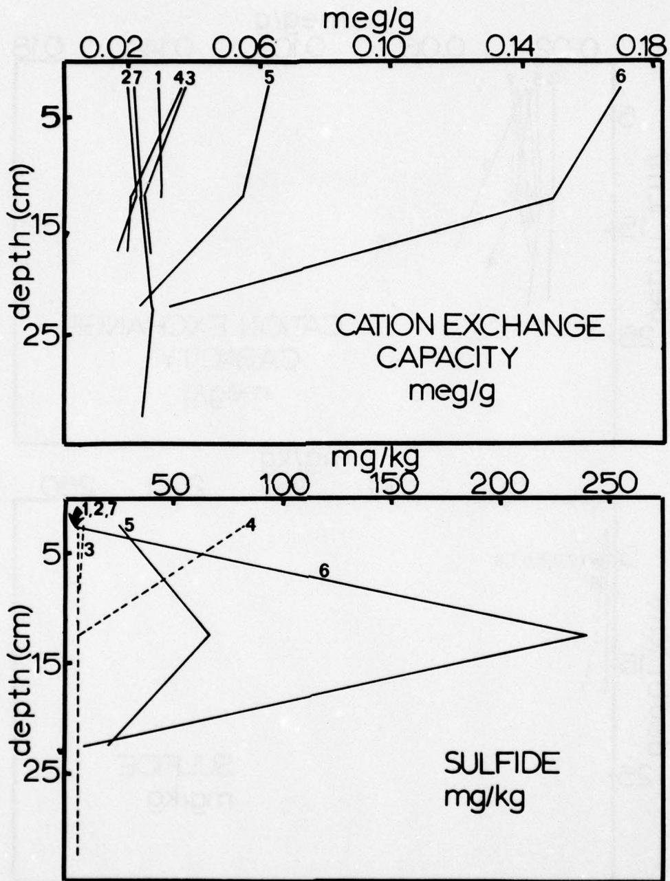
Figure B102. Distribution of cation exchange capacity and sulfide in sediment cores taken from stations sampled on cruise Y7409 F
