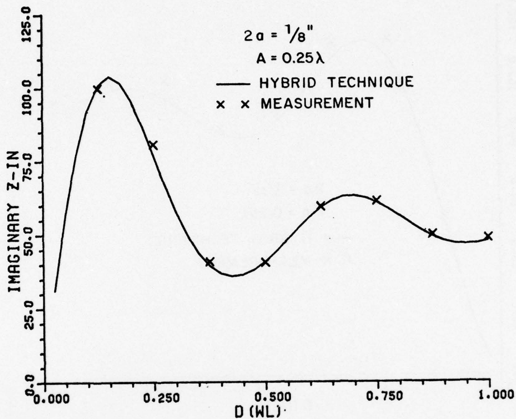
Figure 34b. Imaginary part of axial dipole input impedance near cylinder of radius A=0.25\lambda .
