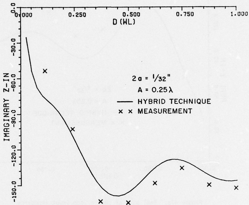
Figure 47b. Imaginary part of square loop input impedance near cylinder of radius A=0.25\lambda .
