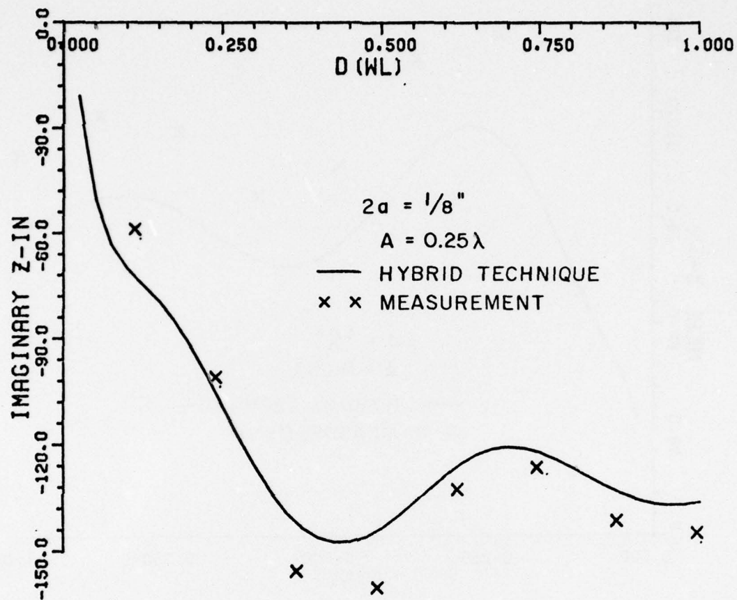
Figure 44b. Imaginary part of square loop input impedance near cylinder of radius A=0.25\lambda .
