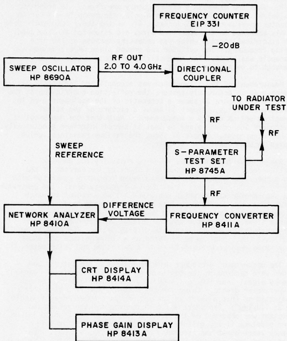
Figure 30. Block diagram of experimental measurement setup.
