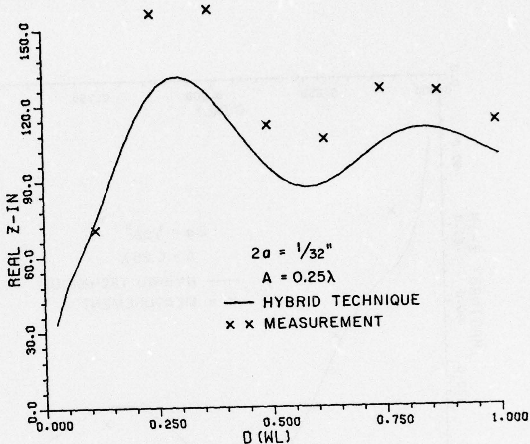
Figure 47a. Real part of square loop input impedance near cylinder of radius A=0.25\lambda .
