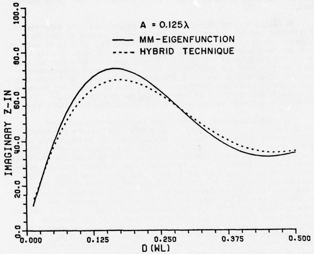
Figure 28b. Imaginary part of axial dipole input impedance near cylinder of radius A=0.125\lambda .
