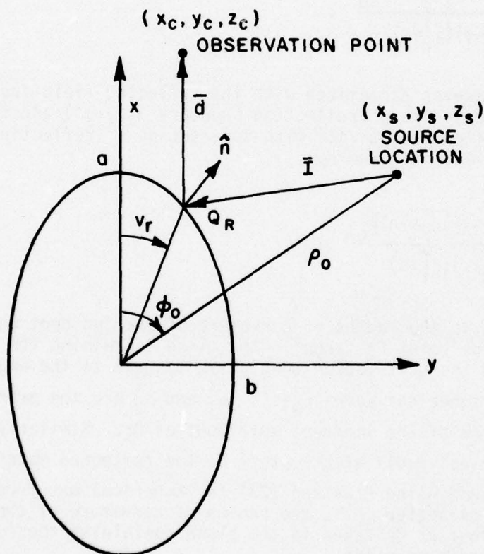
Figure 8. Geometry for determination of reflection point on elliptic cylinder.
