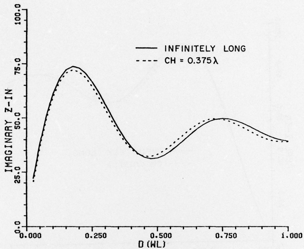
Figure 50b. Imaginary part of axial dipole input impedance near cylinder of radius A=0.25\lambda .
