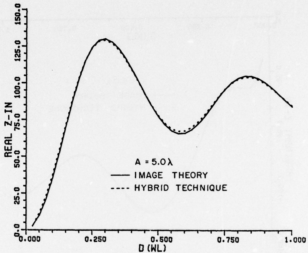
Figure 43a. Real part of square loop input impedance near cylinder of radius A=5.0\lambda .
