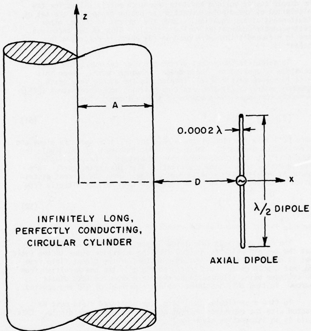
Figure 9. Half-wave dipole axially oriented a distance D from a perfectly conducting circular cylinder of radius A .
