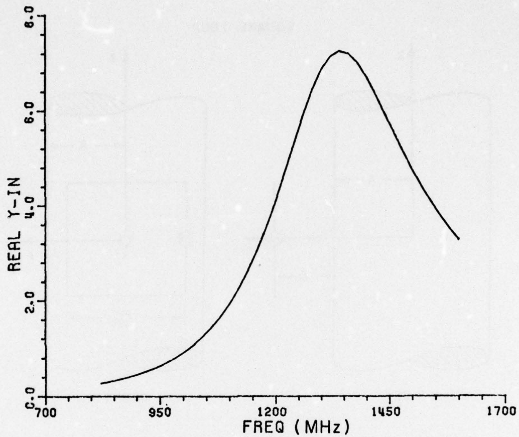
Figure 42a. Real part of the input admittance of the square loop as a function of frequency.
