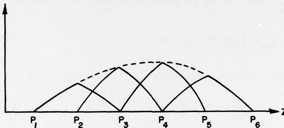
Figure 3. Current distribution modeled by overlapping piecewise sinusoidal modes.
