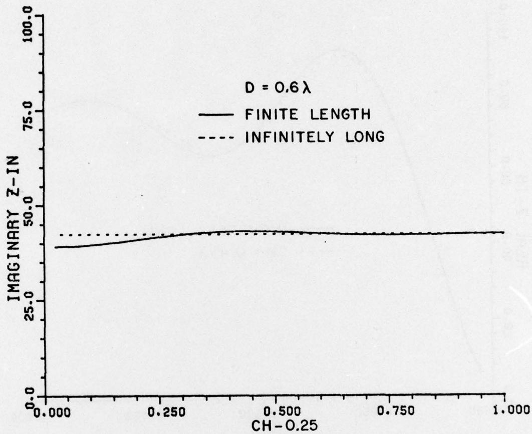
Figure 52b. Imaginary part of input impedance of dipole as a function of cylinder height above dipole.
