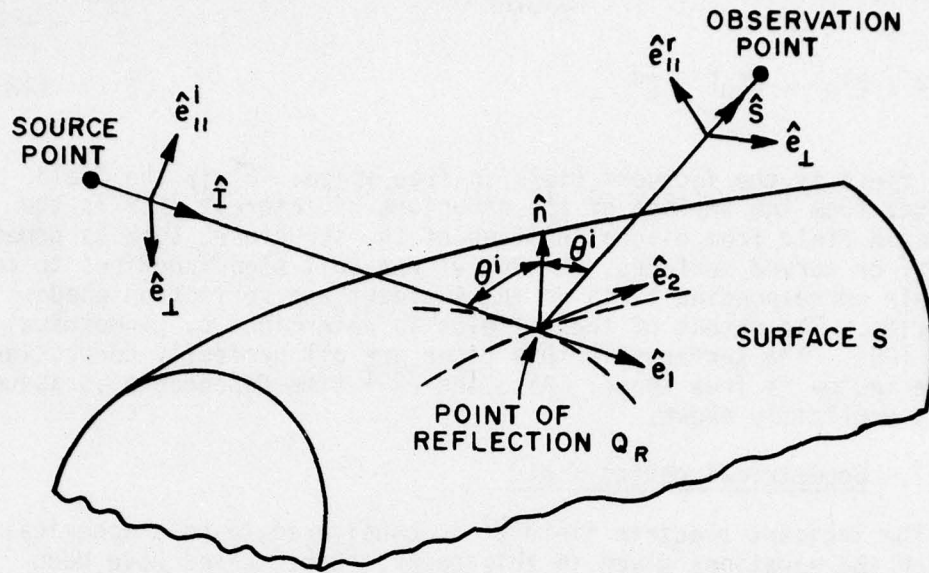
Figure 5. Reflection by a smooth convex surface.
