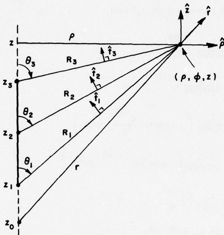
Figure 22. Z-directed center fed dipole source with observation point (\rho, \phi, z) .
