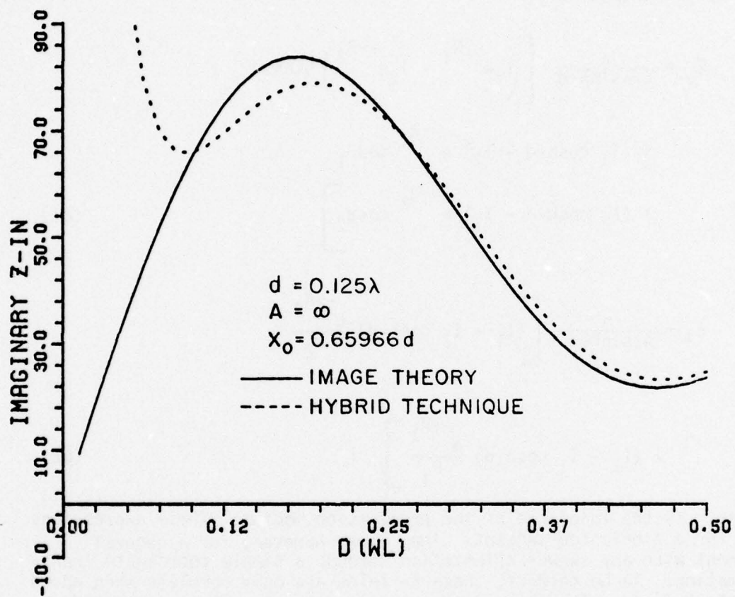
Figure 19b. Imaginary part of axial dipole input impedance near cylinder of radius A=\infty .
