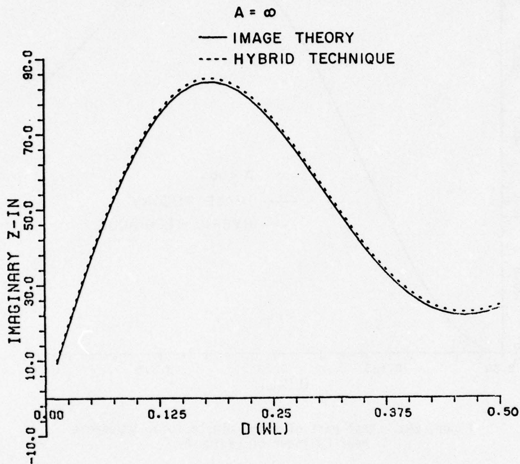
Figure 29b. Imaginary part of axial dipole input impedance near cylinder of radius A=\infty .
