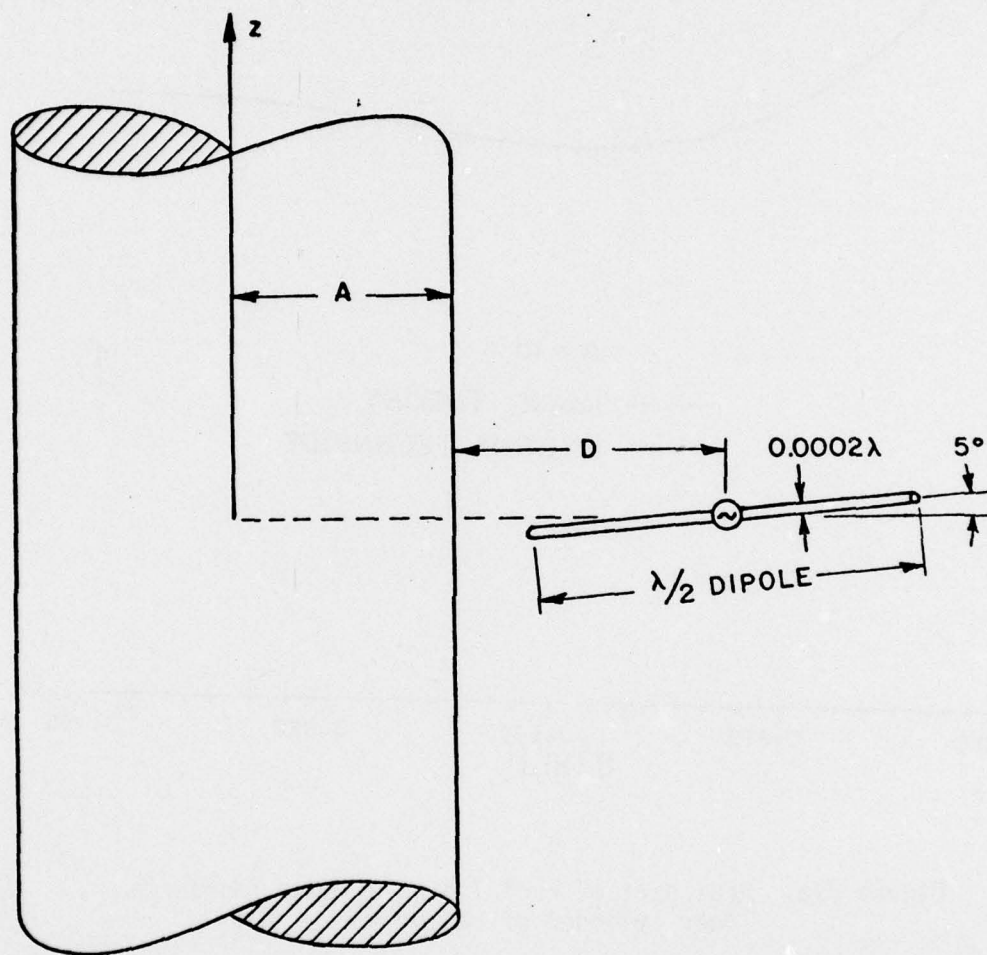
Figure 38. Geometry for a radial dipole tilted 5^\circ .
