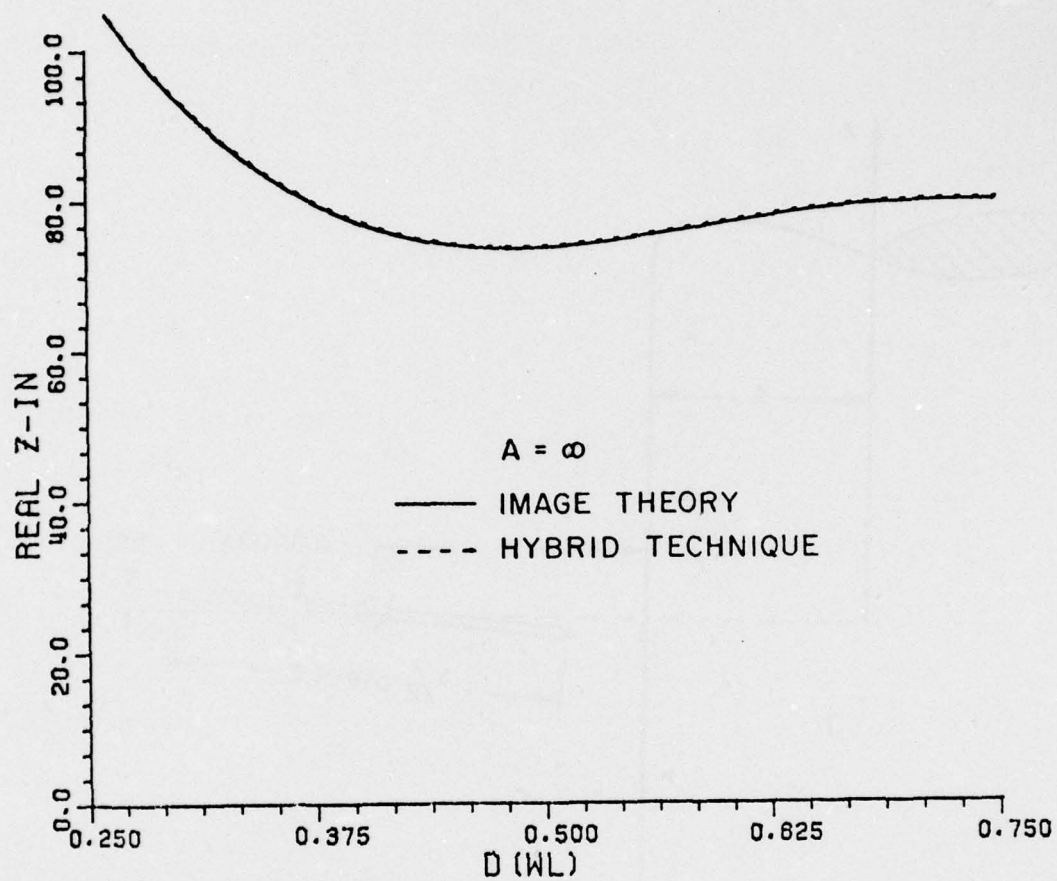
Figure 39a. Real part of radial dipole input impedance near cylinder of radius A=\infty .
