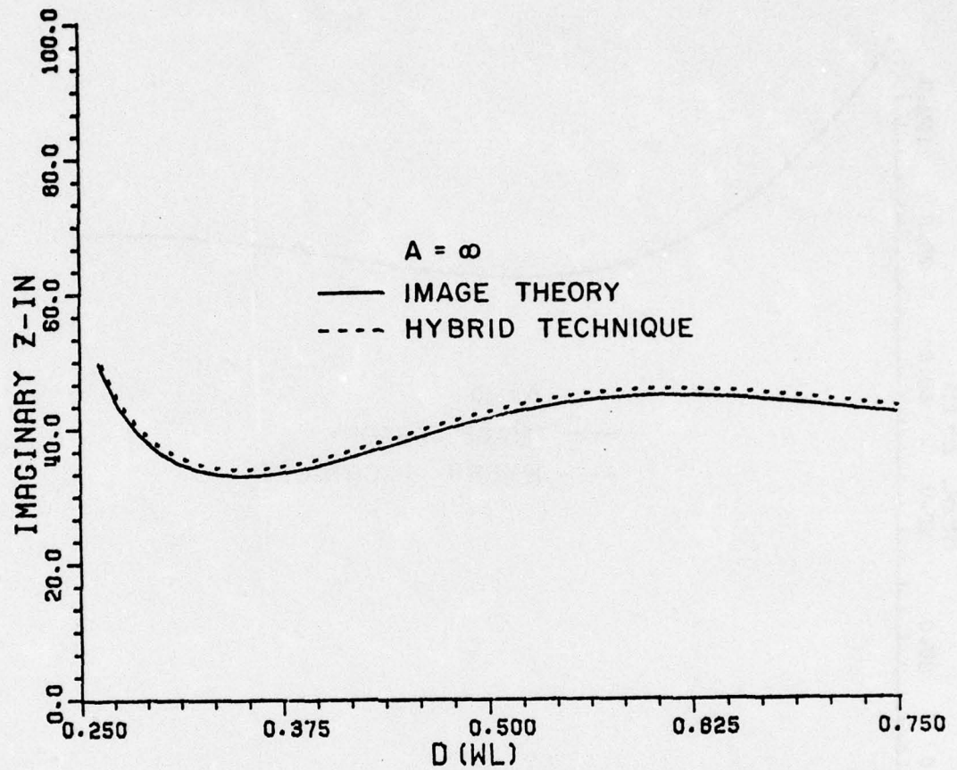
Figure 39b. Imaginary part of radial dipole input impedance near cylinder of radius A=\infty .
