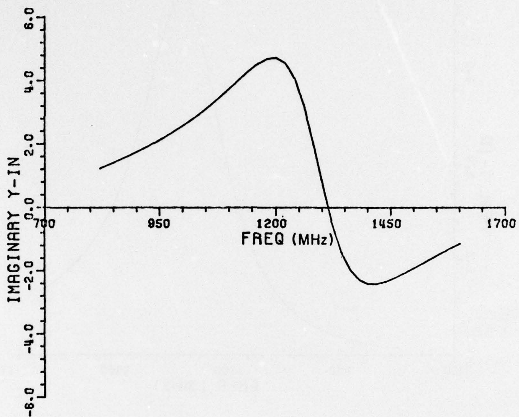
Figure 45b. Imaginary part of the input admittance of the square loop as a function of frequency.
