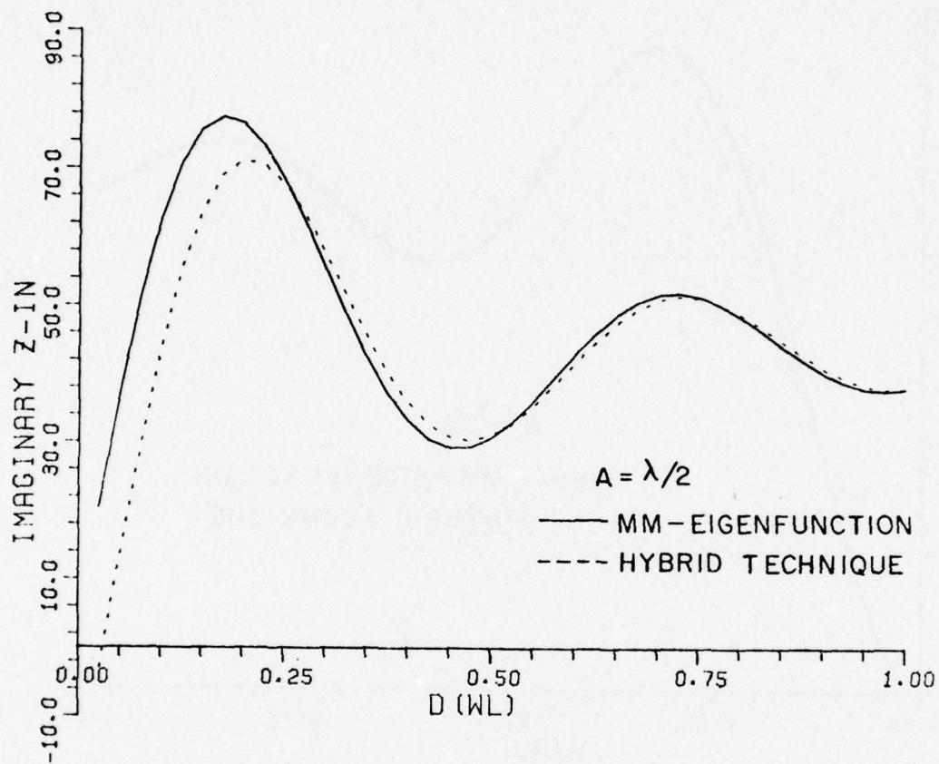
Figure 11b. Imaginary part of axial dipole input impedance near cylinder of radius A=0.5\lambda .
