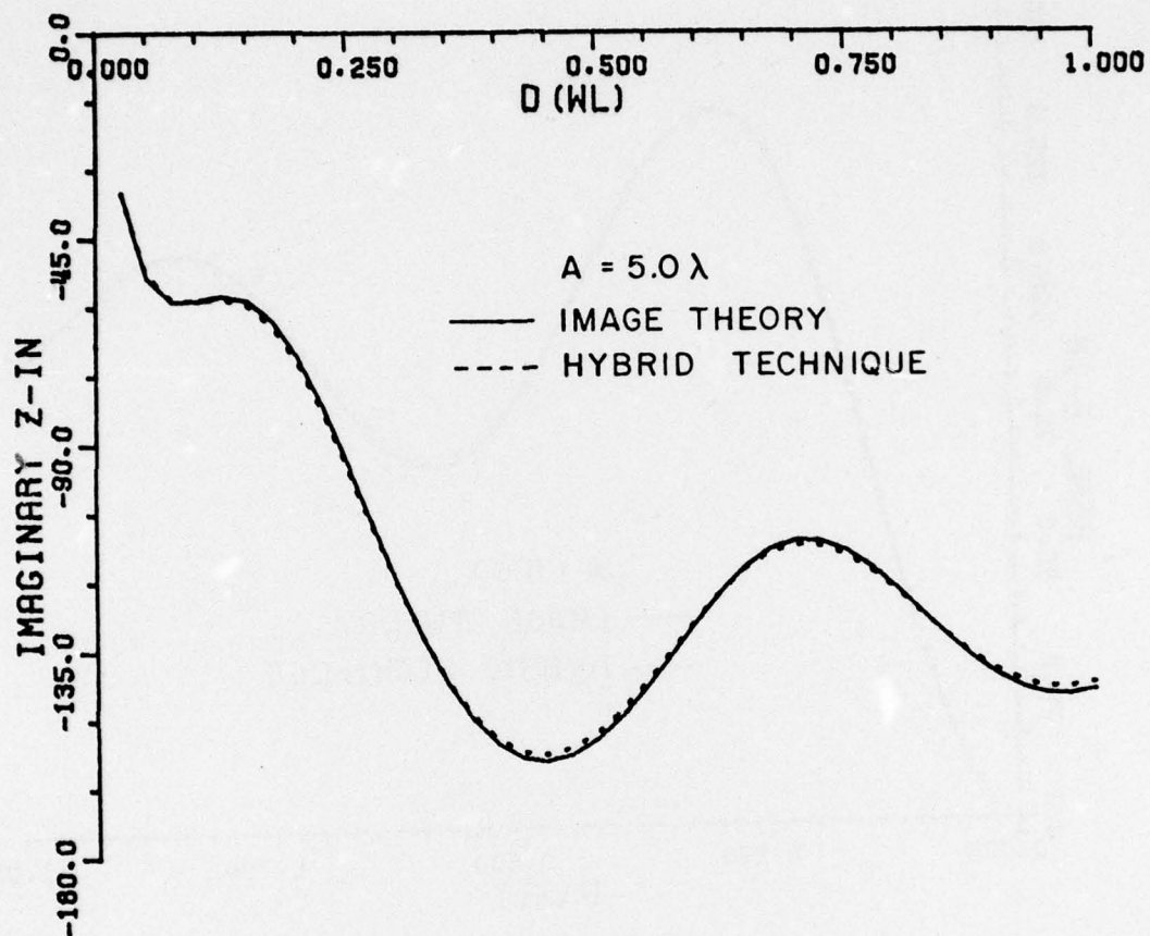
Figure 43b. Imaginary part of square loop input impedance near cylinder of radius A=5.0\lambda .
