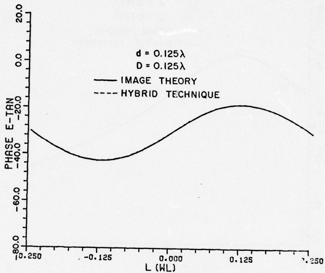
Figure 21b. Phase of E-field tangent to axial dipole along its length with endpoint separation.
