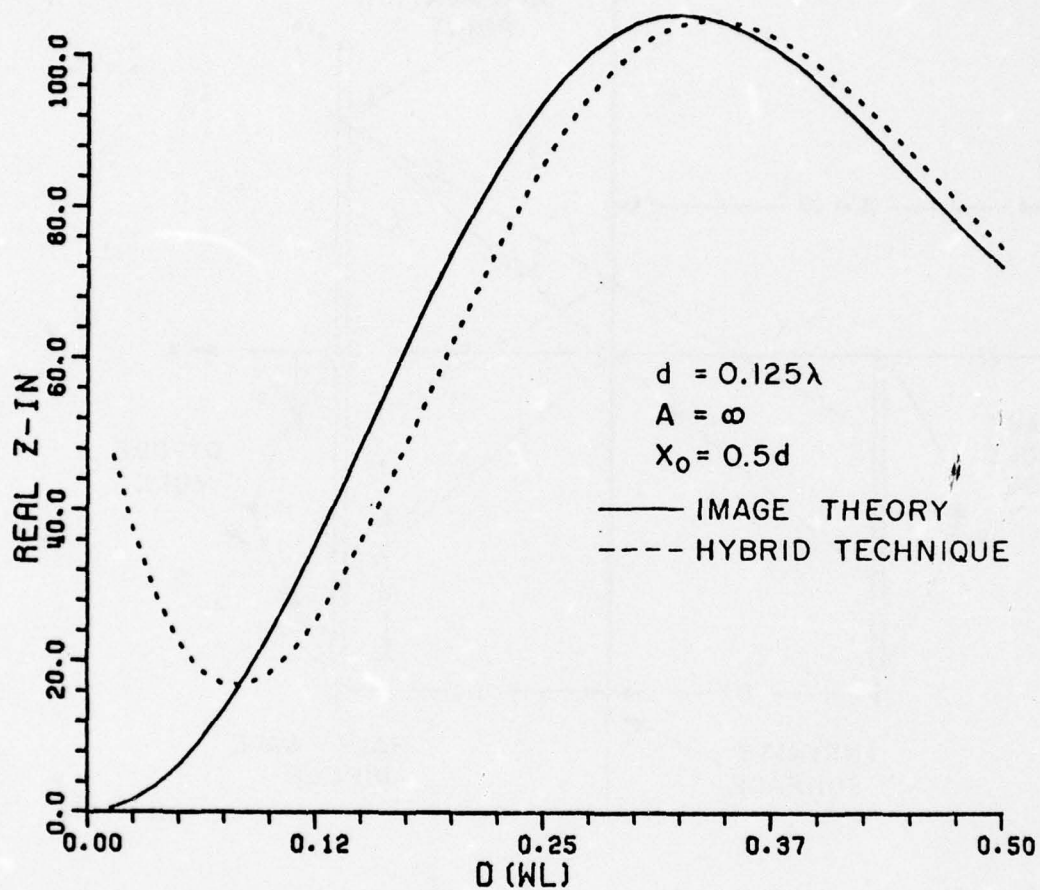
Figure 13a. Real part of axial dipole input impedance near cylinder of radius A=\infty .
