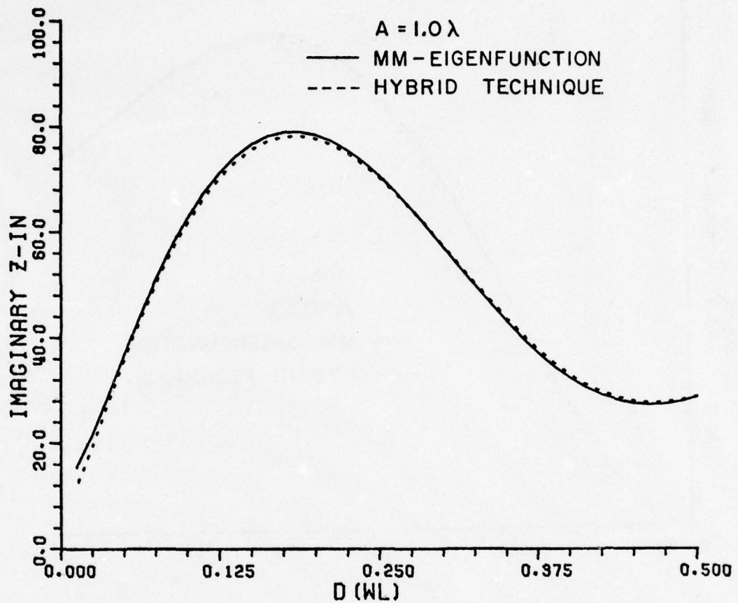
Figure 25b. Imaginary part of axial dipole input impedance near cylinder of radius A=1.0\lambda .
