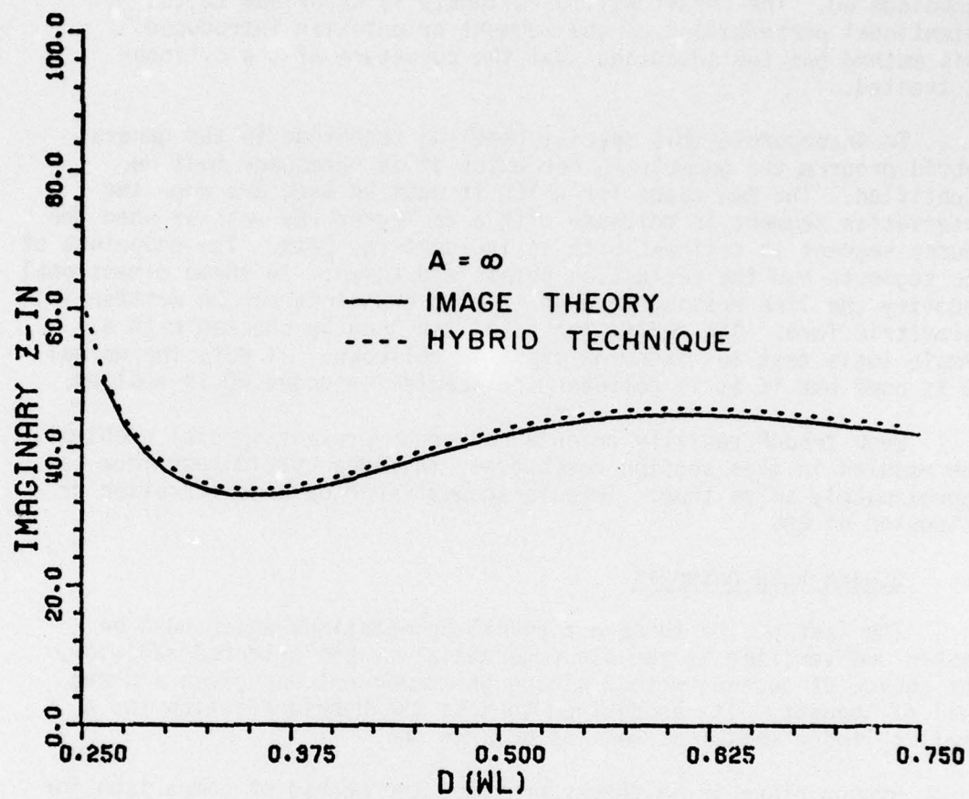
Figure 40b. Imaginary part of radial dipole input impedance near cylinder of radius A=\infty .
