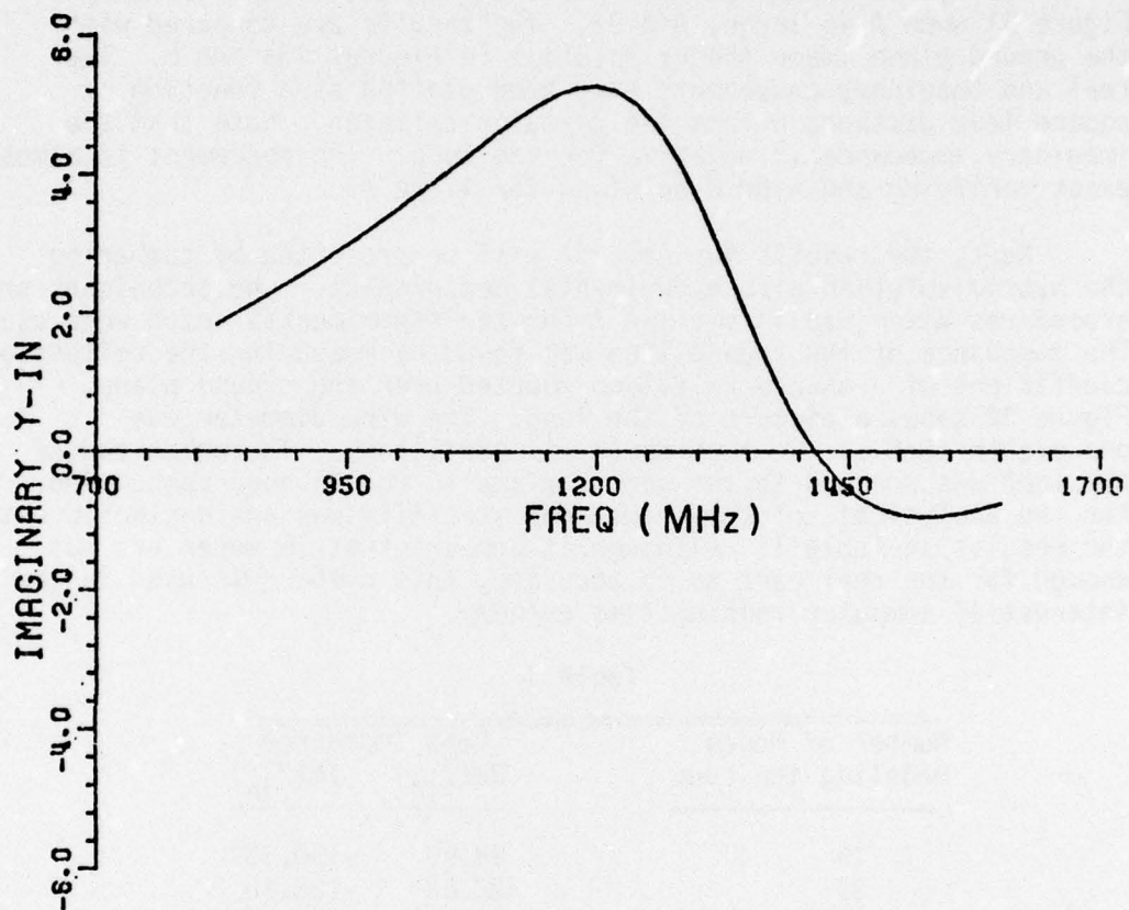
Figure 42b. Imaginary part of the input admittance of the square loop as a function of frequency.
