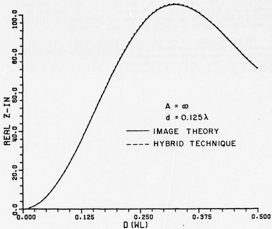
Figure 23a. Real part of axial dipole input impedance near cylinder of radius A=\infty .
