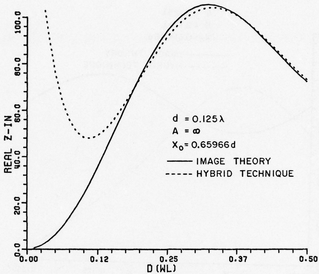
Figure 19a. Real part of axial dipole input impedance near cylinder of radius A=\infty .
