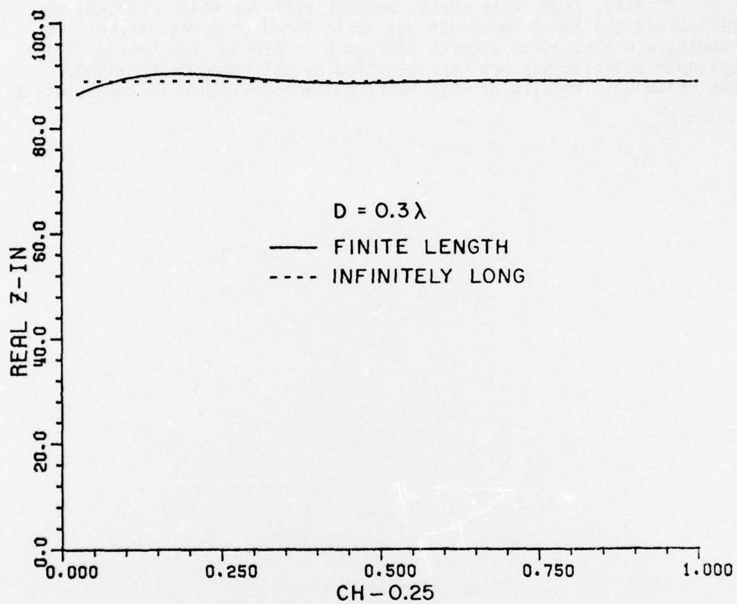
Figure 51a. Real part of input impedance of dipole as a function of cylinder height above dipole.
