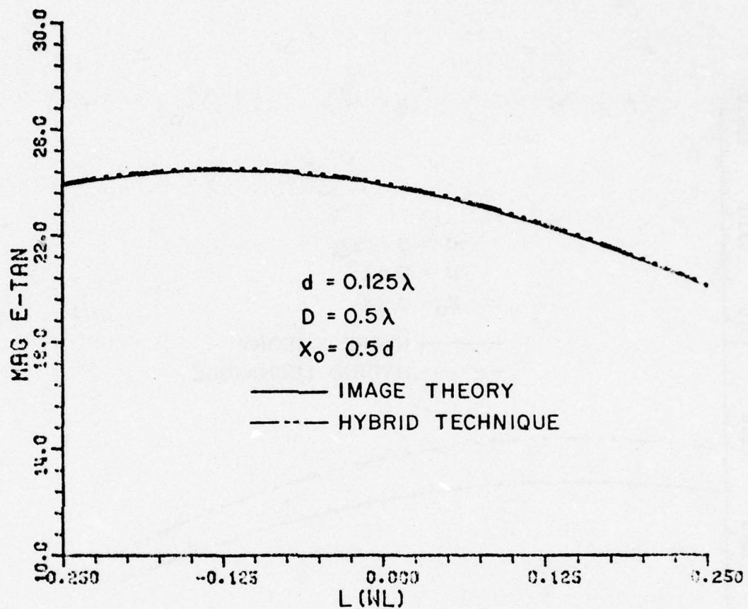
Figure 14a. Magnitude of E-field tangent to axial dipole along its length.
