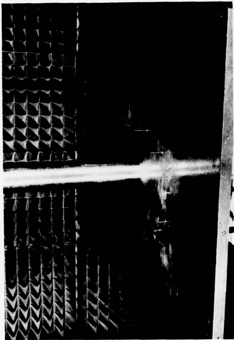
Figure 32. Various antenna measured mounted over ground plane around the cylinder.
