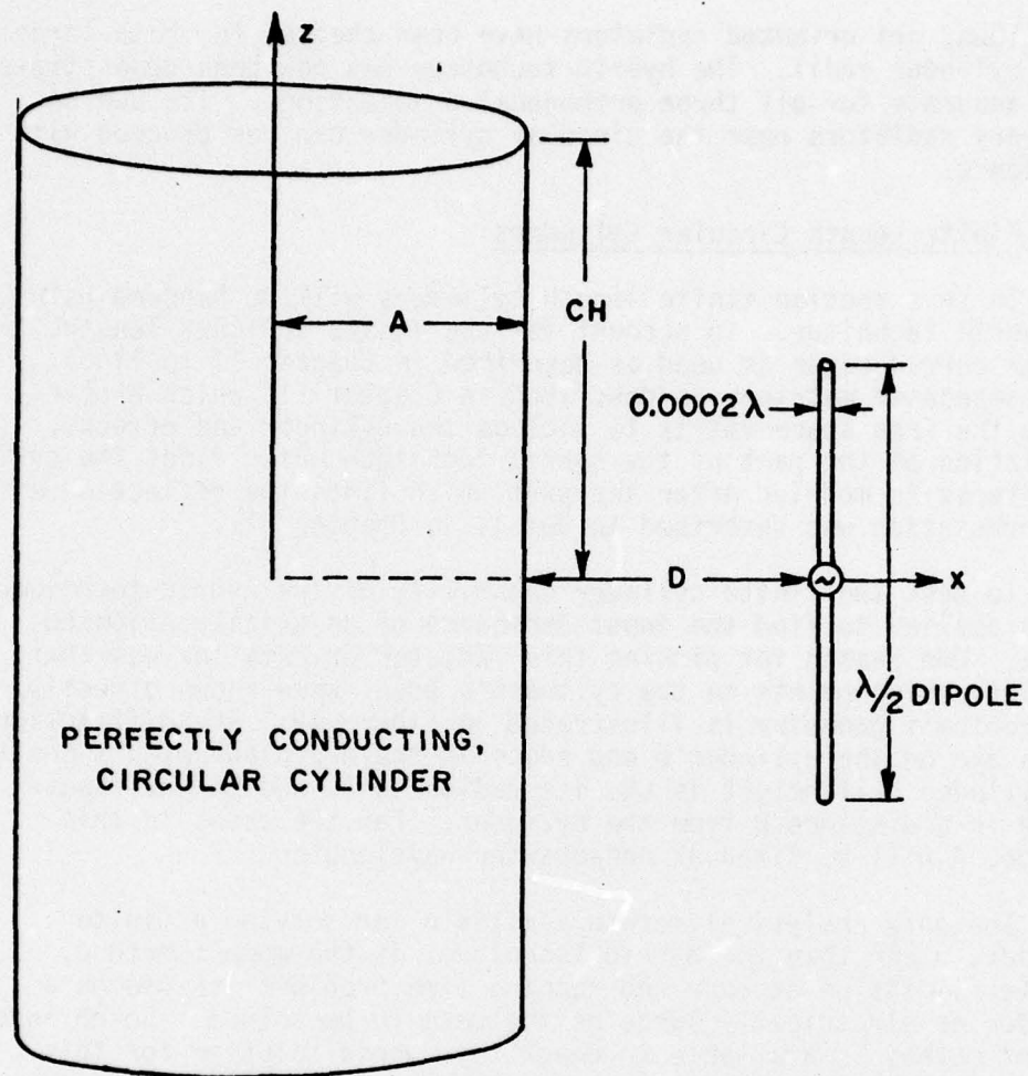
Figure 49. Axial half-wave dipole located near a finite length cylinder.
