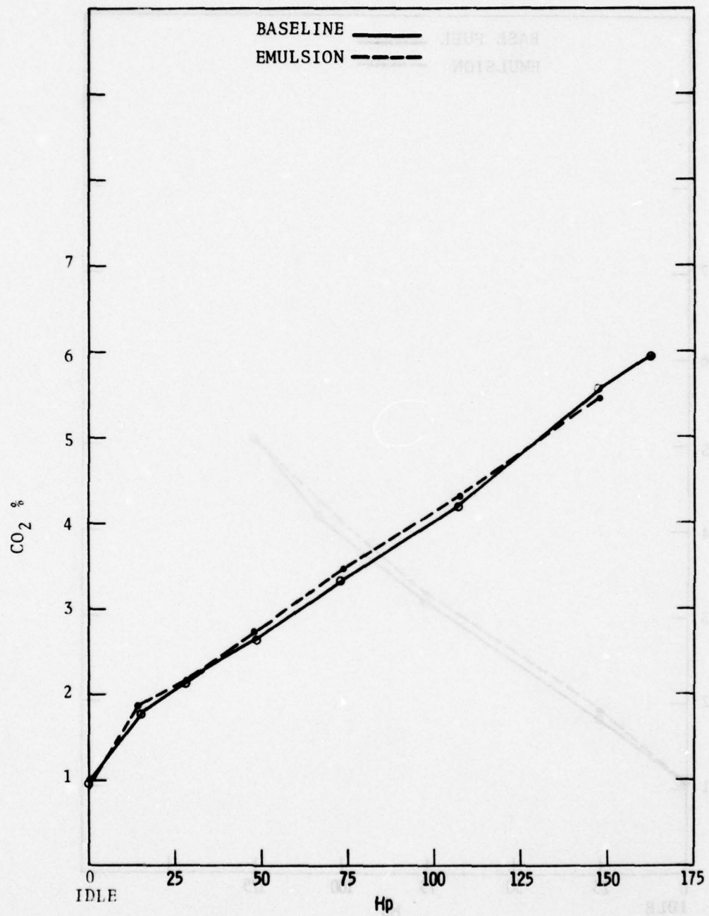
FIGURE 37. CO 2 EMISSIONS: PROP LOAD, 3.6° ADVANCE
