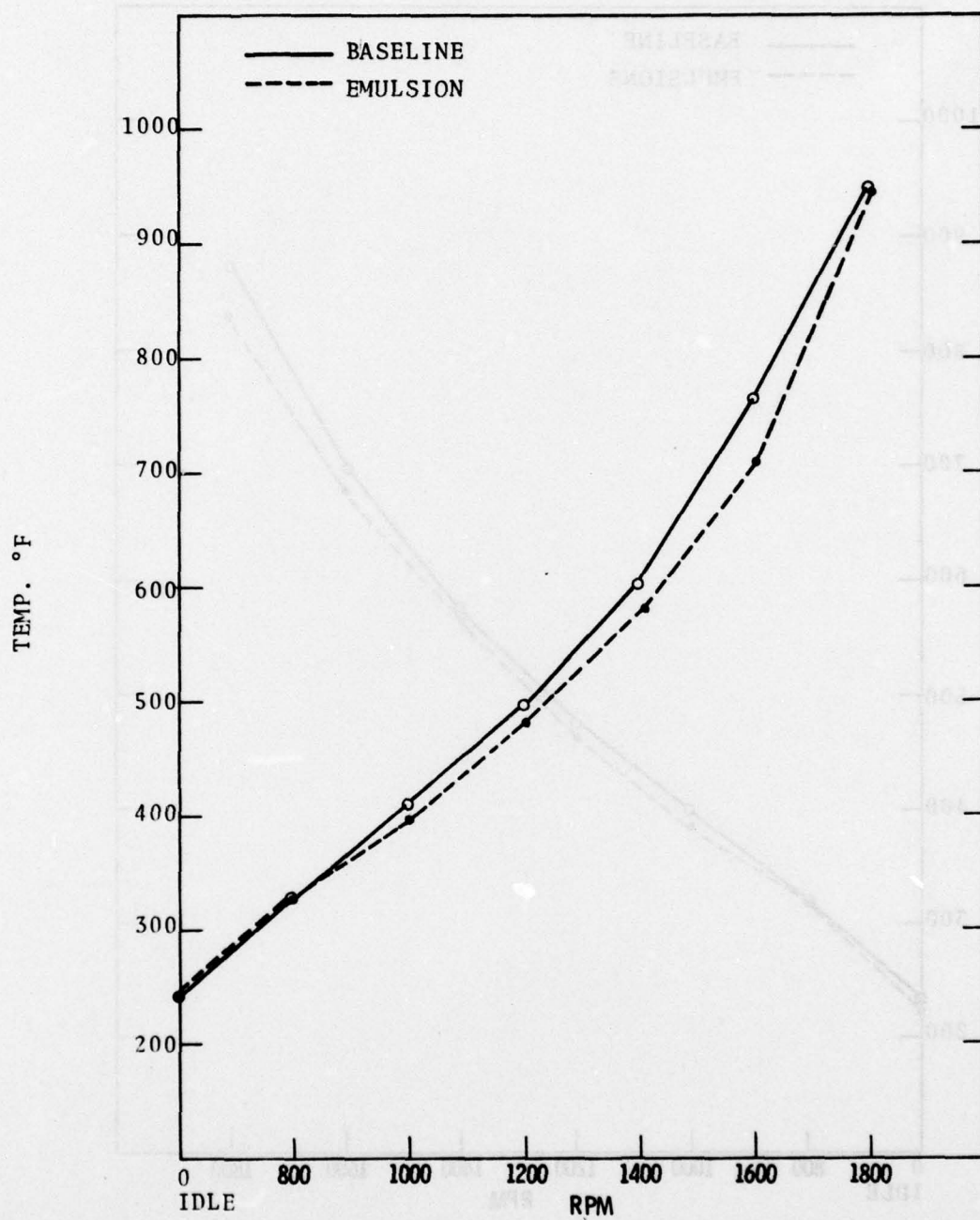
FIGURE 45. EXHAUST TEMP: PROP LOAD, 7.2° RETARD
