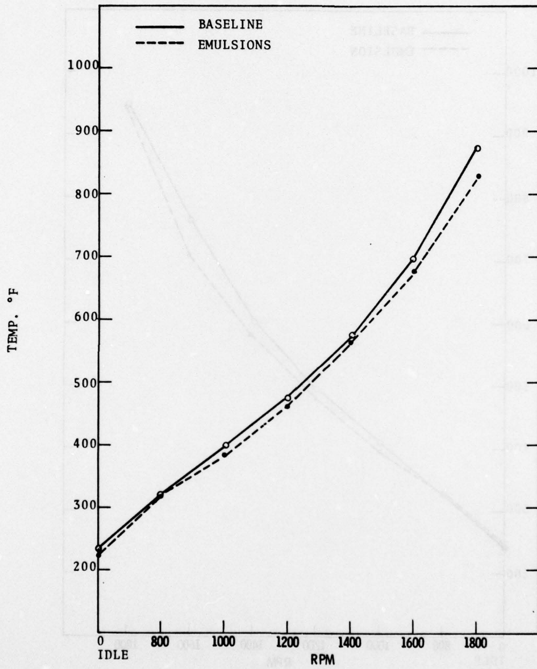
FIGURE 46. EXHAUST TEMP: PROP LOAD, 3.6° ADVANCE
