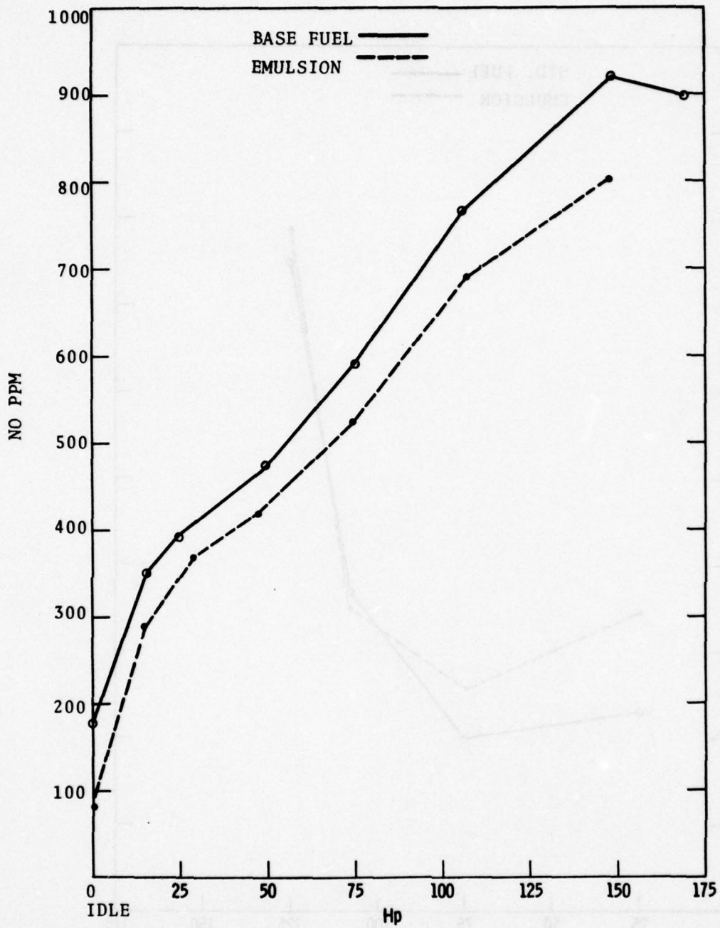
FIGURE 20. NO x EMISSIONS: PROP LOAD, STANDARD TIMING
