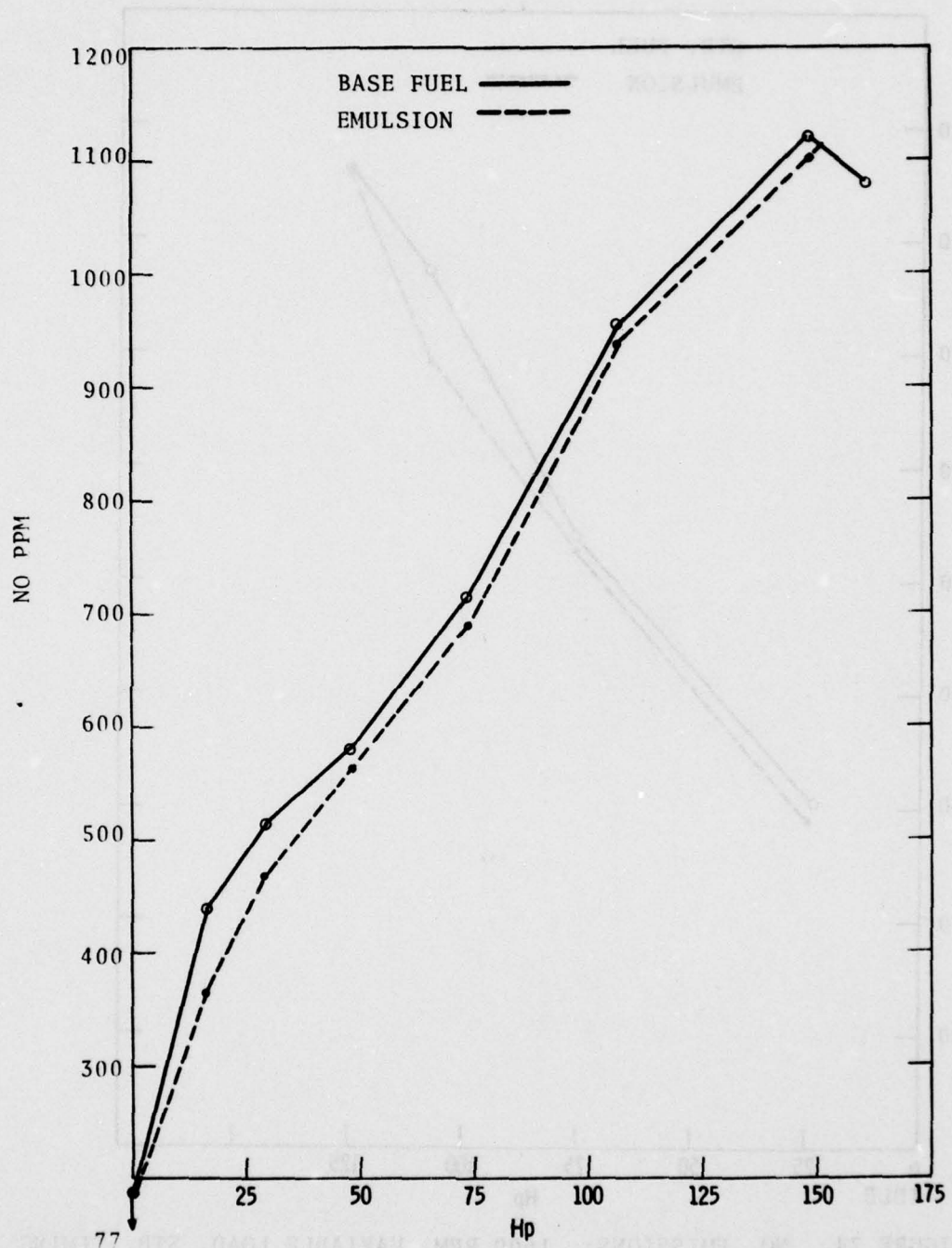
FIGURE 23. NO x EMISSIONS: PROP LOAD, 3.6° ADVANCE
