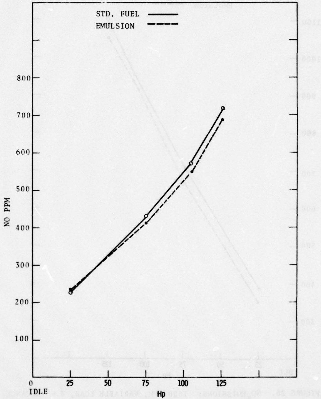
FIGURE 25. NO x EMISSIONS: 1600 RPM, VARIABLE LOAD, 3.6° RETARD
