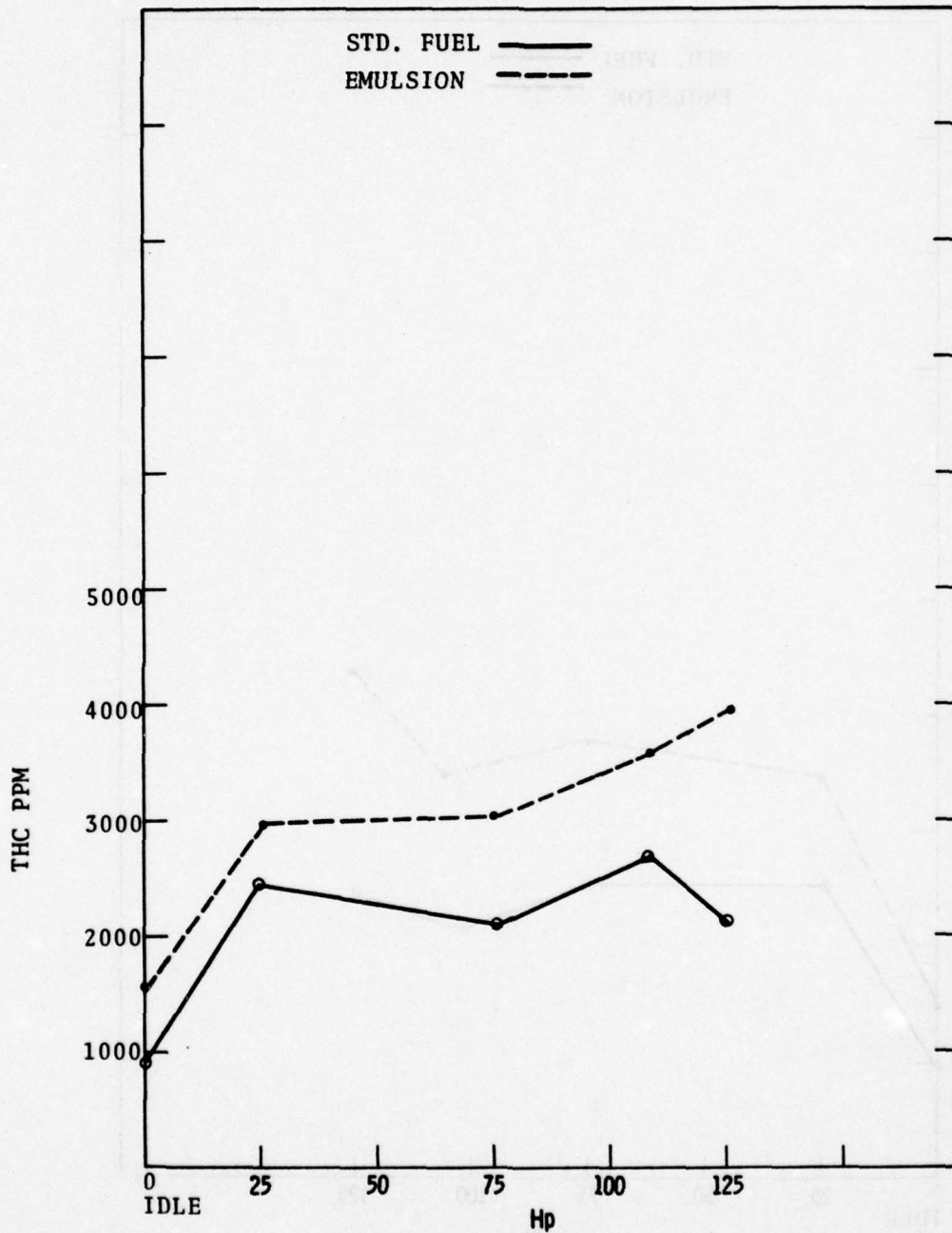
FIGURE 32. THC EMISSIONS: 1600 RPM, VARIABLE LOAD, 3.6° RETARD
