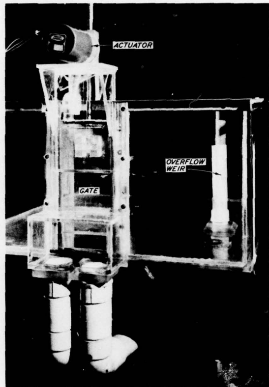
Figure 5. Head tank
