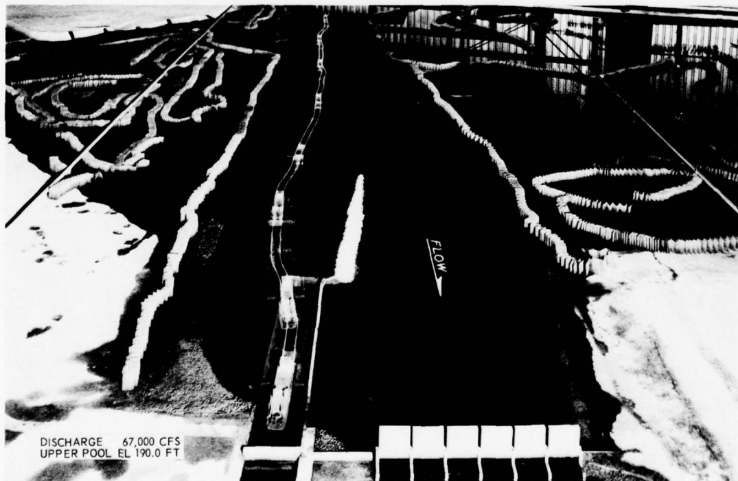
Photo 4. Plan C, path of upbound tow leaving upper guard wall and proceeding upstream along the right bank
