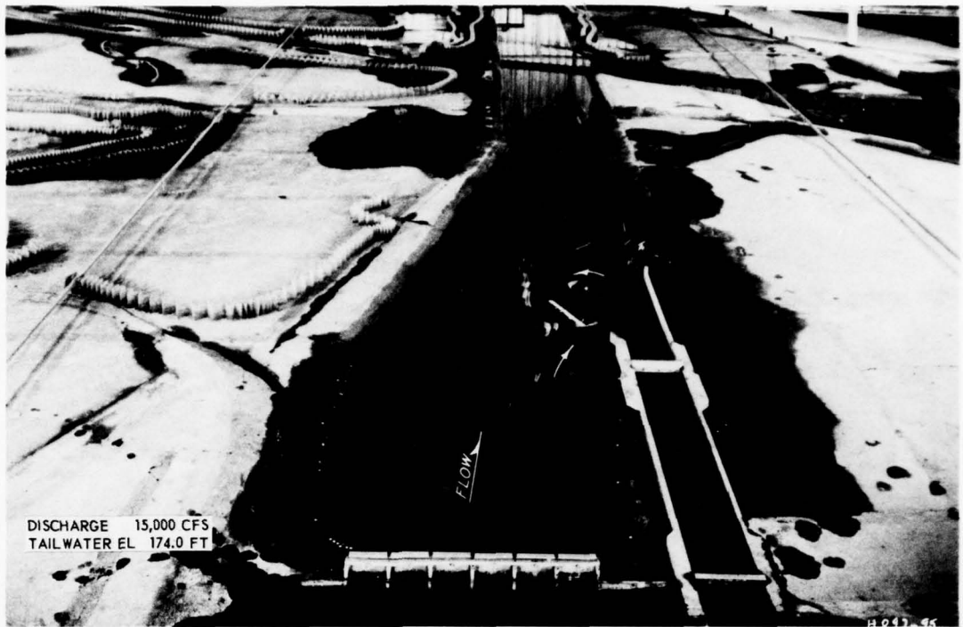
Photo 1. Plan C, surface currents downstream of gated spillway and in lower lock approach. Note effect of wing dike to left of approach
