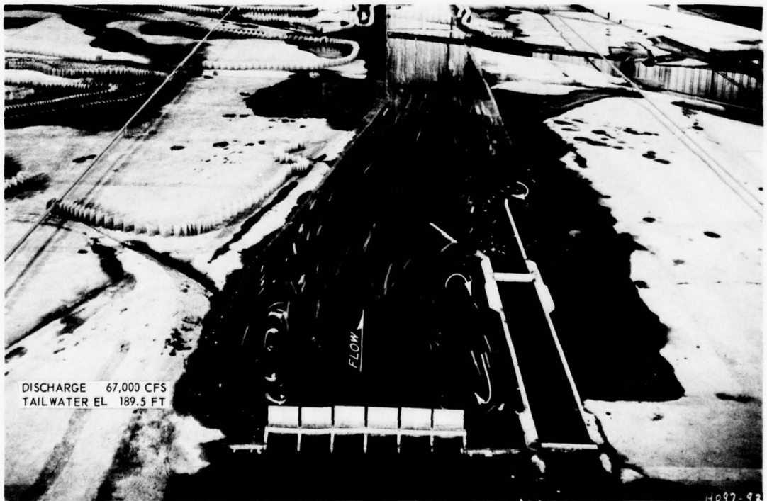
Photo 2. Plan C, surface currents through gated spillway and in lower lock approach with wing dike in place
