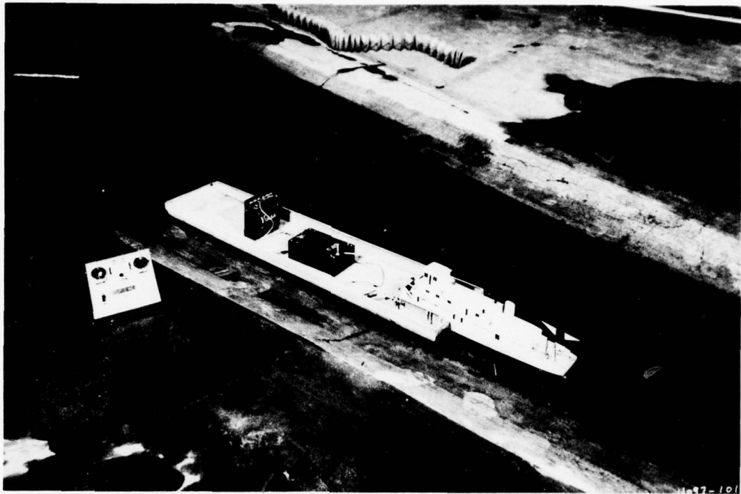
Figure 3. Model towboat and tow with remote-controls existing prototype conditions. This type of adjustment was not considered necessary since the proposed improvements would involve considerable change from existing conditions. The model was constructed with a brushed cement-mortar finish to provide a roughness factor (Manning's n ) of about 0.0135, which corresponds to a prototype channel roughness of about 0.030. Based on experience with other models of this type, brushed concrete gives a very close approximation of the roughness required to reproduce prototype conditions.
