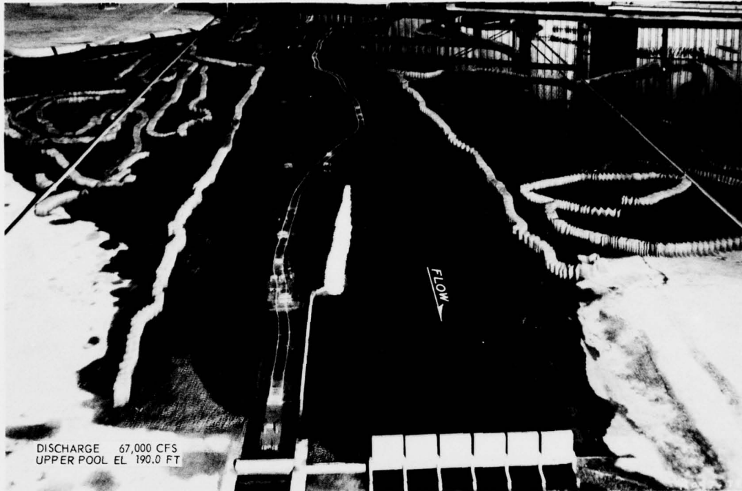
Photo 5. Plan C, path of upbound tow leaving upper lock approach and bypassing tow along the right bank
