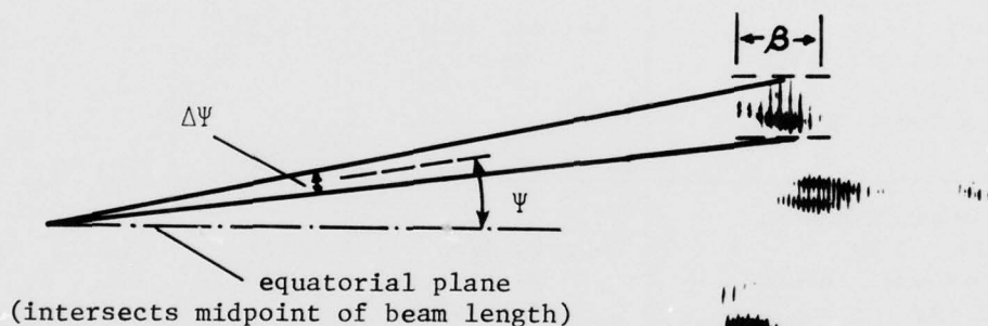
FIGURE 3C Enlargement of Typical Grain Reflections From a Deformed Aluminum Alloy Specimen
