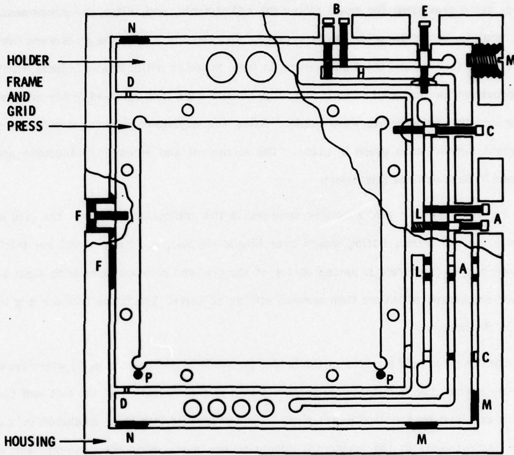
Fig. 3. Grid Assembly Positioned in the Collimator Housing with Cut-Aways of Mounting and Positioning Mechanisms
