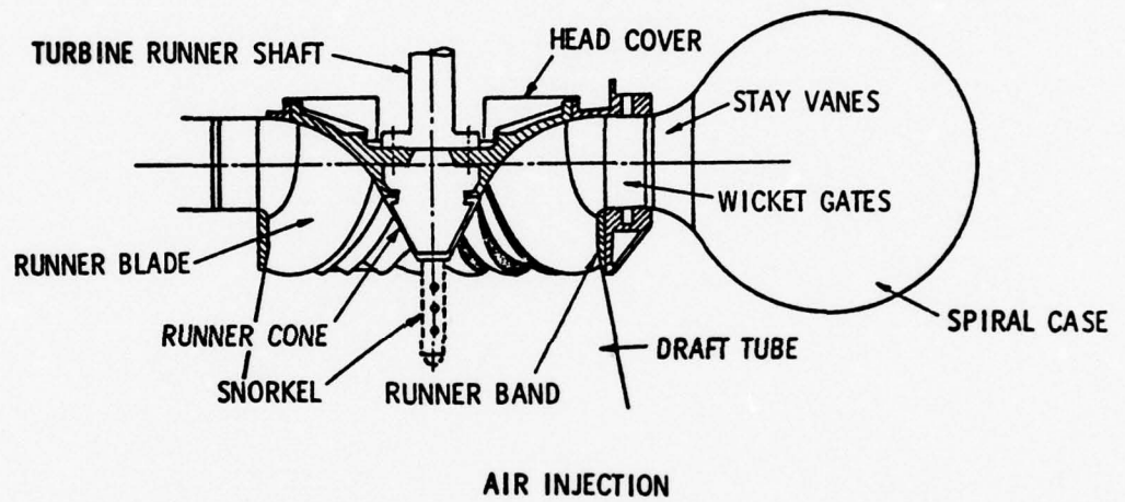
Figure 2. Arrangement used for air admission to the draft tube in an effort to reduce draft tube surge.
