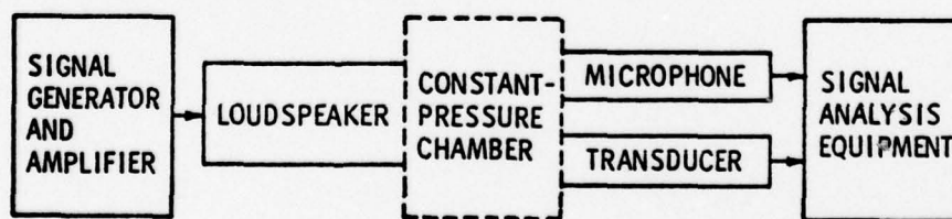
Figure 26. Schematic diagram of constant pressure calibration chamber showing location of microphone, pressure tapping, and loudspeaker.
