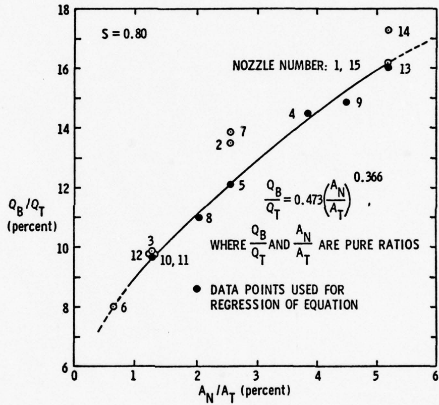
Figure 21. Injection flow required to eliminate surge for all nozzles tested using the cylindrical draft tube, S = 0.80 .
