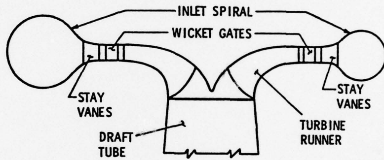
Figure 1. Schematic of a turbine cross section illustrating the geometry of the flow passage in the region of the wicket gates.
