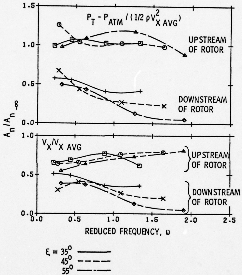
Figure 44. Amplitude ratio versus reduced frequency for a constant 0^\circ mean incidence angle.
