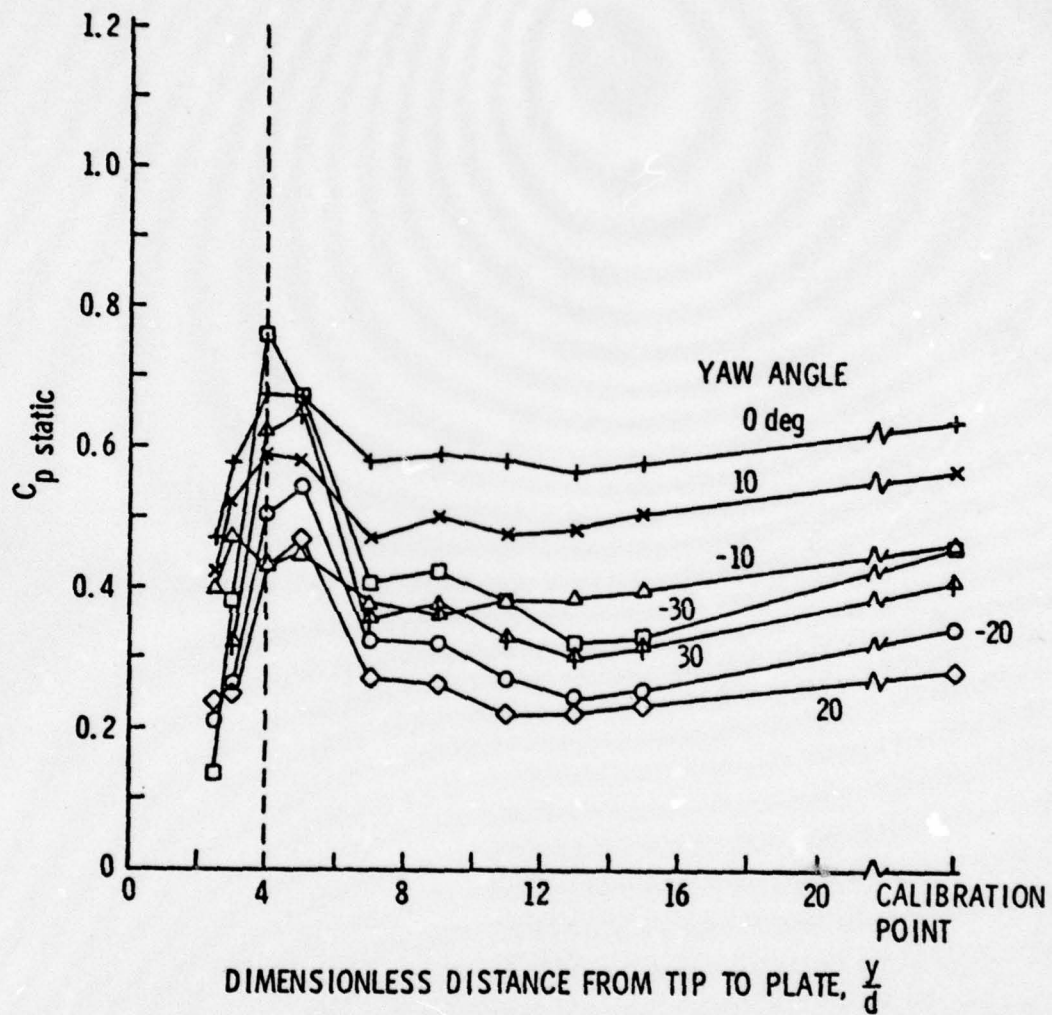
Figure A.17. C_p static versus the dimensionless distance from the probe tip to the plate for Probe 1. The probe is drawn through a hole in the plate.
