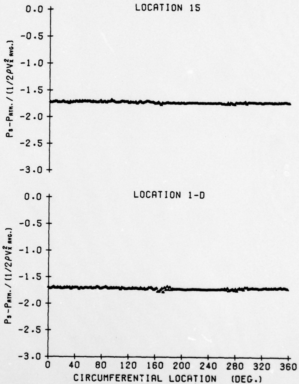
Figure C.5. Static pressure distribution for the 90° square distortion without the rotor installed.
