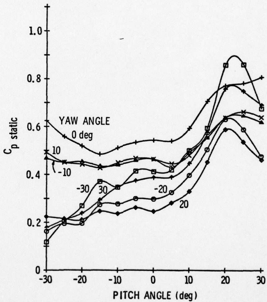
Figure A.7. Calibration data for Probe 2, C_p static versus pitch angle.
