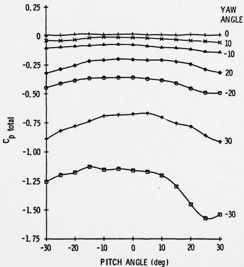
Figure 10. Calibration data for Probe 1, C_p total versus pitch angle.
