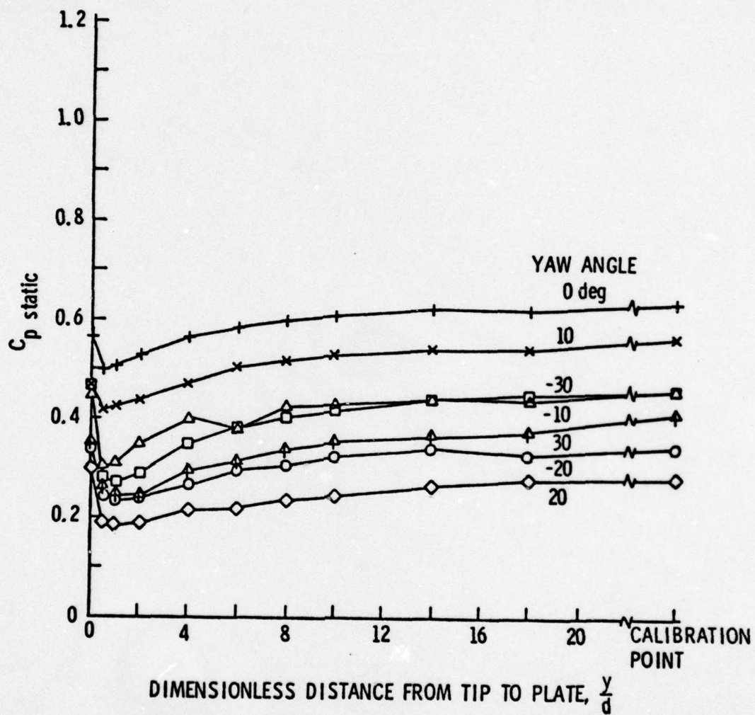
Figure A.15. C_p static versus the dimensionless distance from the probe tip to the plate for Probe 1. The probe is approaching the plate.
