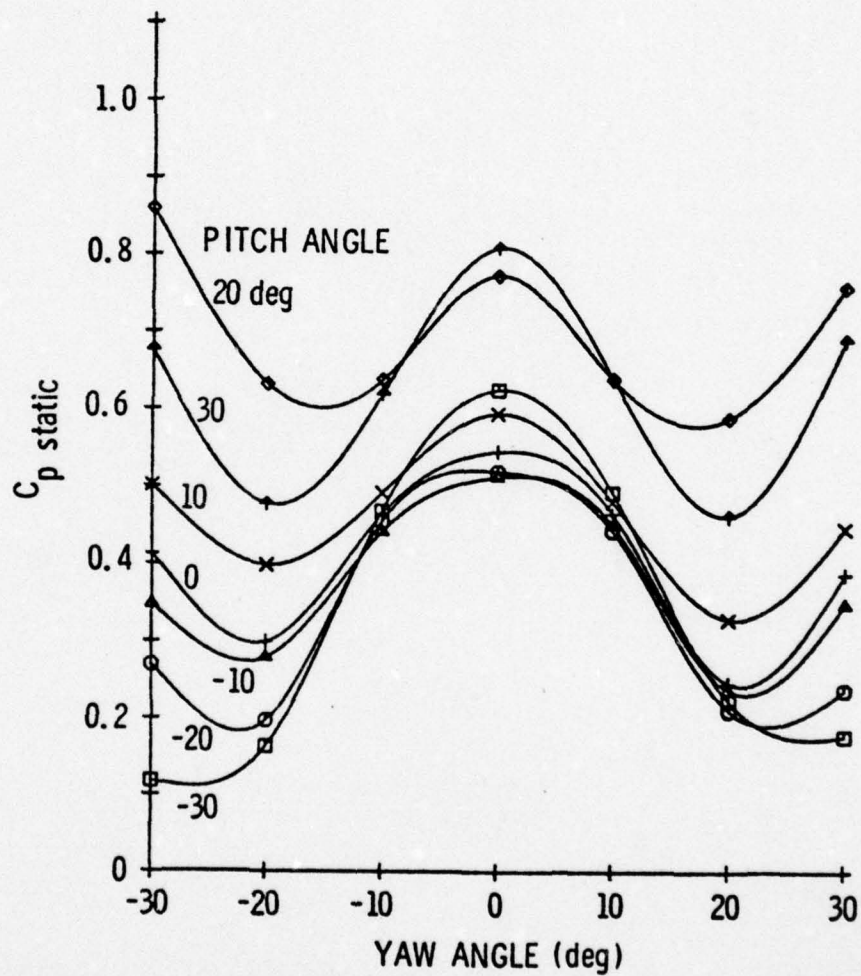
Figure A.8. Calibration data for Probe 2, C_{p \text{ static}} versus yaw angle.
