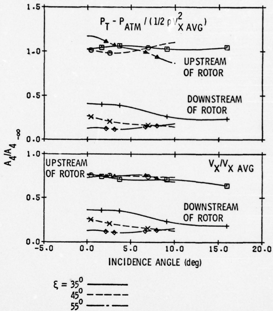
Figure 42. Measured axial velocity and total pressure distortion versus incidence angle for a four-cycle sinusoidal distortion.
