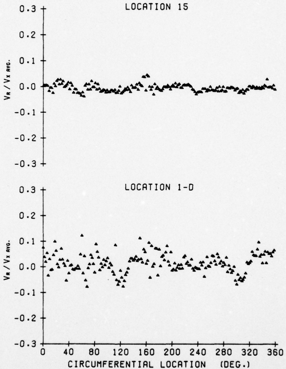
Figure 36. Sample V_R distribution for a sinusoidal distortion.
