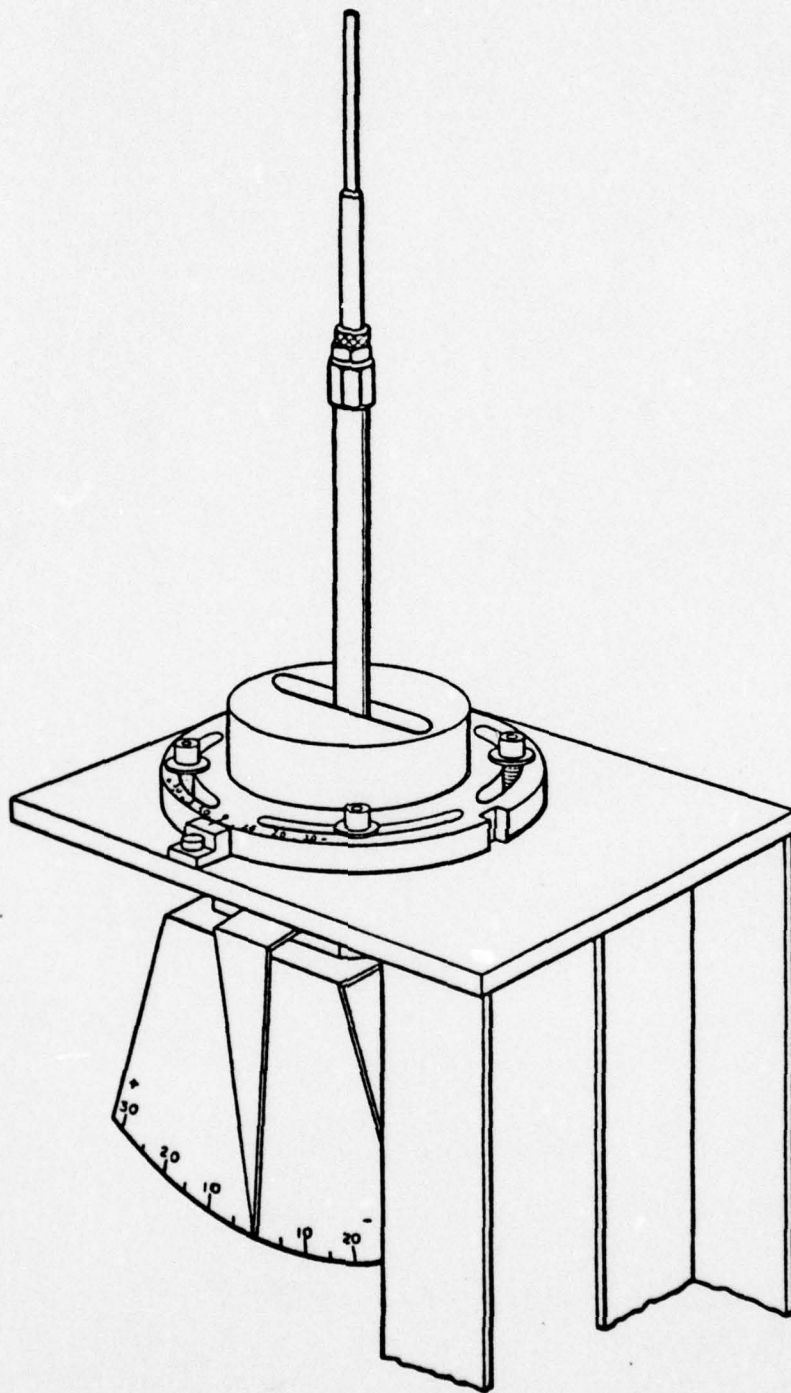
Figure A.3. A sketch of the probe calibration positioning device.
