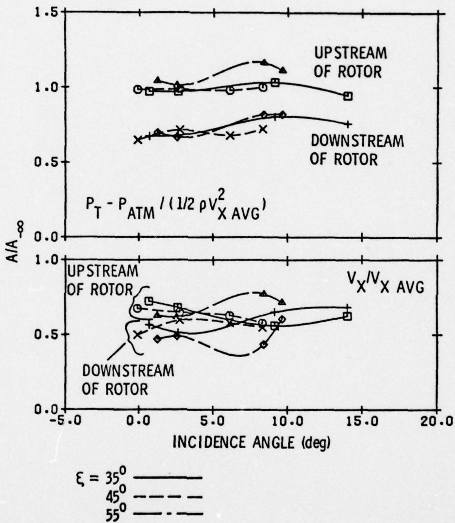
Figure 47. Amplitude ratio versus incidence for a 180° square distortion.
