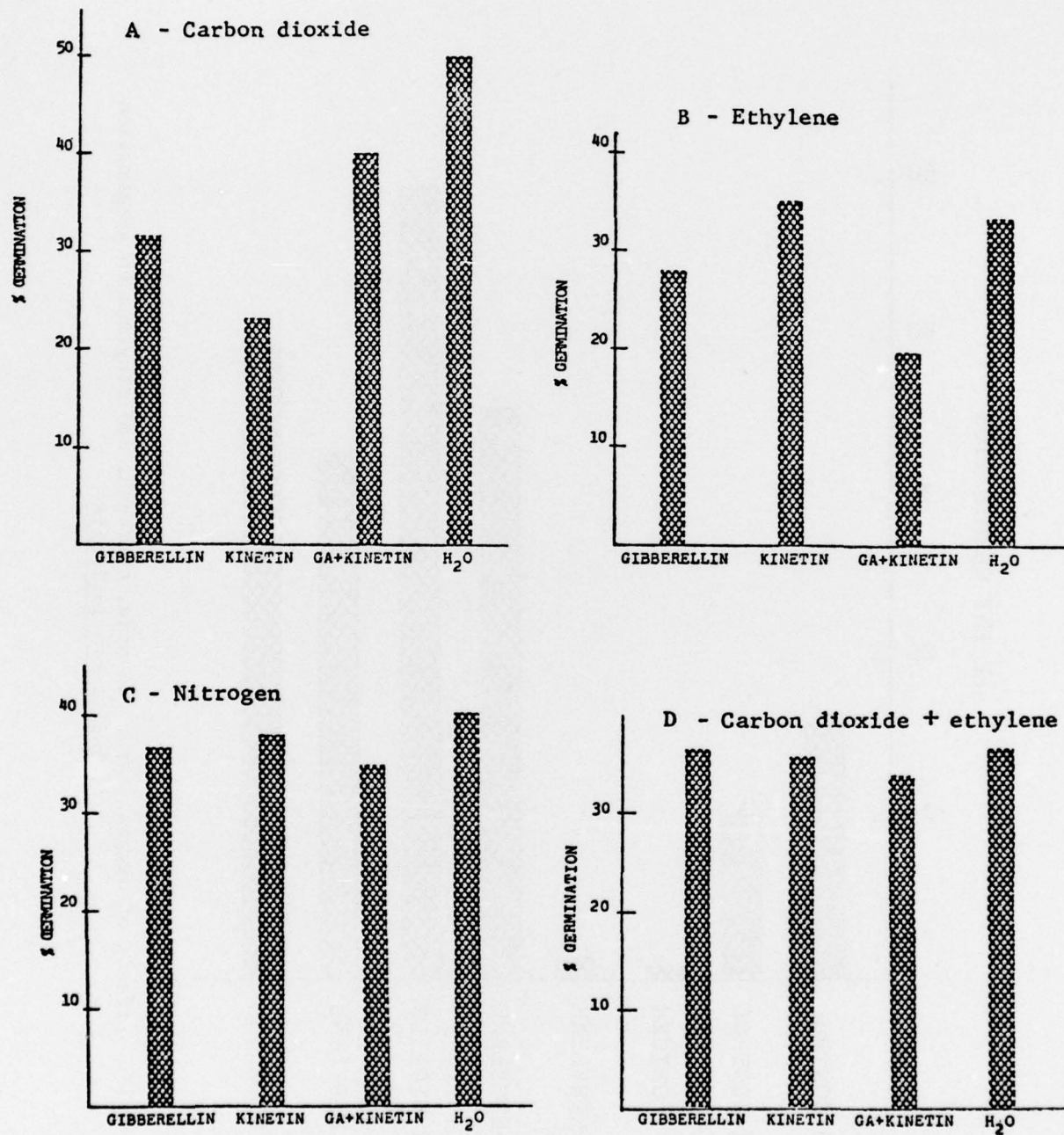
Figure 16. Interaction of gases with gibberellin and kinetin on germination of Sagittaria latifolia
