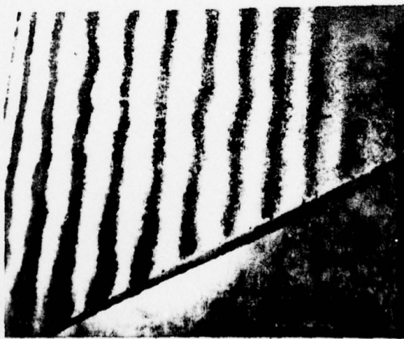
Fig. 8. Bright-field image after 3 min at 300°C. Zone axis [211]. Mag. 15,000. Grain boundary precipitates and G.P. zones in matrix (50-70 A).
