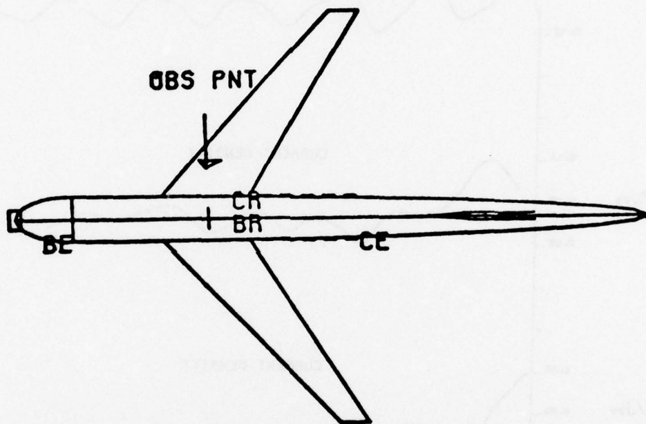
Figure 66. Computer model of a KC-135 aircraft.
