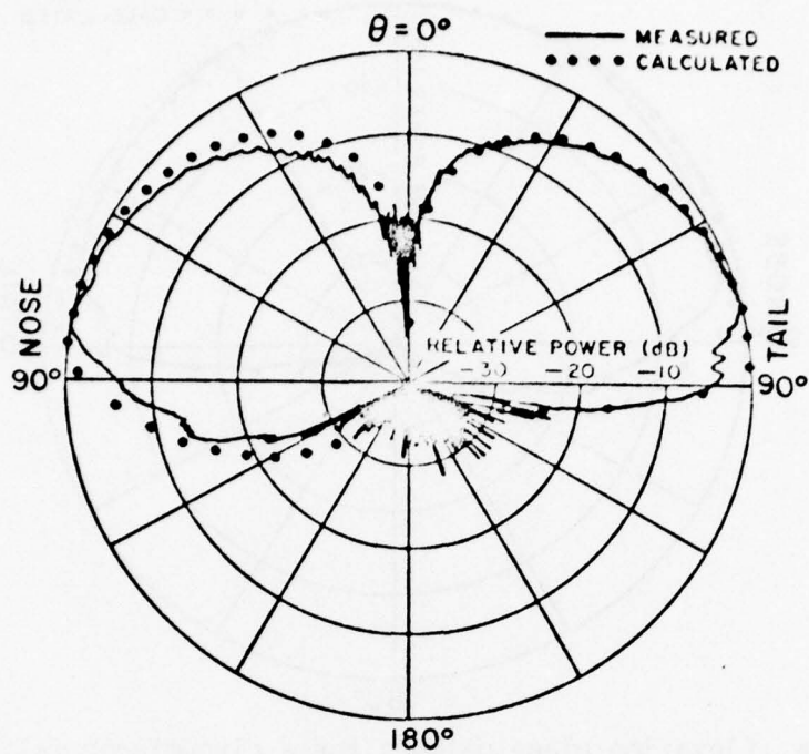
Figure 14a. Elevation plane pattern for a \lambda/4 monopole mounted forward of the wings on a KC-135 aircraft. (No radome and vertical stabilizer included).
