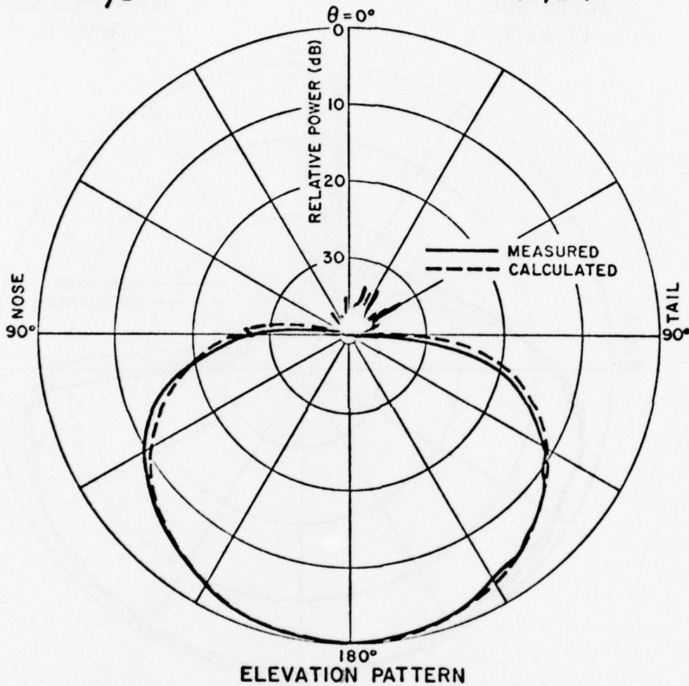
Figure 23. Elevation pattern of axial slot on a 1/35th scale model of space shuttle (with radome included).
