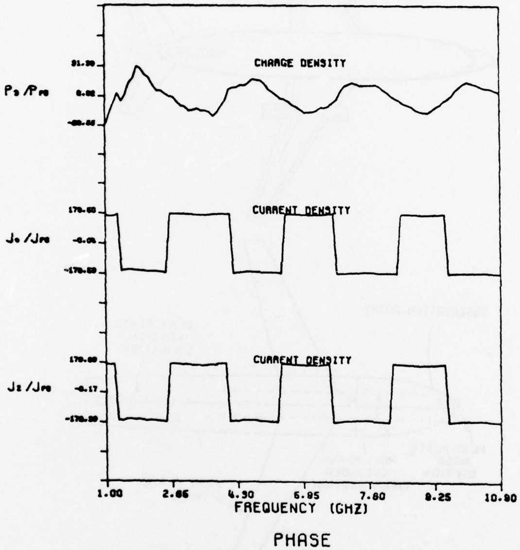
PHI MODE Figure 70. The surface current and charge densities induced on a KC-135 aircraft.
