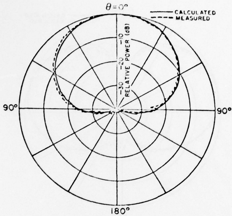
Figure 28a. Roll plane pattern ( E_{\theta} ) for a KA-band circumferential waveguide forward of the wings.
