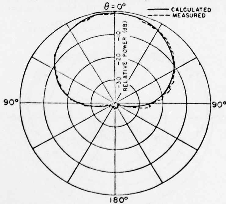
Figure 28b. Roll plane pattern ( E_{\theta} ) for a KA-band circumferential waveguide above the wings.
