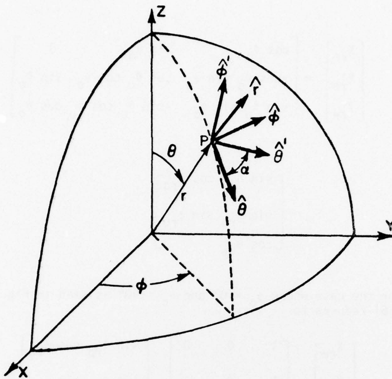
Figure 36. Illustration of the spherical coordinate system.
