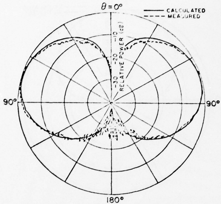
Figure 27a. Roll plane pattern ( E_\theta ) for a 1/25 scale model of a KC-135 with a \lambda/4 monopole on the fuselage forward of the wings at freq. = 34.92 GHz (model frequency).
