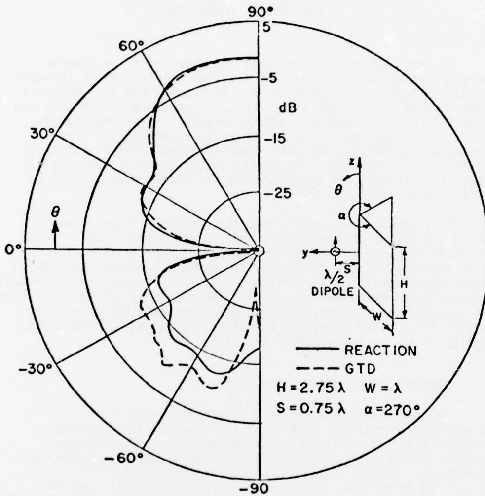
Figure 11b. E-plane pattern.
