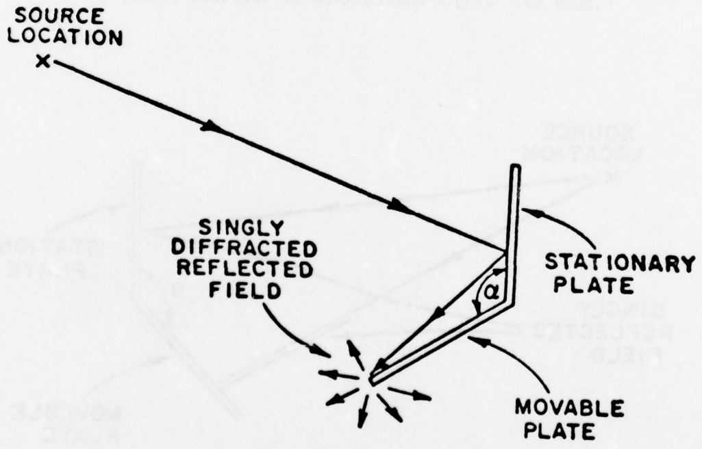
Figure 8d. Single diffraction of reflected field.
