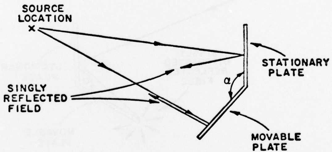
Figure 8b. Single reflection of incident field.
