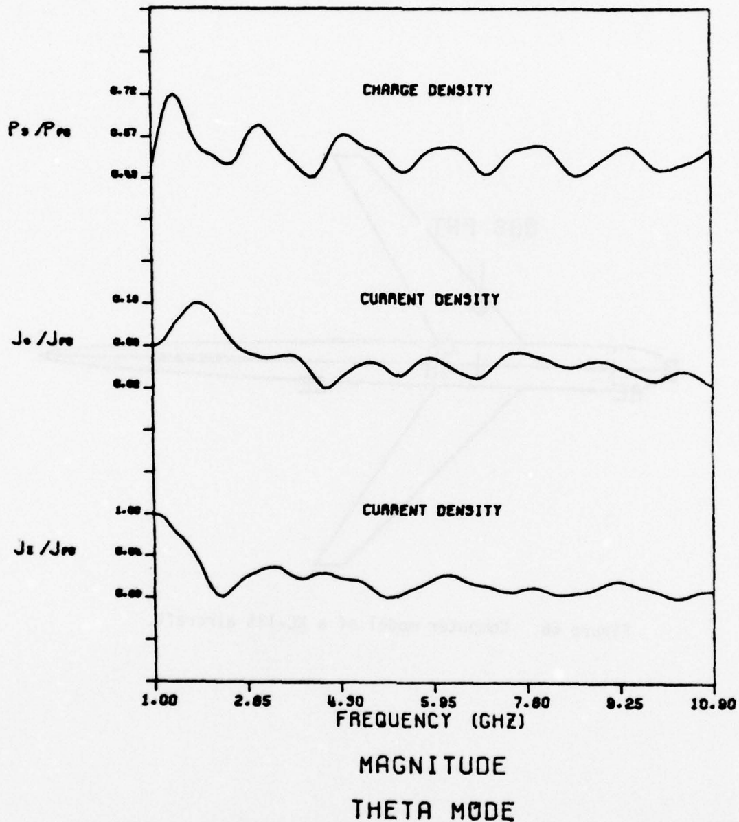
Figure 67. The surface current and charge densities induced on a KC-135 aircraft.
