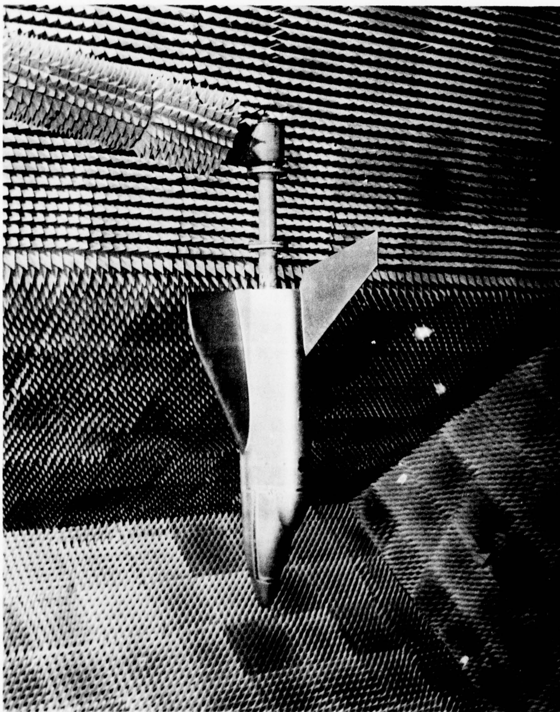
Figure 20a. Scale model (1/35) of Space Shuttle in Anechoic Chamber at NASA, (Hampton, Va.).
