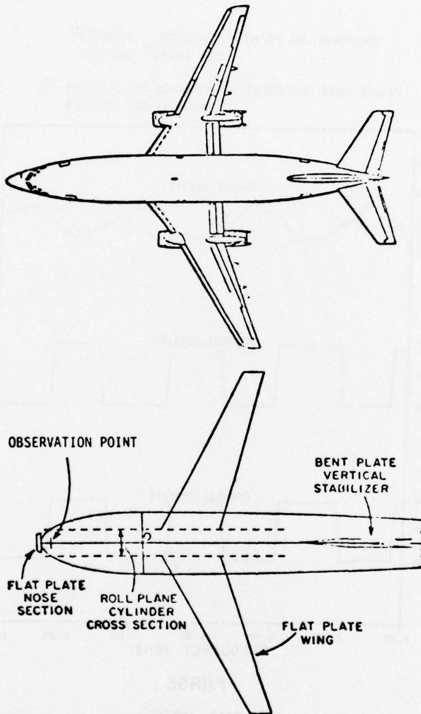
Figure 71. Computer simulated model for a Boeing 737 aircraft (top view). The observation point is located at station 220 on the top of the fuselage.
