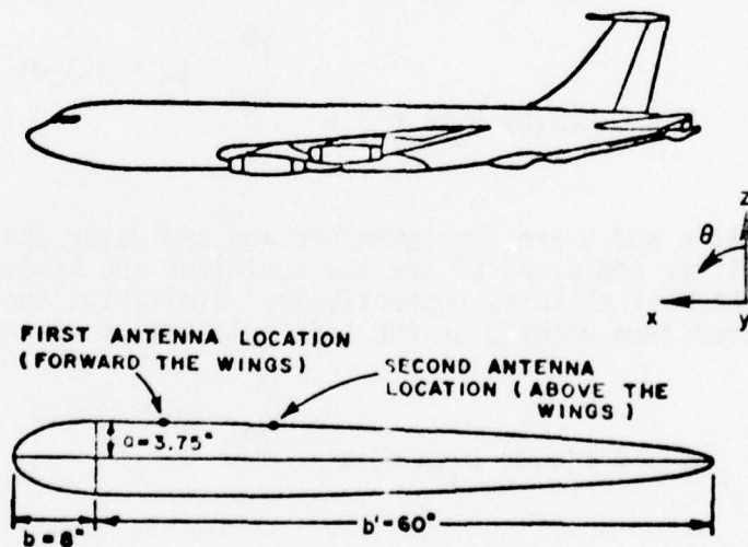
Figure 12. Theoretical model of KC-135 aircraft.
