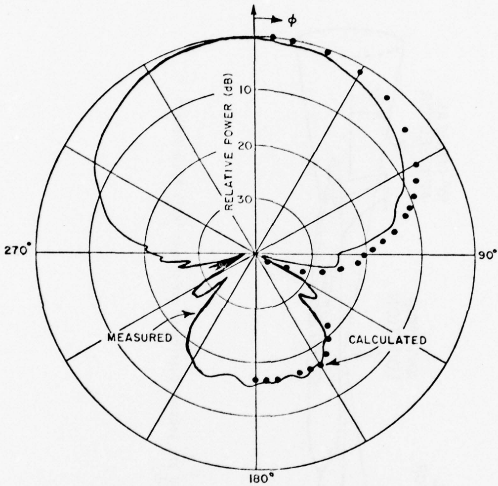
Figure 31b. Elevation plane pattern of an axial slot mounted on a 4\lambda \times 2\lambda prolate spheroid with the three-dimensional theoretical solution presented.
