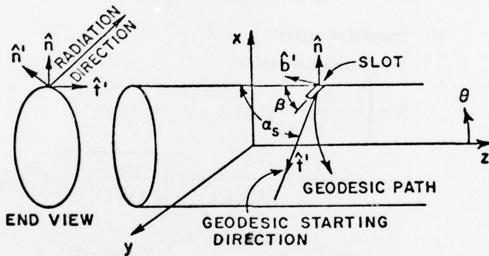
(b) GEOMETRY OF SLOT PROBLEM
