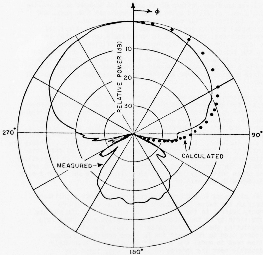
Figure 3la. Elevation plane pattern of an axial slot mounted on a 4\lambda \times 2\lambda prolate spheroid with the two-dimensional theoretical solution presented.
