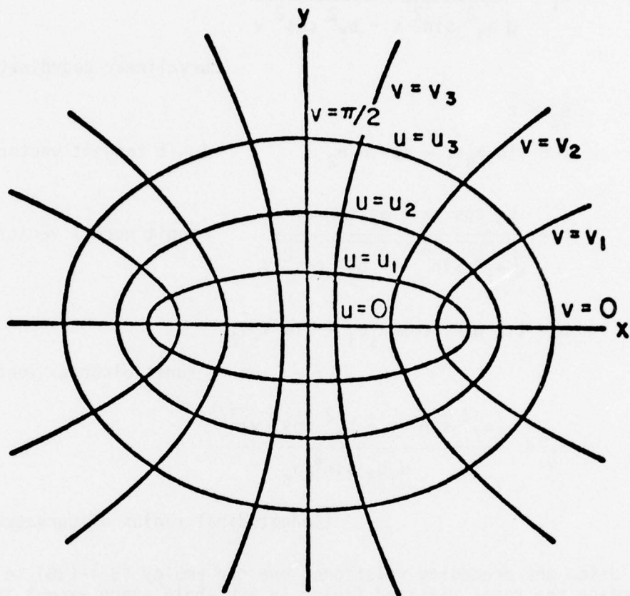
Figure 6. Diagram showing the elliptic cylinder coordinate system.
