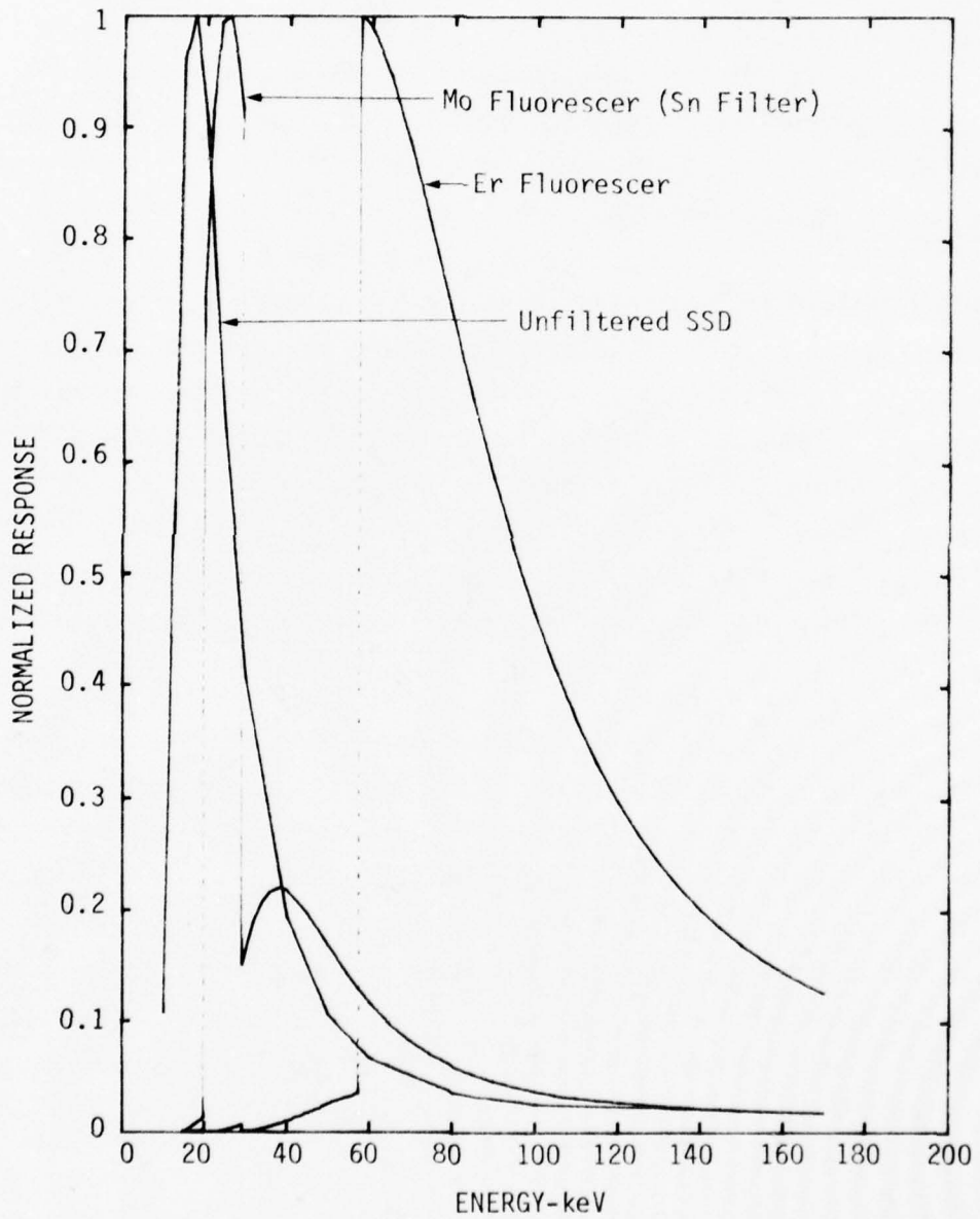
Figure 2.6. Response functions for typical x-ray transmission channels.
